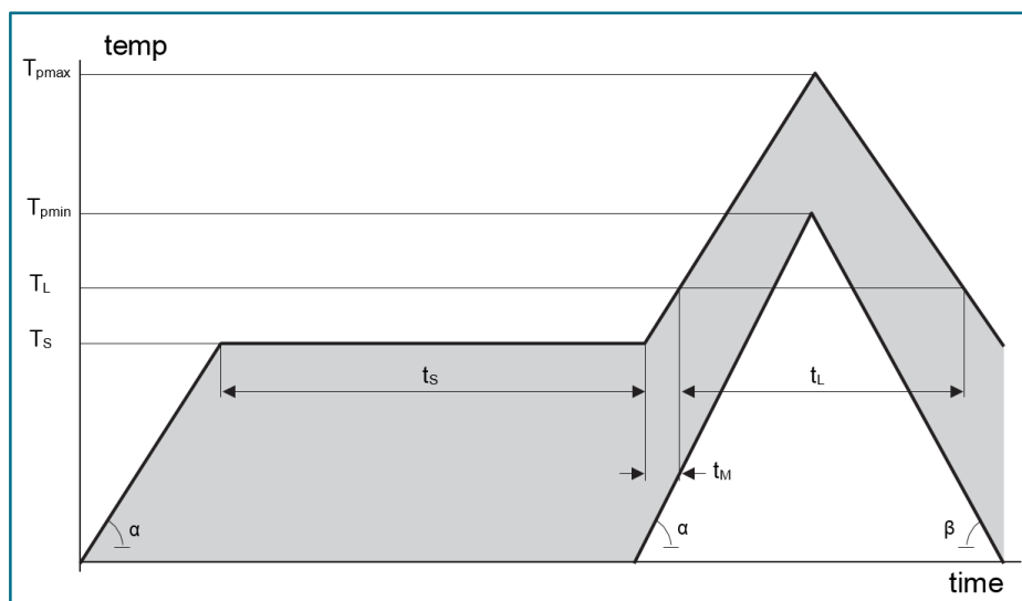
Figure 14 Reflow profile
