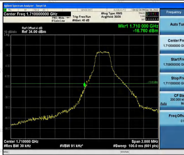
Band4-1.4MHz-QPSK-19957-1RB#5
