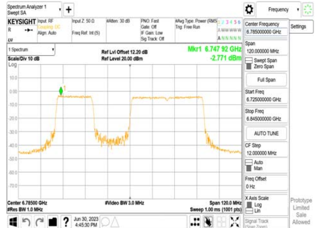
802.11be_80MHz_Chain0_6785MHz_SU_Punc20_Mid2
