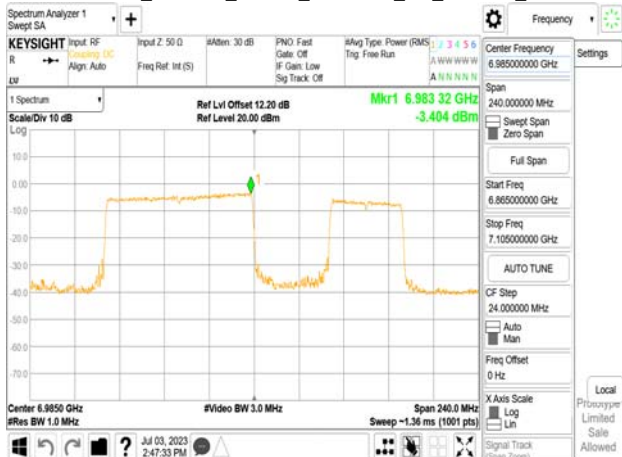
802.11be_160MHz_Chain0_6985MHz_SU_Punct40_Mid2
