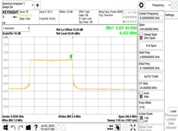
802.11be_160MHz_Chain1_6025MHz_SU_Punct20_Mid3
