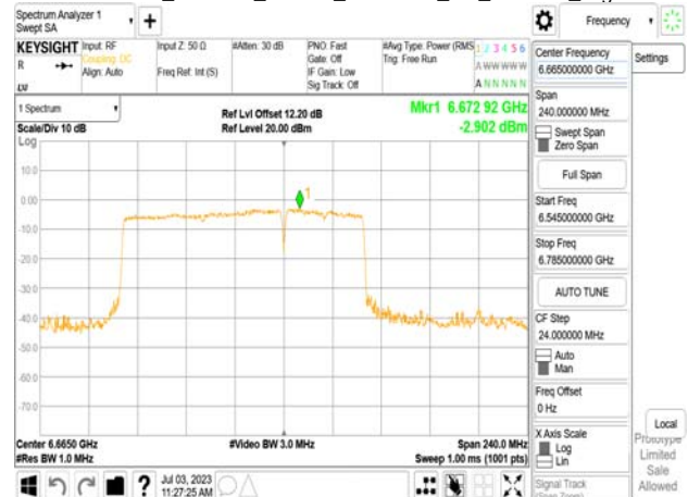
802.11be_160MHz_Chain1_6665MHz_SU_Punct40_High
