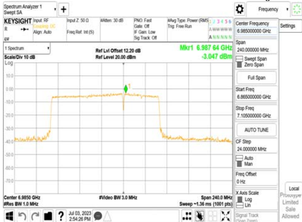
802.11be_160MHz_Chain0_6985MHz_SU_Punct40_Mid2
