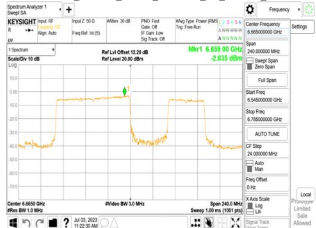
802.11be_160MHz_Chain0_6665MHz_SU_Punct40_Mid2
