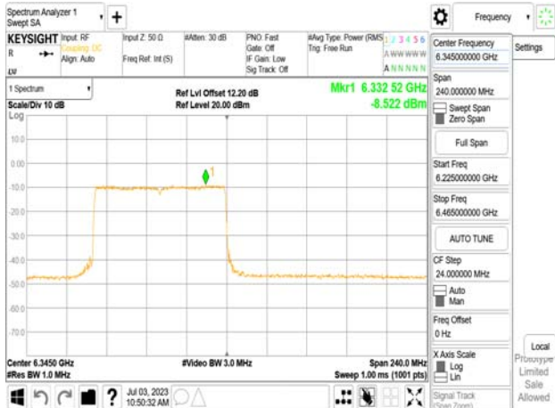
802.11be_160MHz_Chain1_6345MHz_SU_Punct20_High
