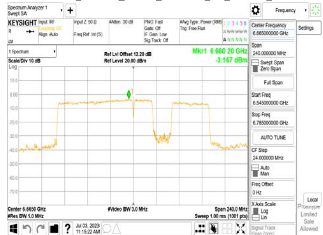
802.11be_160MHz_Chain0_6665MHz_SU_Punct40_High
