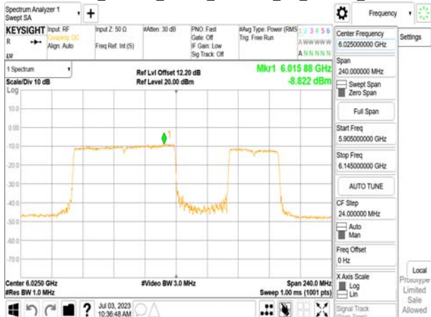
802.11be_160MHz_Chain1_6025MHz_SU_Punct40_Mid2
