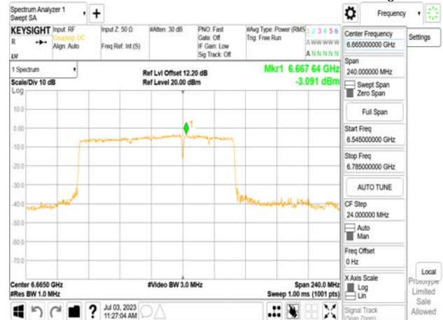
802.11be_160MHz_Chain0_6665MHz_SU_Punct40_Mid2
