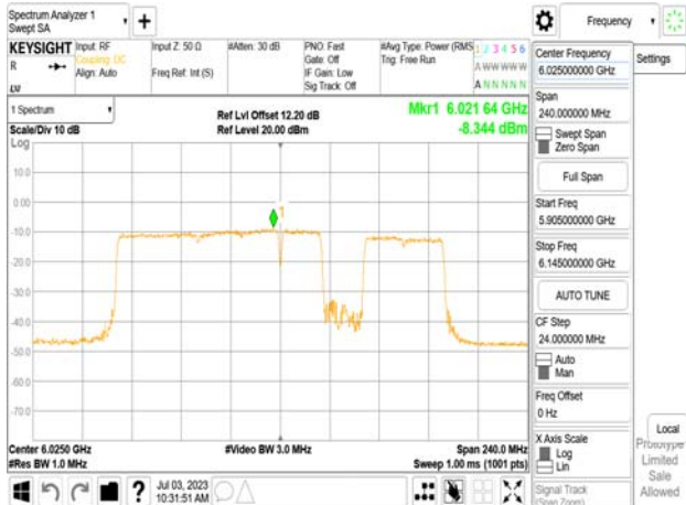
802.11be_160MHz_Chain1_6025MHz_SU_Punct40_Mid2
