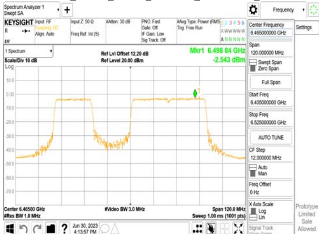
802.11be_80MHz_Chain0_6465MHz_RU484+242_Punc20
