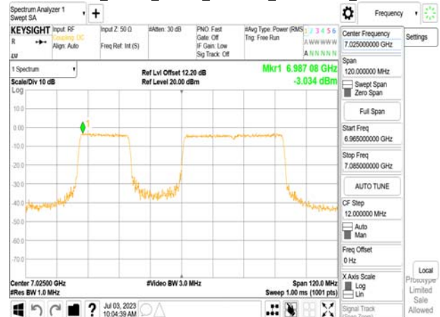
802.11be_80MHz_Chain0_7025MHz_RU484+242_Punc20
