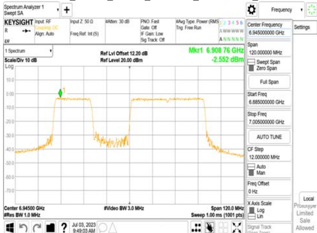
802.11be_80MHz_Chain0_6945MHz_RU484+242_Punc20
