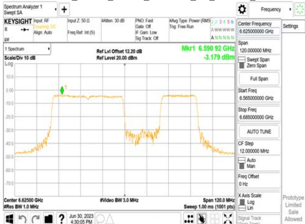
802.11be_80MHz_Chain1_6625MHz_SU_Punc20_Mid2
