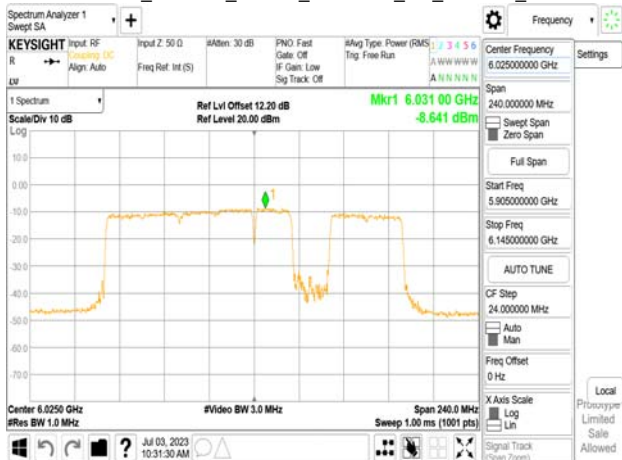
802.11be_160MHz_Chain0_6025MHz_SU_Punct40_Mid2
