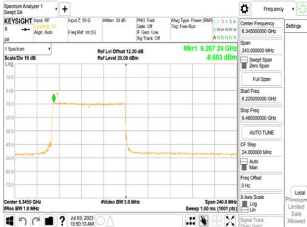
802.11be_160MHz_Chain0_6345MHz_SU_Punct20_High
