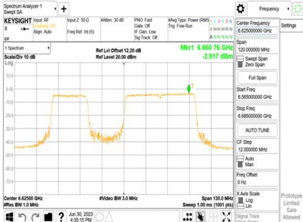
802.11be_80MHz_Chain0_6625MHz_SU_Punc20_Mid2
