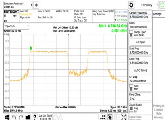
802.11be_80MHz_Chain0_6785MHz_SU_Punc20_Mid2
