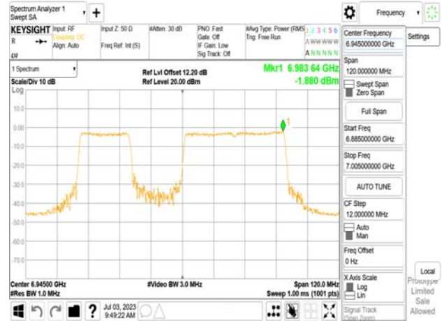
802.11be_80MHz_Chain1_6945MHz_SU_Punct20_Mid2
