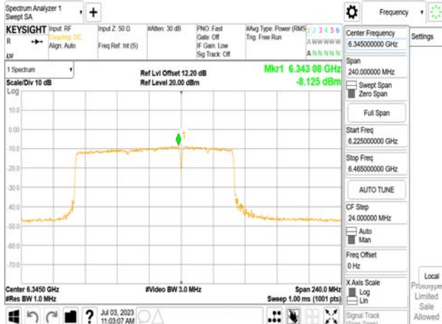
802.11be_160MHz_Chain0_6345MHz_SU_Punct40_High
