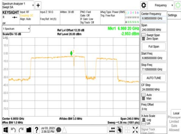
802.11be_160MHz_Chain0_6985MHz_SU_Punct40_High
