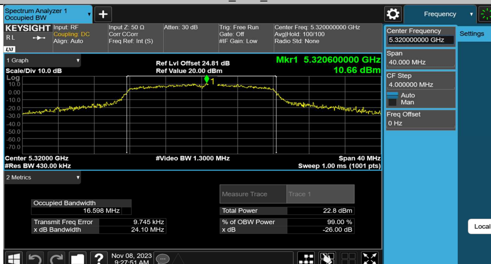
11A Ant2 5320
