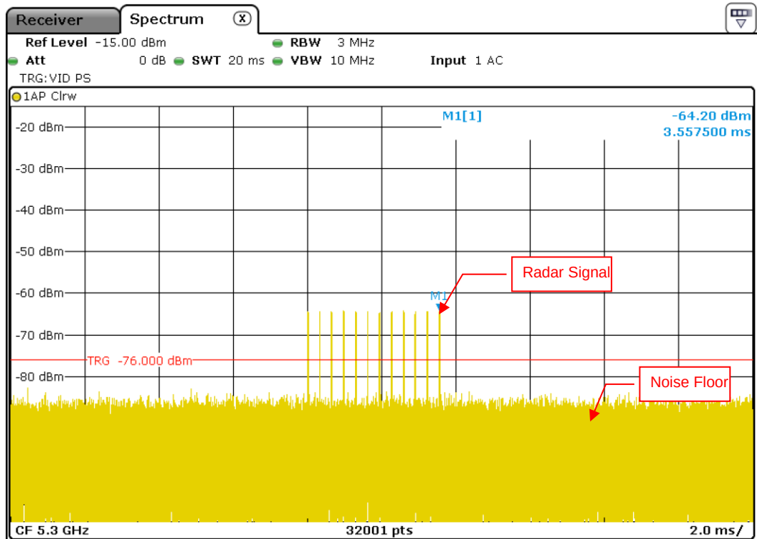
Radar Signal 4
