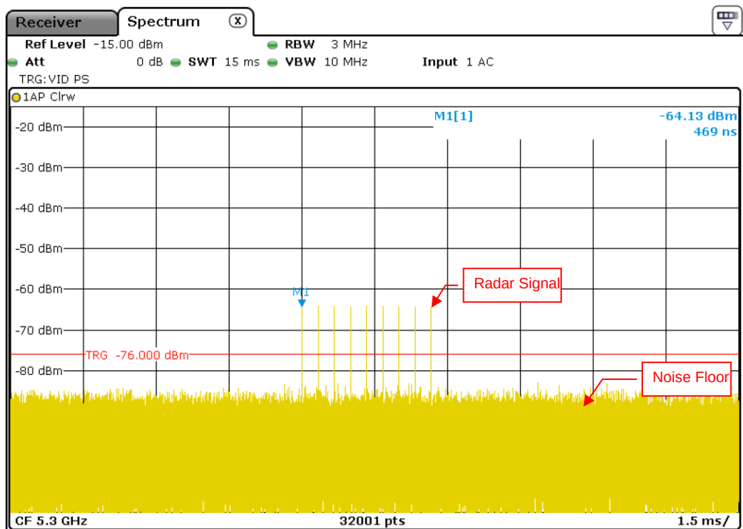
Radar Signal 6
