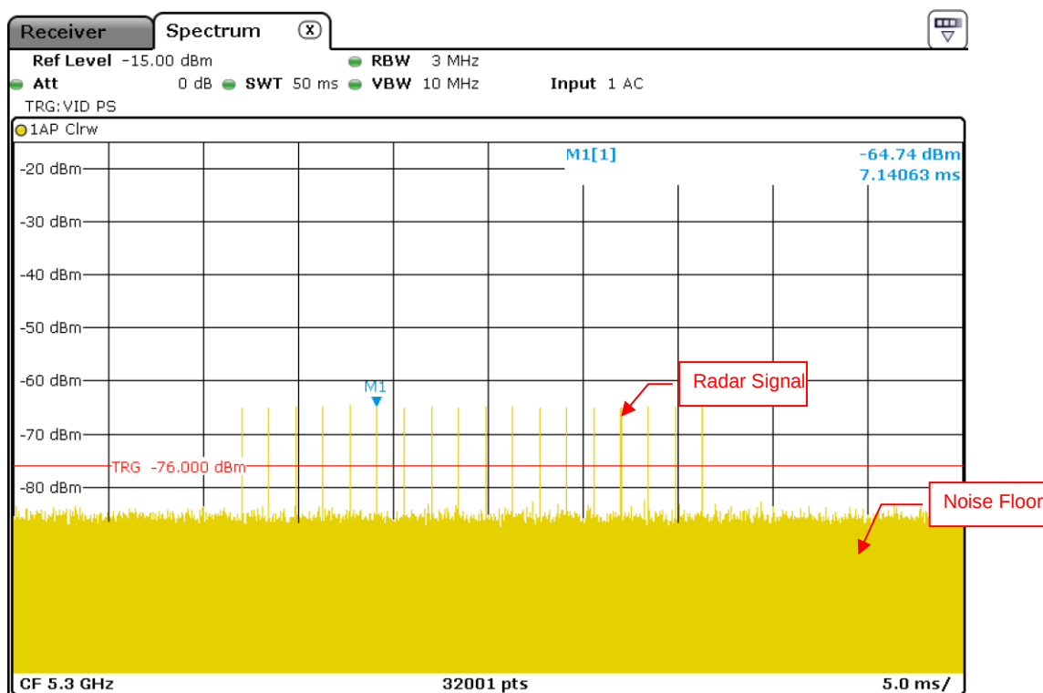
Radar Signal 0
