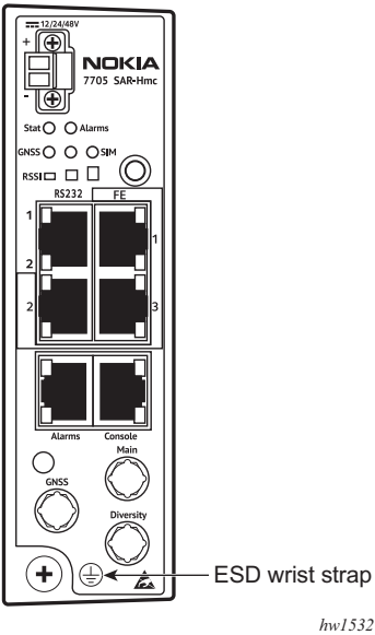
Figure 3 Wrist Strap Label at the Front of the 7705 SAR-Hmc Chassis
