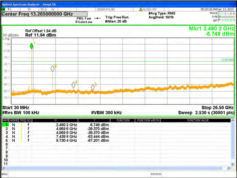
Tx. Spurious NVNT 3-DH5 2480MHz Ant1 Emission 30MHz~26.5GHz
