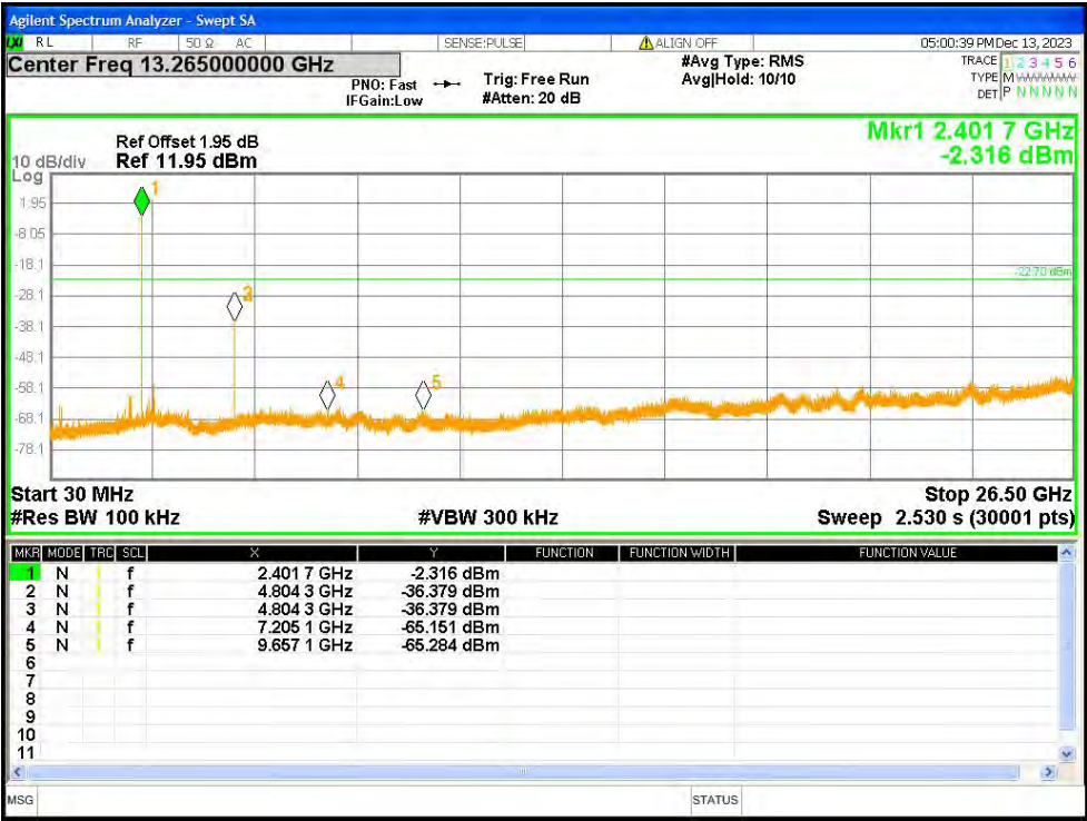
Tx. Spurious NVNT 1-DH5 2402MHz Ant1 Emission 30MHz~26.5GHz
