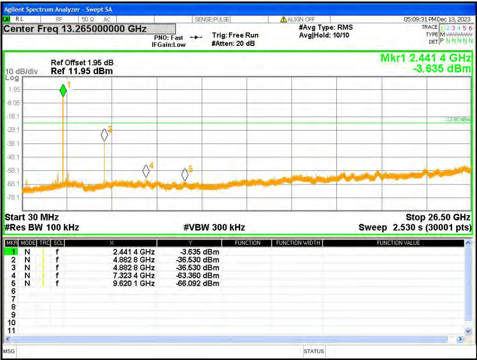
Tx. Spurious NVNT 1-DH5 2441MHz Ant1 Emission 30MHz~26.5GHz
