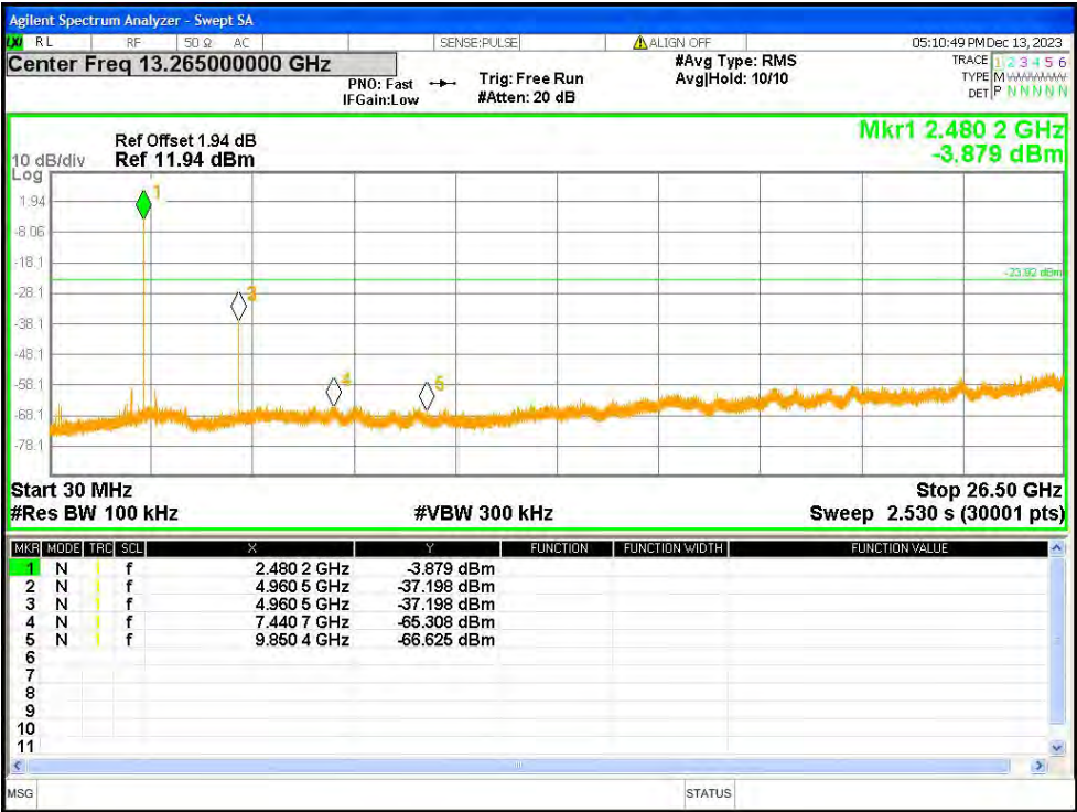
Tx. Spurious NVNT 1-DH5 2480MHz Ant1 Emission 30MHz~26.5GHz
