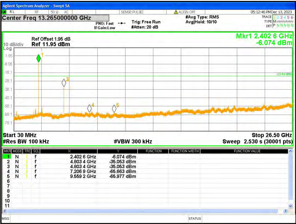
Tx. Spurious NVNT 2-DH5 2402MHz Ant1 Emission 30MHz~26.5GHz
