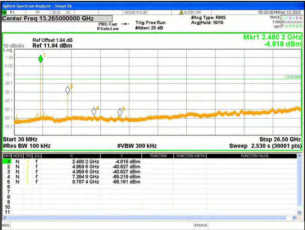
Tx. Spurious NVNT 2-DH5 2480MHz Ant1 Emission 30MHz~26.5GHz
