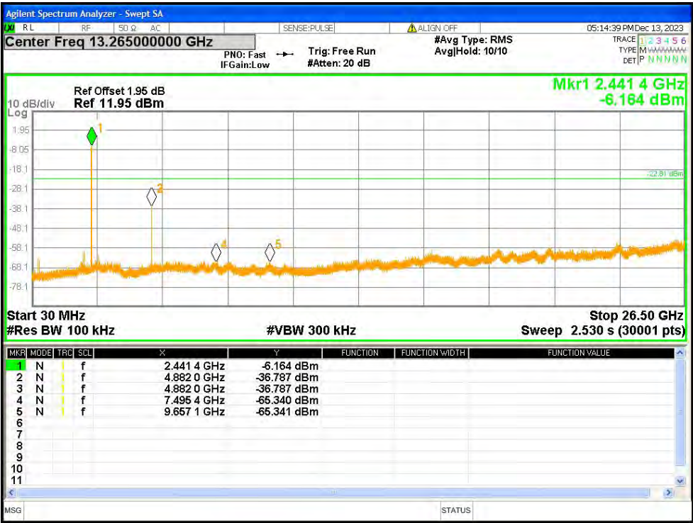
Tx. Spurious NVNT 2-DH5 2441MHz Ant1 Emission 30MHz~26.5GHz
