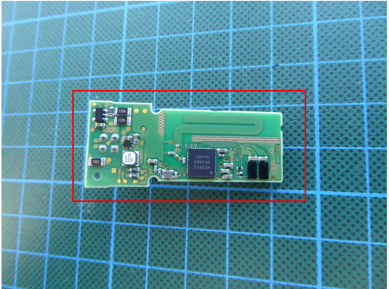
172289_E3_int_02: EUT internal – bottom view – without housing
