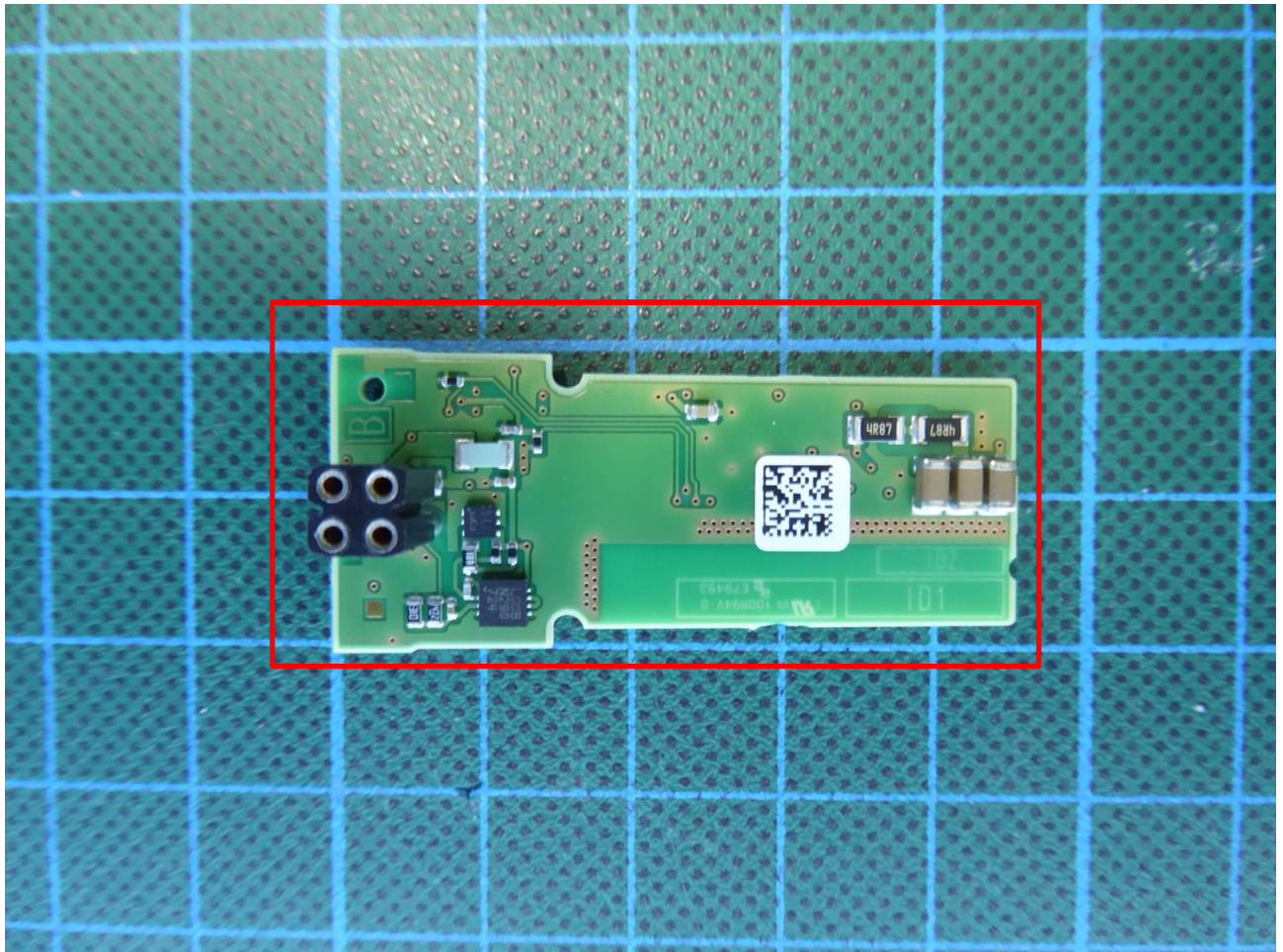
172289_E3_int_01: EUT internal – top view – without housing
