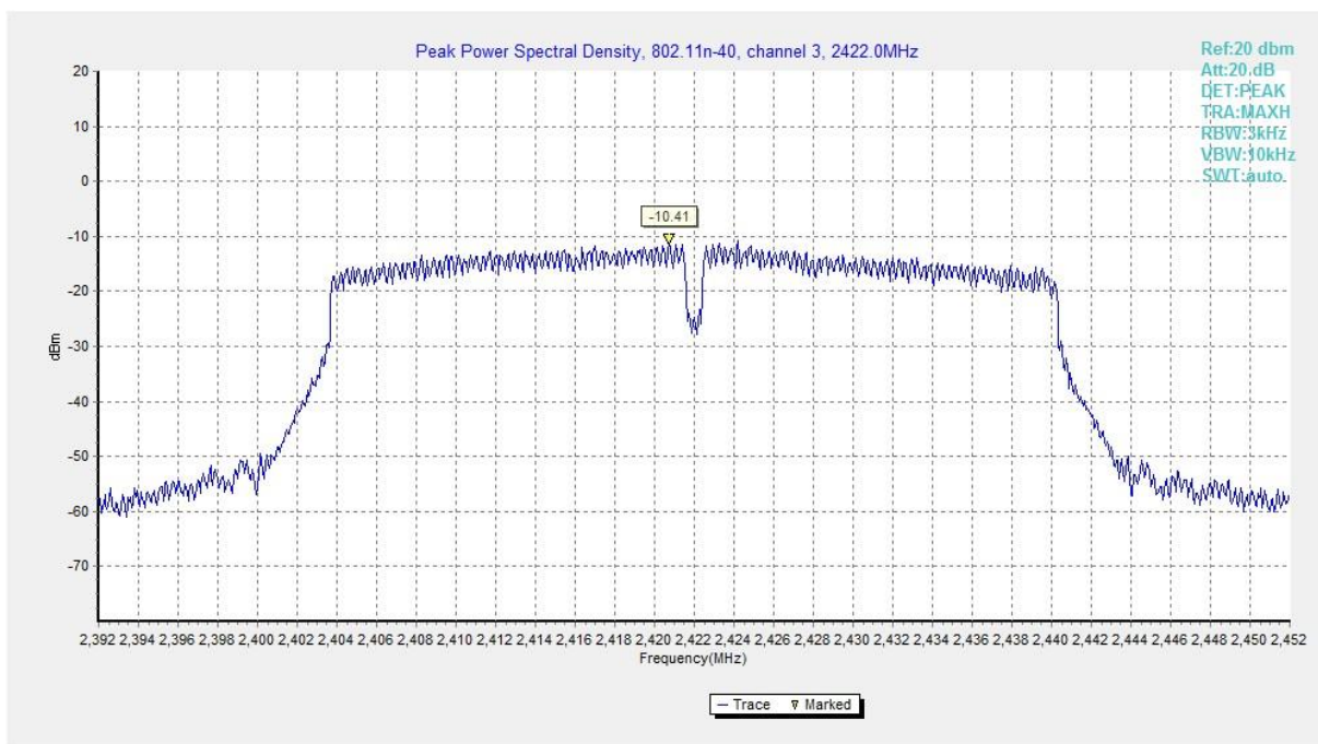
Fig.B.3.10 Power Spectral Density (802.11n-HT40, Ch 3)
