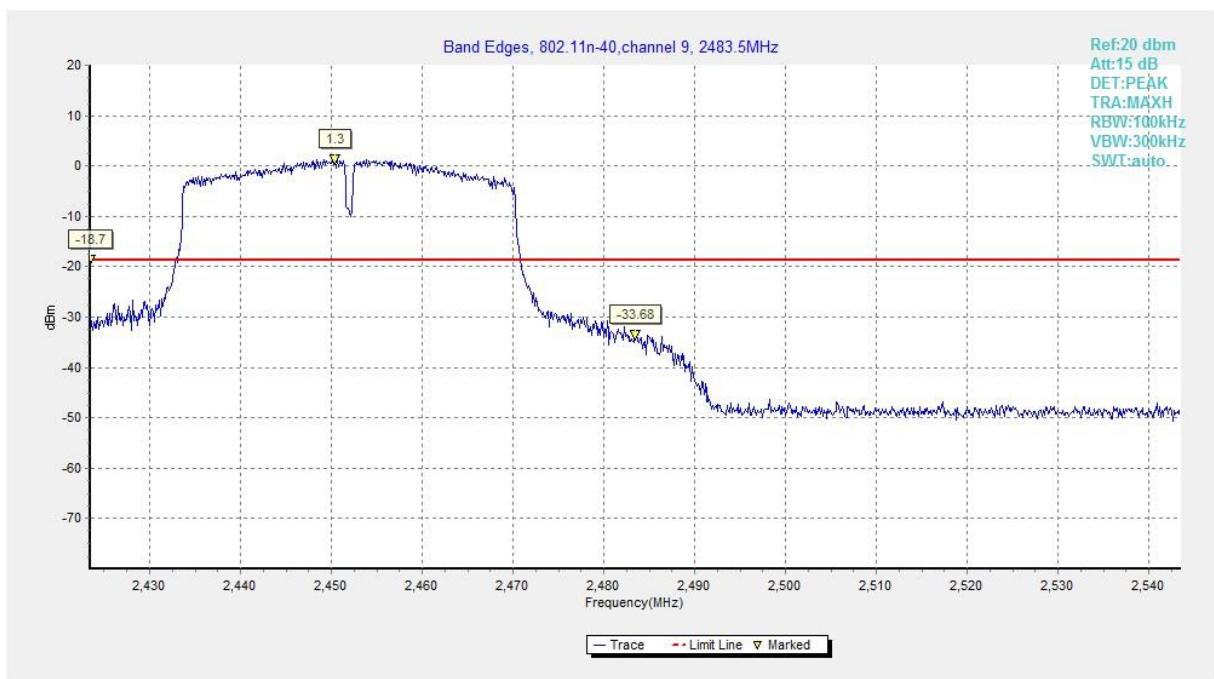
Fig.B.5.8 Band Edges (802.11n-HT40, Ch 9)
