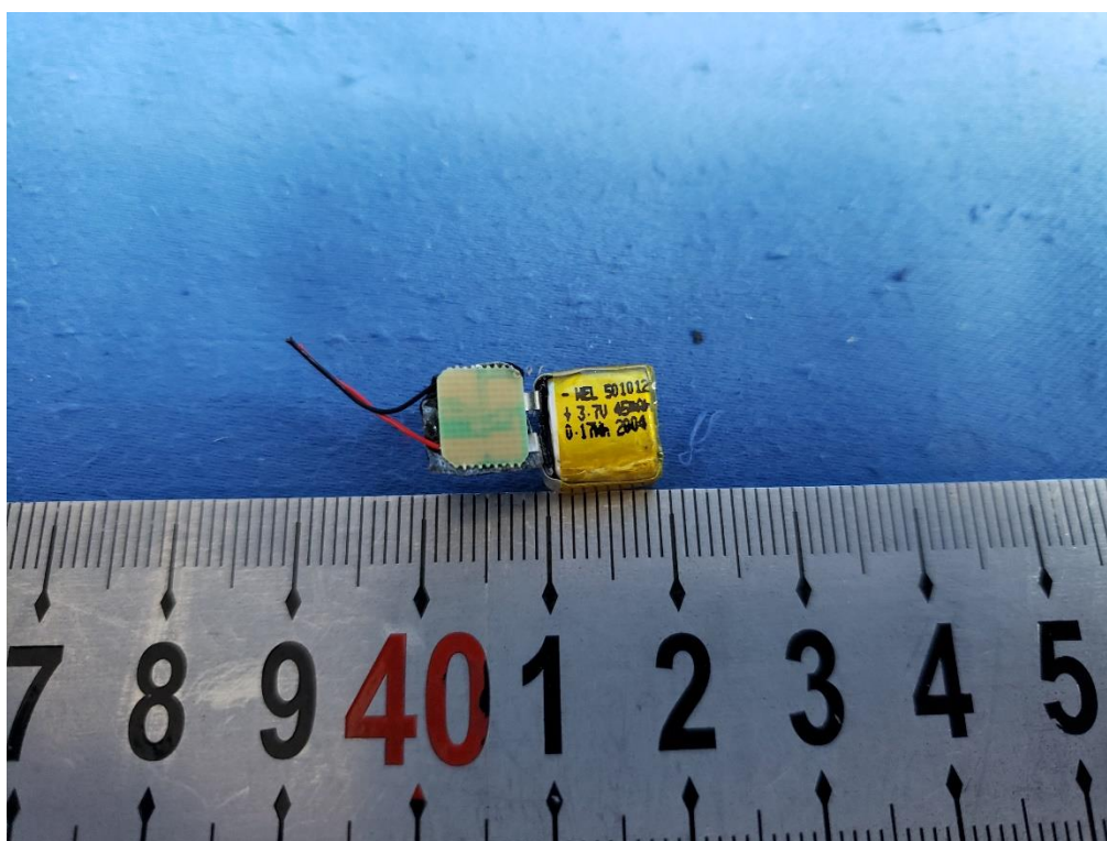
Right earbud
