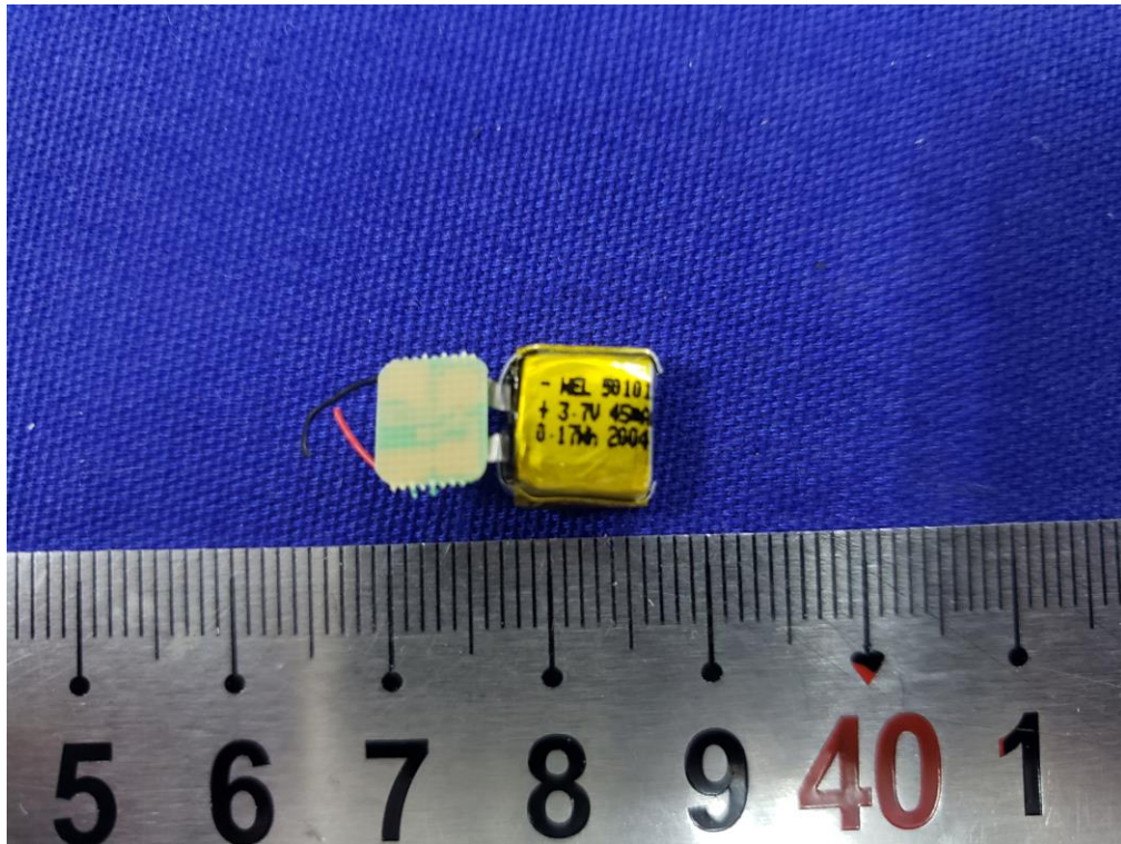
Left earbud
