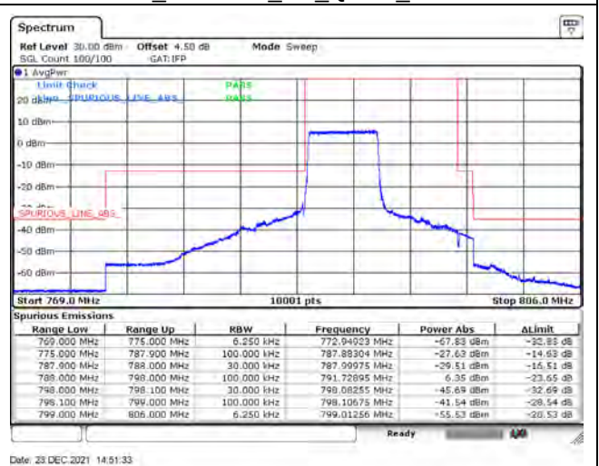
B14_CH23355_5M_QPSK_25RB0
