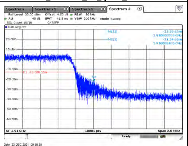
B2_CH19175_5M_QPSK_25RB0
