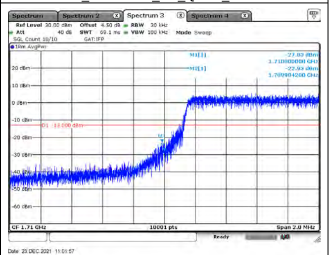
B66_CH131987_3M_QPSK_15RB0
