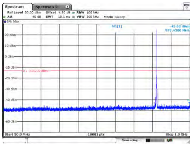
B5_CH20415_3M_1RB0_QPSK_Below 1G
