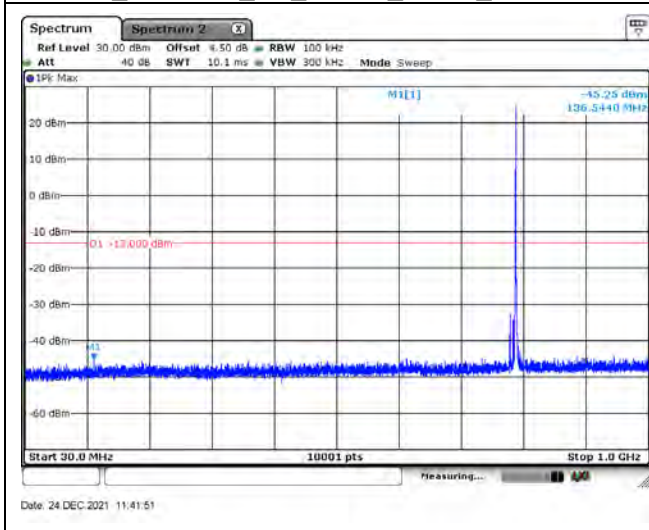
B14_CH23355_5M_1RB12_QPSK_Below 1G
