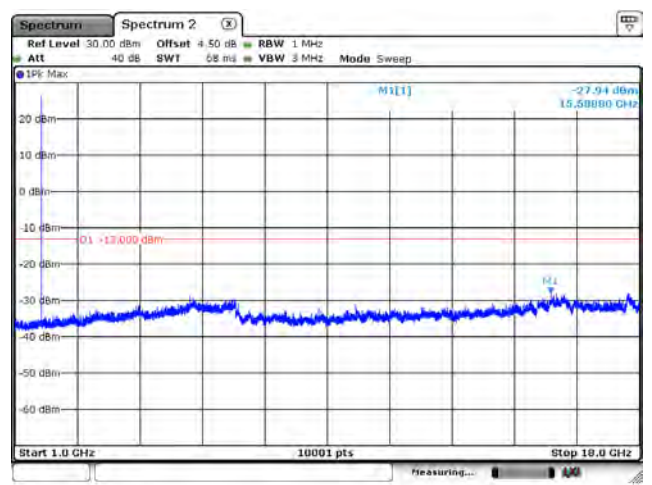
B66_CH131979_1.4M_1RB0_QPSK_Above 1G
