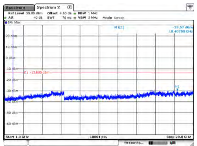
B2_CH18700_20M_1RB0_QPSK_Above 1G
