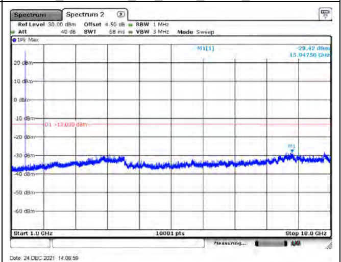
B66_CH132322_5M_1RB0_QPSK_Above 1G
