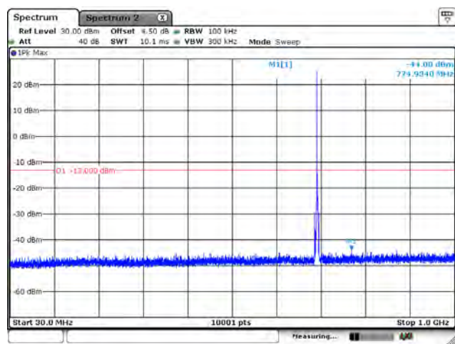
B12_CH23025_3M_1RB0_QPSK_Below 1G
