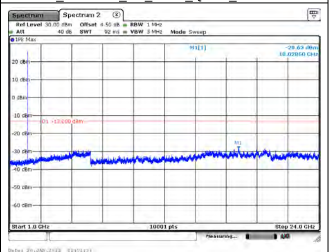
B30_CH27735_5M_1RB0_QPSK_Above 1G
