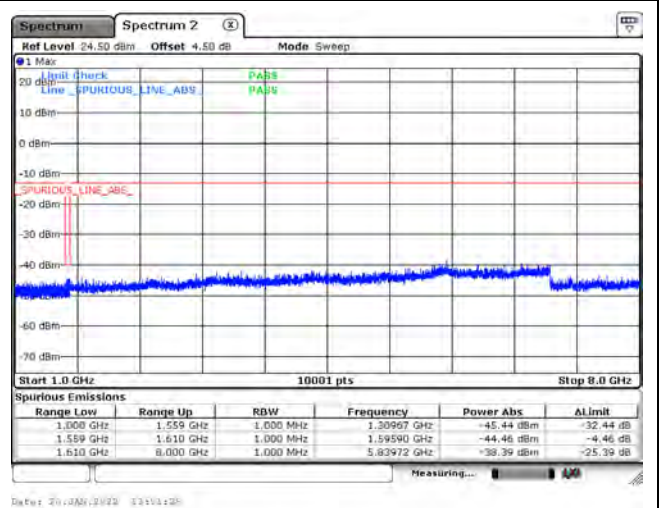
B14_CH23355_5M_1RB12_QPSK_Above 1G
