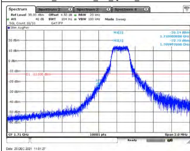
B66_CH131987_3M_QPSK_1RB0
