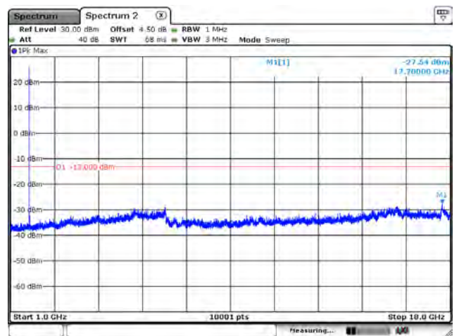
B66_CH132047_15M_1RB0_Above 1G
