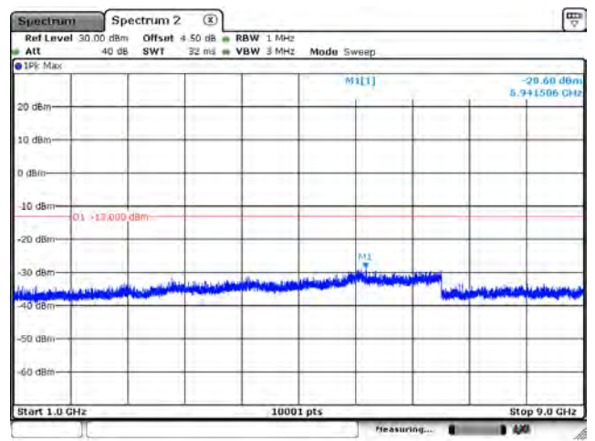
B5_CH20415_3M_1RB0_QPSK_Above 1G
