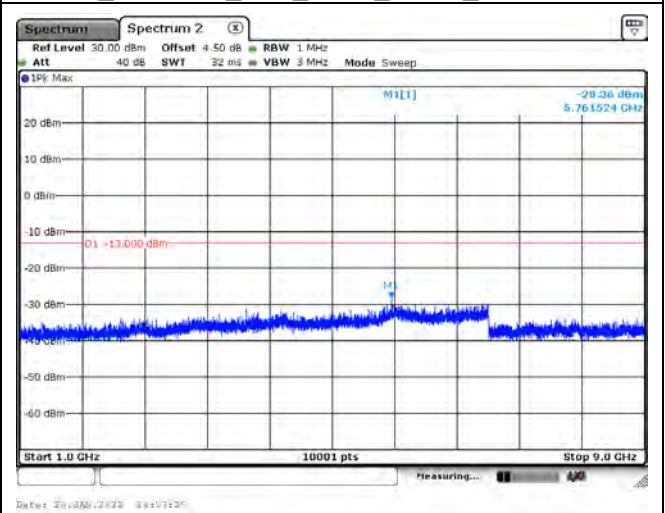
B5_CH20525_10M_1RB0_QPSK_Above 1G
