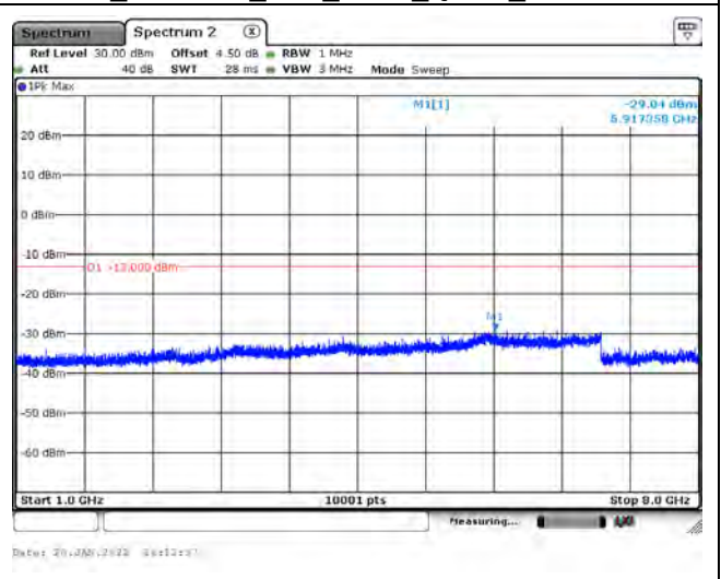
B12_CH23095_10M_1RB0_QPSK_Above 1G
