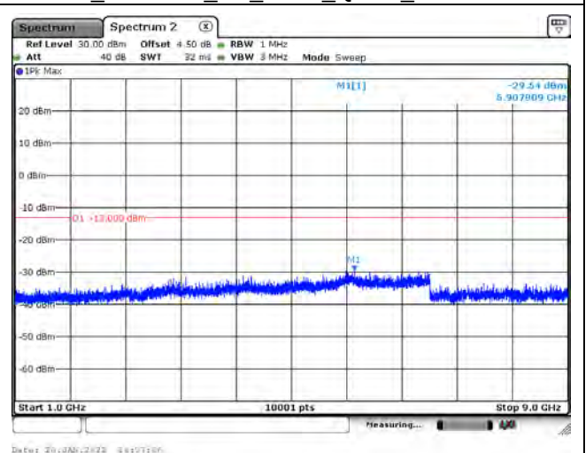
B5_CH20625_5M_1RB0_QPSK_Above 1G
