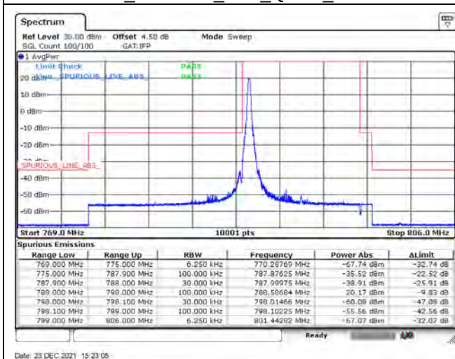
B14_CH23330_10M_QPSK_1RB0
