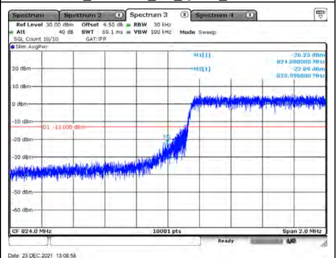
B5_CH20415_3M_QPSK_15RB0
