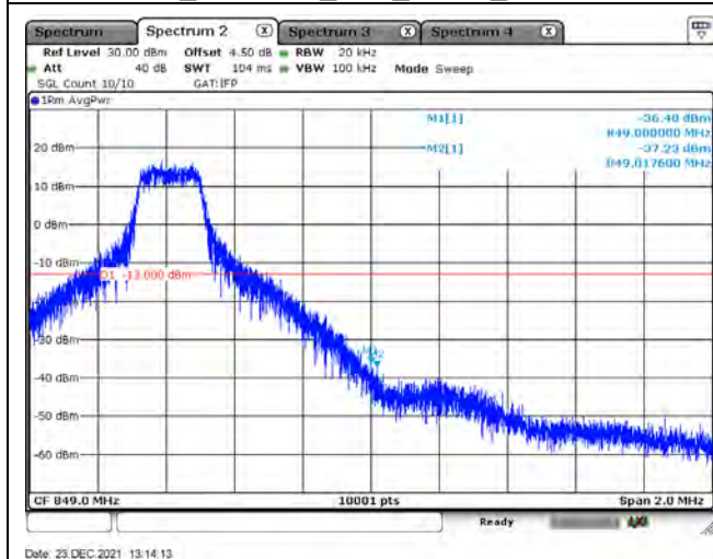
B5_CH20600_10M_QPSK_1RB49
