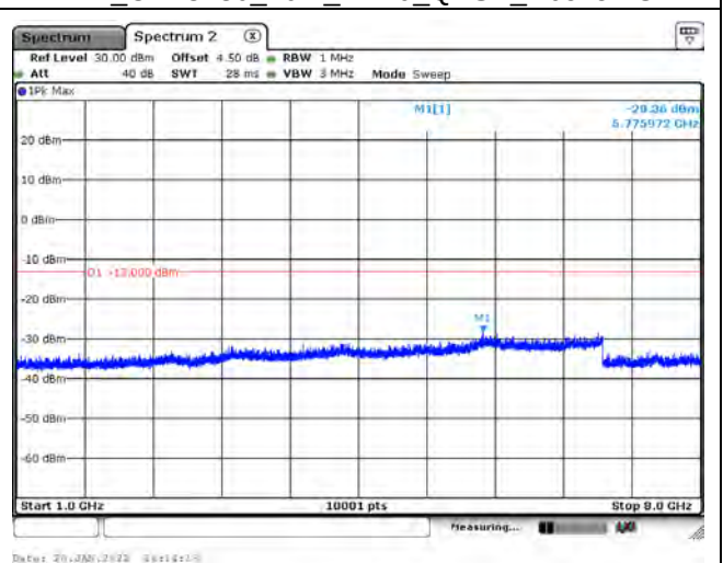
B12_CH23130_10M_1RB0_QPSK_Above 1G
