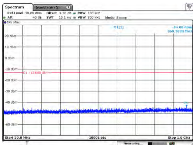
B66_CH132597_15M_1RB0_QPSK_Below 1G
