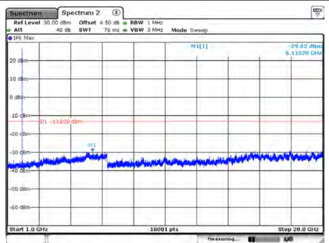
B2_CH18900_20M_1RB0_QPSK_Above 1G
