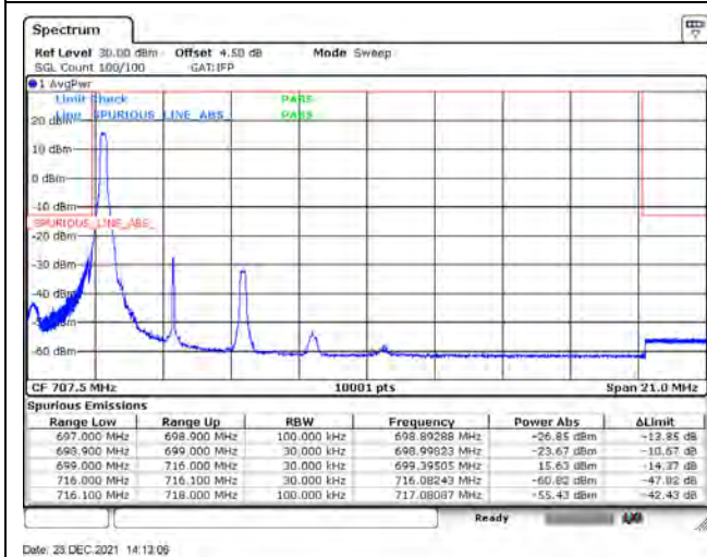
B12_CH23155_5M_QPSK_1RB24
