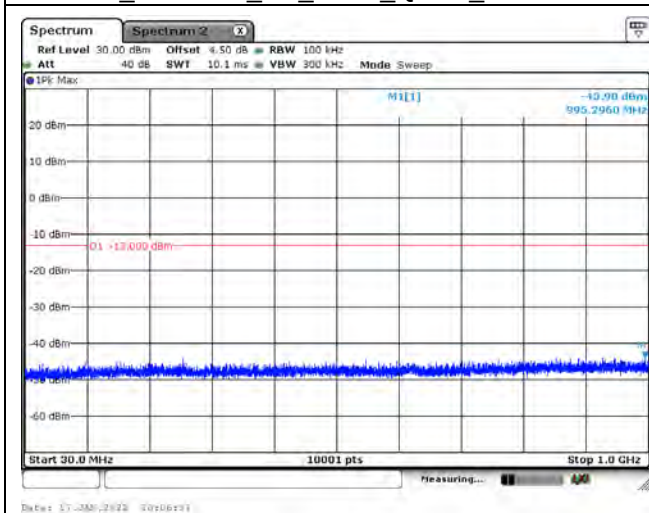
B30_CH27735_5M_1RB0_QPSK_Below 1G
