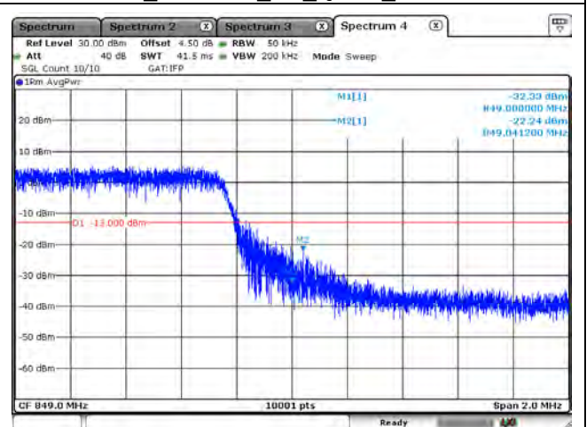
B5_CH20625_5M_QPSK_25RB0
