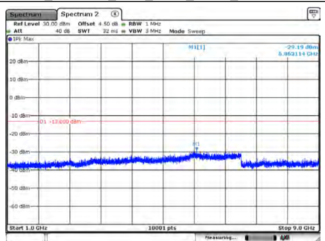
B5_CH20643_1.4M_1RB0_QPSK_Above 1G
