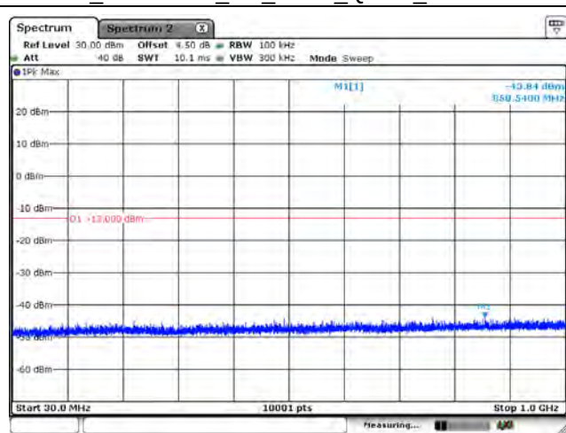
B66_CH132657_3M_1RB0_QPSK_Below 1G
