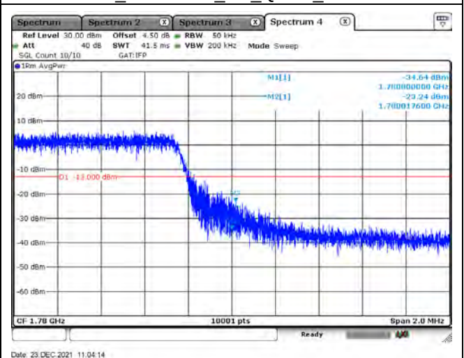
B66_CH132647_5M_QPSK_25RB0
