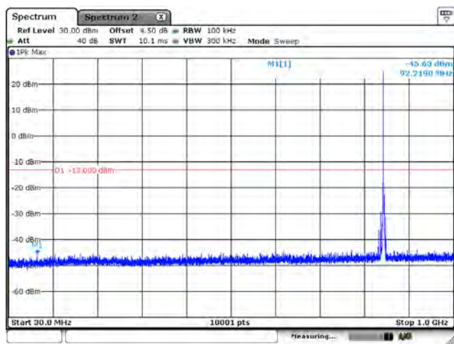
B5_CH20635_3M_1RB0_QPSK_Below 1G
