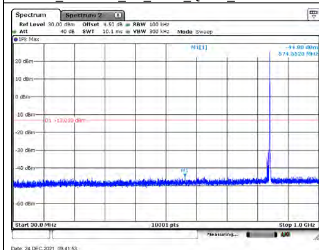
B5_CH20625_5M_1RB0_QPSK_Below 1G
