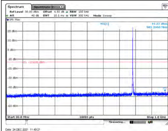
B14_CH23330_5M_1RB12_QPSK_Below 1G
