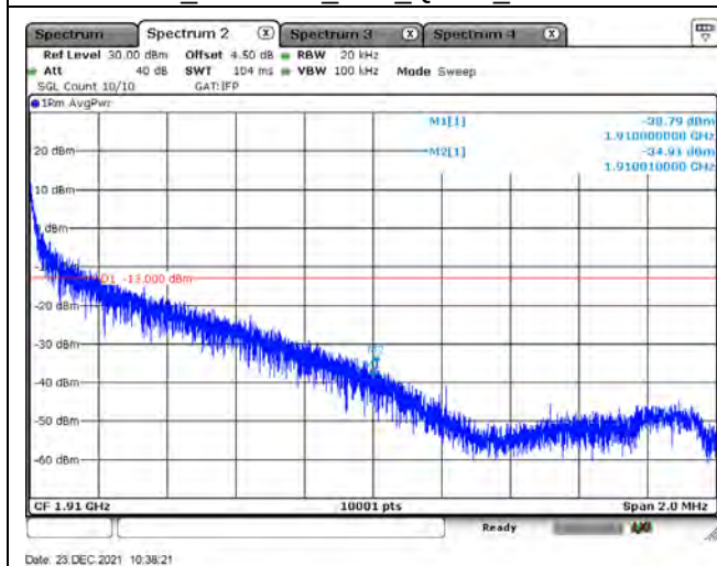
B2_CH19100_20M_QPSK_1RB99
