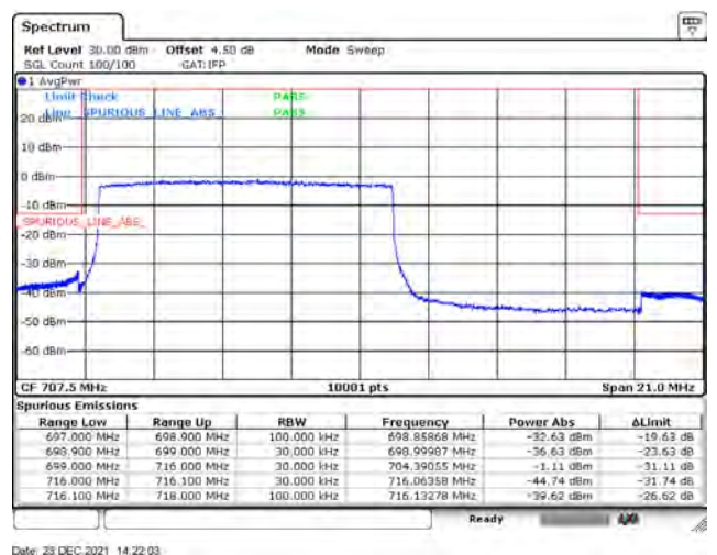
B12_CH23130_10M_QPSK_50RB0
