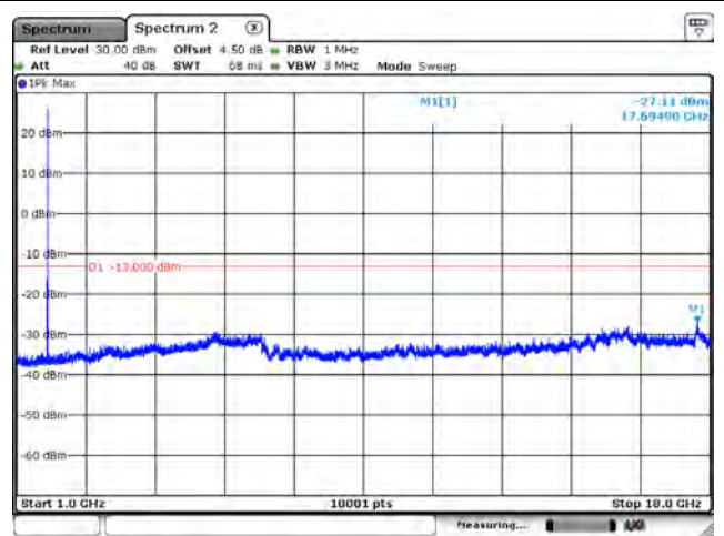
B66_CH132322_1.4M_1RB0_QPSK_Above 1G
