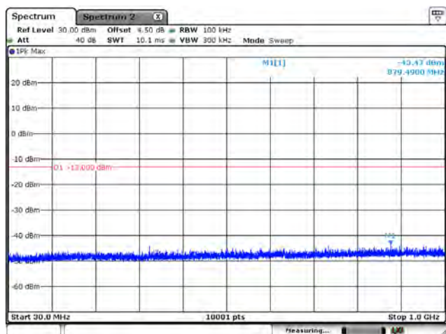
B66_CH132322_15M_1RB0_QPSK_Below 1G
