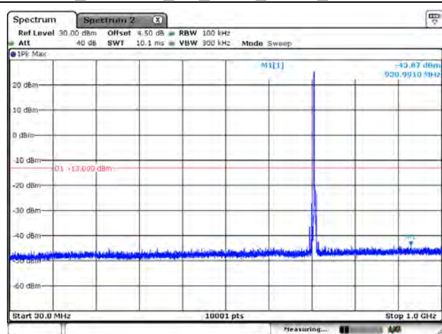
B12_CH23165_3M_1RB0_QPSK_Below 1G
