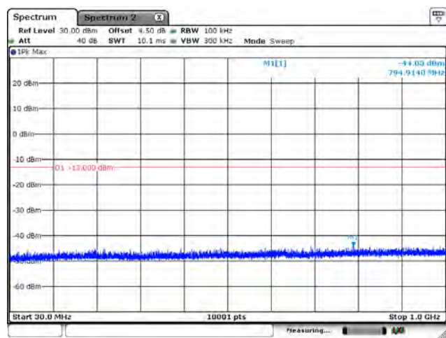
B2_CH18700_20M_1RB0_QPSK_Below 1G
