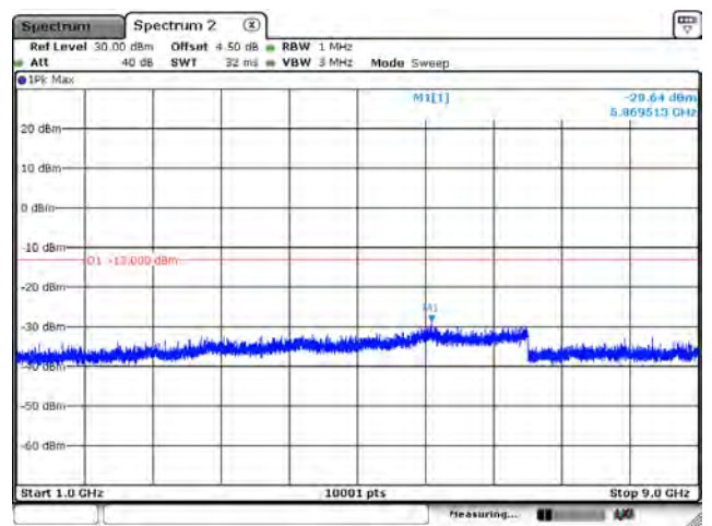
B5_CH20635_3M_1RB0_QPSK_Above 1G
