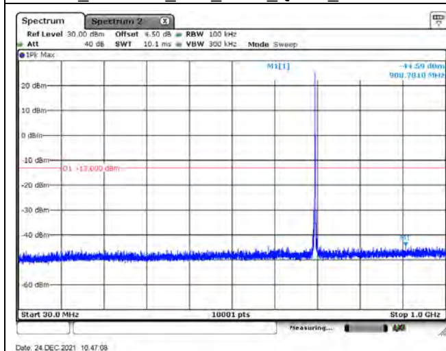
B12_CH23130_10M_1RB0_QPSK_Below 1G
