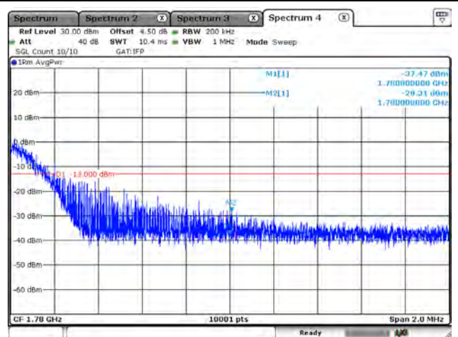
B66_CH132572_20M_QPSK_100RB0
