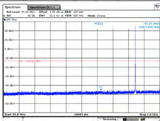
B5_CH20643_1.4M_1RB0_QPSK_Below 1G
