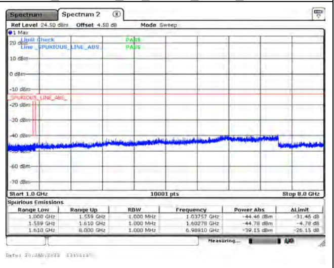
B14_CH23355_5M_1RB12_QPSK_Above 1G
