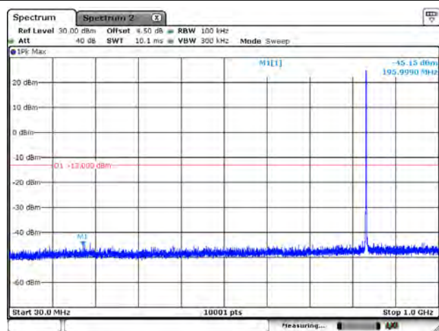
B5_CH20525_1.4M_1RB0_QPSK_Below 1G
