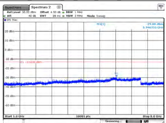
B12_CH23165_3M_1RB0_QPSK_Above 1G
