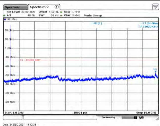
B66_CH132322_10M_1RB0_QPSK_Above 1G
