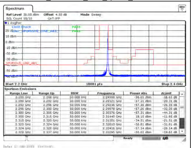
B30_CH27710_10M_QPSK_1RB49
