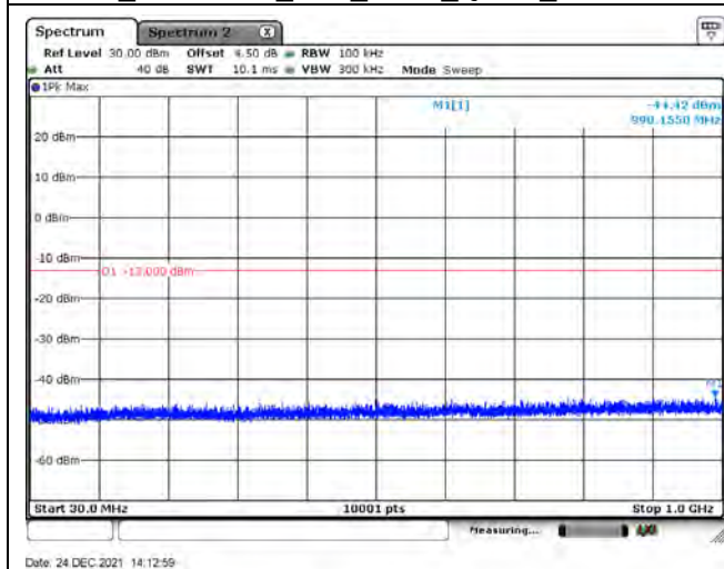
B66_CH132622_10M_1RB0_QPSK_Below 1G
