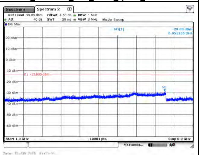
B12_CH23130_10M_1RB0_QPSK_Above 1G
