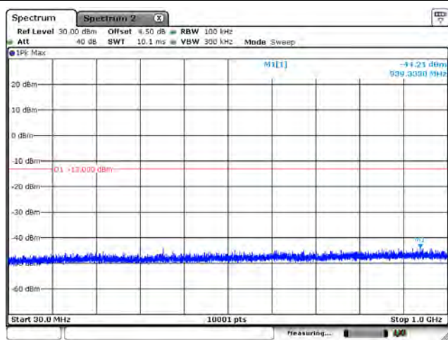
B66_CH132322_1.4M_1RB0_QPSK_Below 1G
