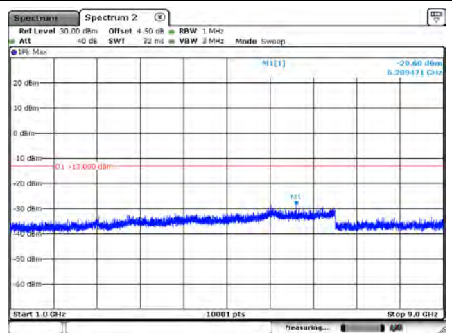
B5_CH20525_1.4M_1RB0_QPSK_Above 1G
