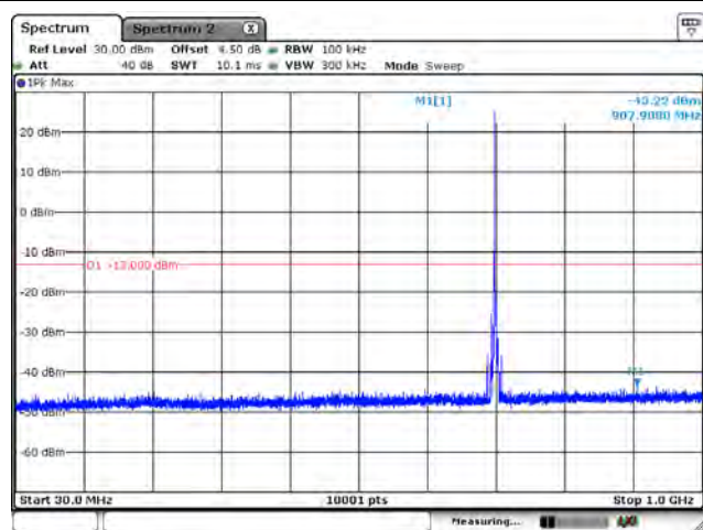
B12_CH23095_3M_1RB0_QPSK_Below 1G
