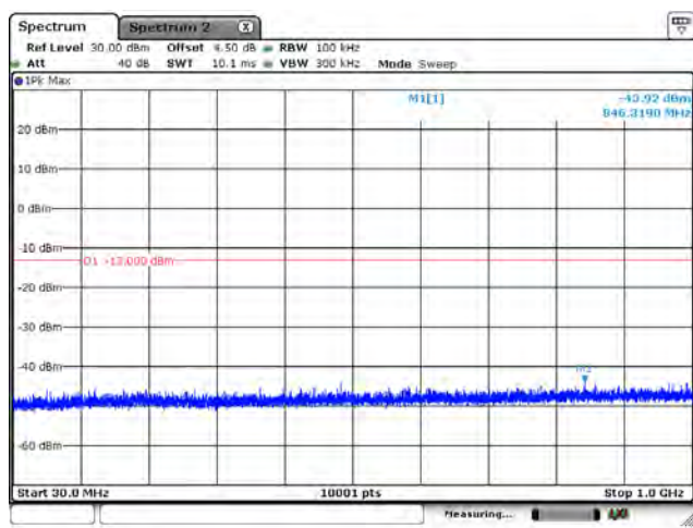
B66_CH131979_1.4M_1RB0_QPSK_Below 1G
