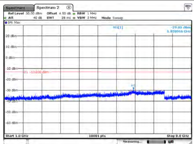
B12_CH23095_3M_1RB0_QPSK_Above 1G
