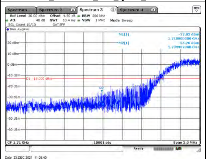
B66_CH132047_15M_QPSK_75RB0
