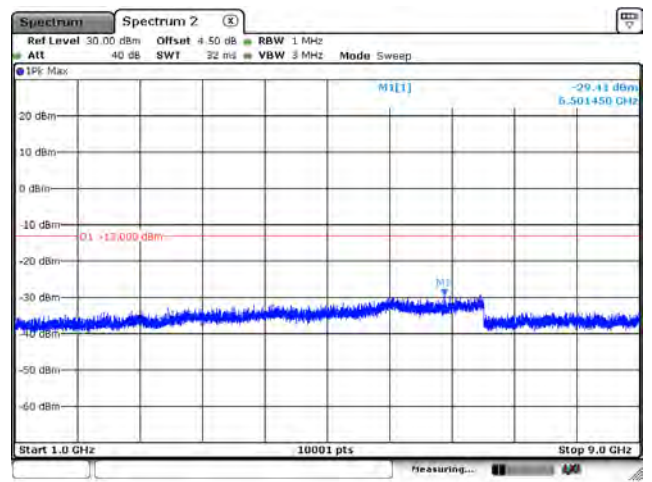
B5_CH20525_3M_1RB0_QPSK_Above 1G
