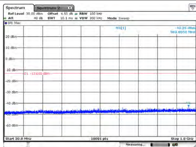
B2_CH18900_20M_1RB0_QPSK_Below 1G
