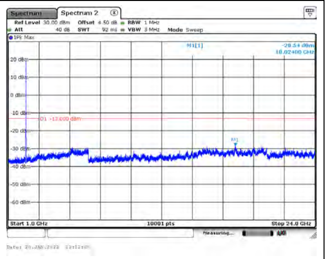
B30_CH27710_10M_1RB0_QPSK_Above 1G
