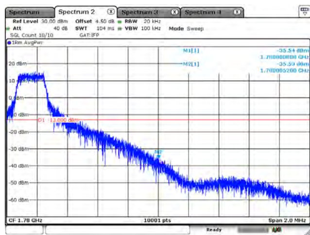
B66_CH132597_15M_QPSK_1RB74
