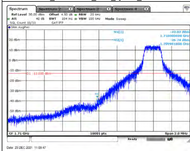
B66_CH132622_10M_QPSK_1RB49
