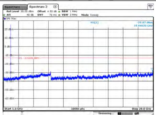
B2_CH19100_20M_1RB0_QPSK_Above 1G
