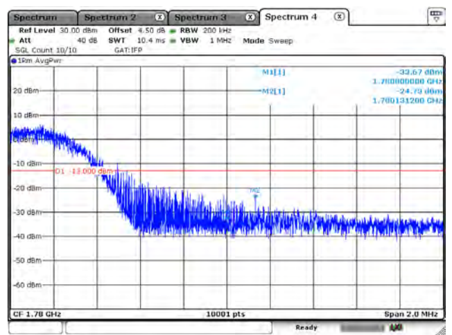
B66_CH132597_15M_QPSK_75RB0
