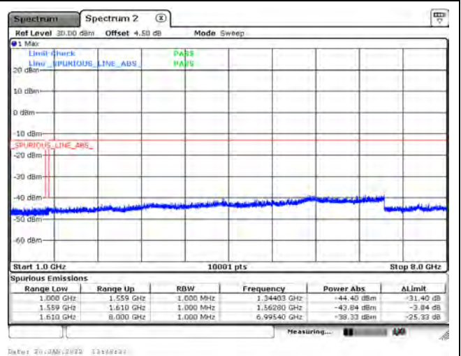
B14_CH23330_5M_1RB12_QPSK_Above 1G
