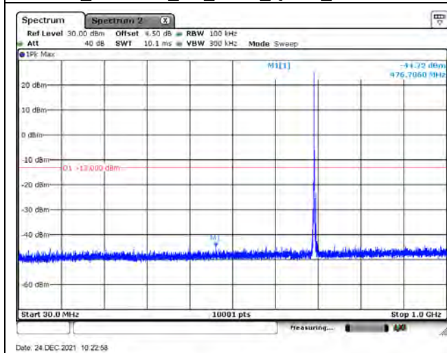
B12_CH23095_5M_1RB0_QPSK_Below 1G
