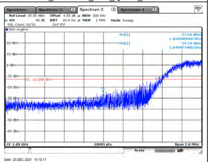
B2_CH18675_15M_QPSK_75RB0
