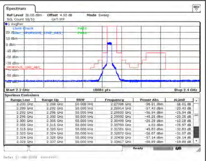
B30_CH27735_5M_QPSK_25RB0
