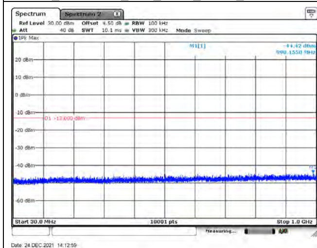
B66_CH132322_10M_1RB0_QPSK_Below 1G
