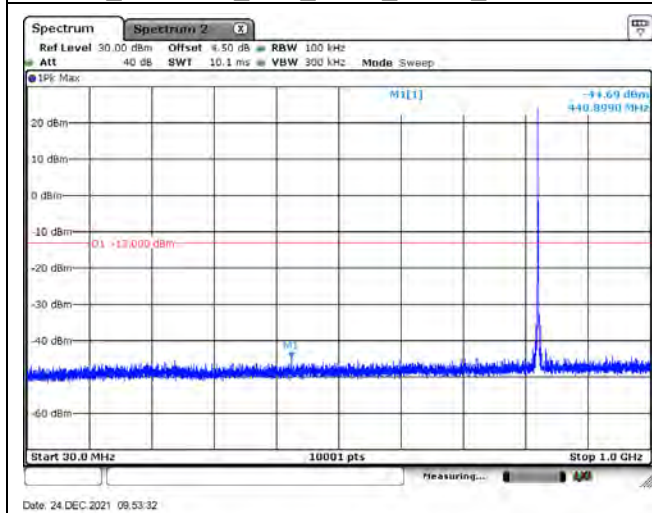
B5_CH20525_10M_1RB0_QPSK_Below 1G
