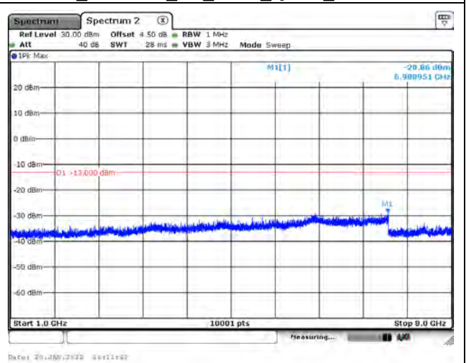
B12_H23095_5M_1RB0_QPSK_Above 1G
