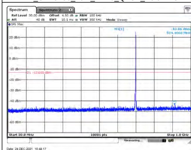
B12_CH23130_10M_1RB0_QPSK_Below 1G
