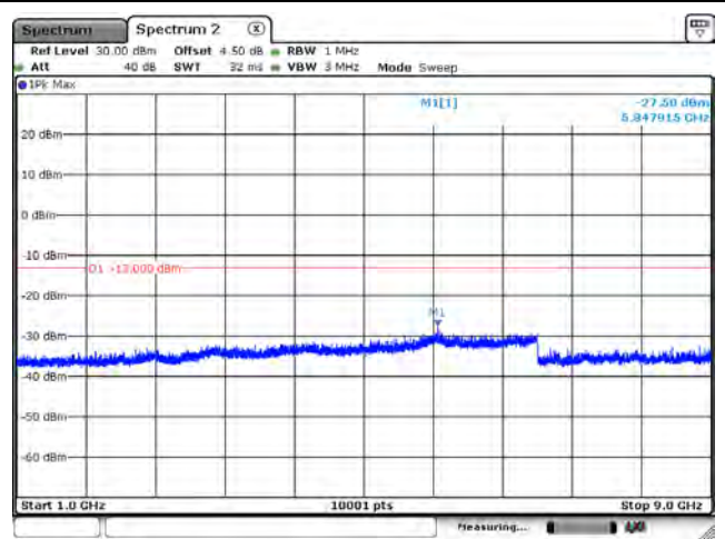
B5_CH20407_1.4M_1RB0_QPSK_Above 1G
