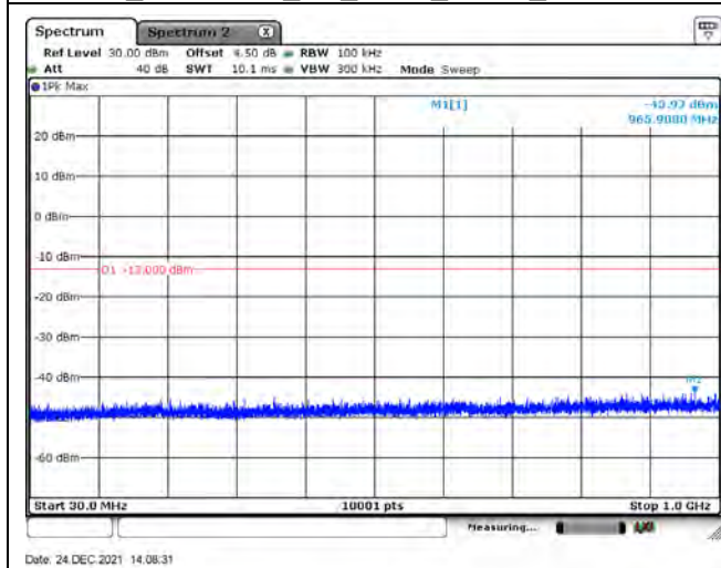
B66_CH132322_5M_1RB0_QPSK_Below 1G
