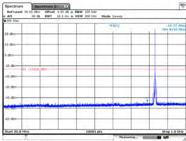
B5_CH20525_3M_1RB0_QPSK_Below 1G
