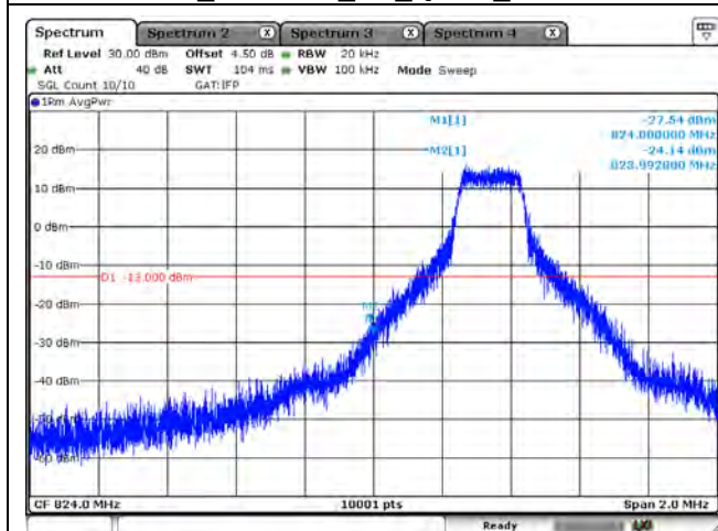
B5_CH20425_5M_QPSK_1RB0
