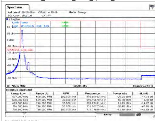
B12_CH23017_1.4M_QPSK_1RB0
