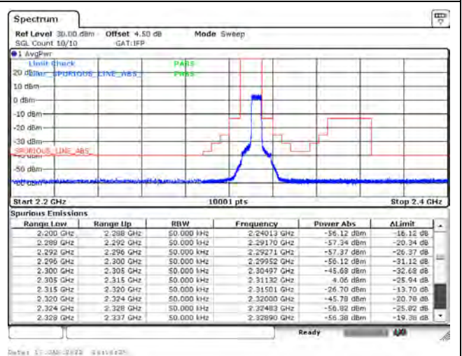
B30_CH27710_10M_QPSK_1RB49
