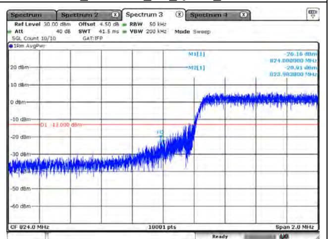
B5_CH20425_5M_QPSK_25RB0
