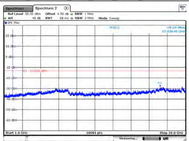
B66_CH132665_1.4M_1RB0_QPSK_Above 1G
