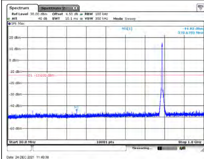
B14_CH23355_5M_1RB12_QPSK_Below 1G
