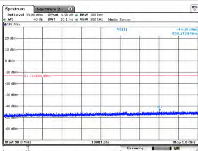
B66_CH132665_1.4M_1RB0_QPSK_Below 1G
