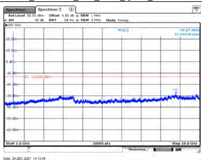
B66_CH132622_10M_1RB0_QPSK_Above 1G
