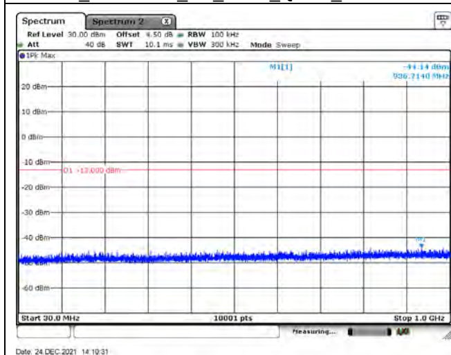
B66_CH132647_5M_1RB0_QPSK_Below 1G
