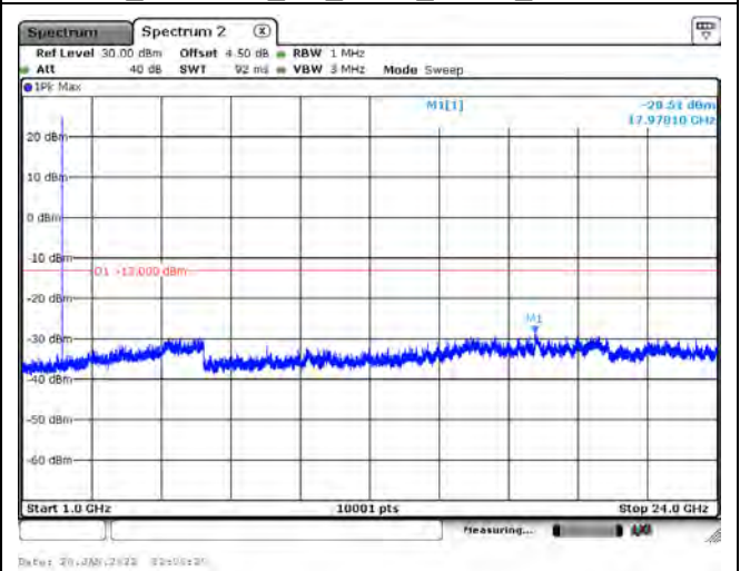
B30_CH27710_5M_1RB0_QPSK_Above 1G
