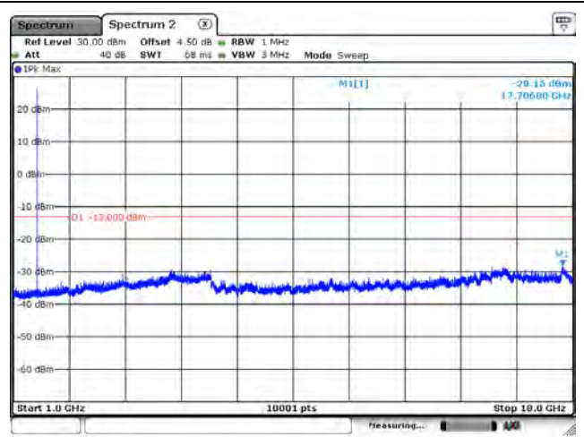
B66_CH131987_3M_1RB0_QPSK_Above 1G
