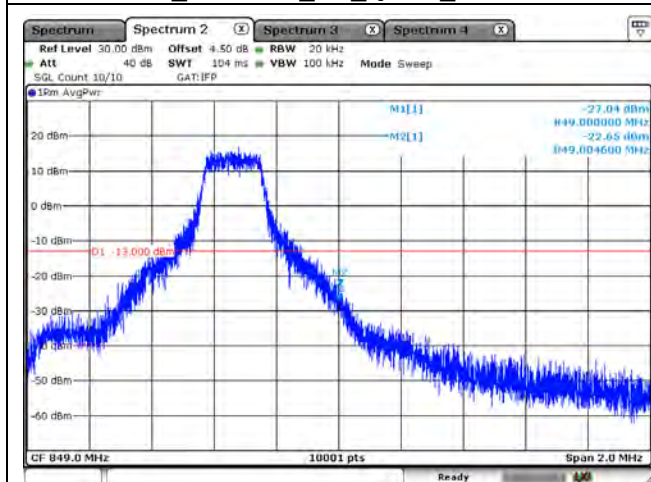
B5_CH20625_5M_QPSK_1RB24
