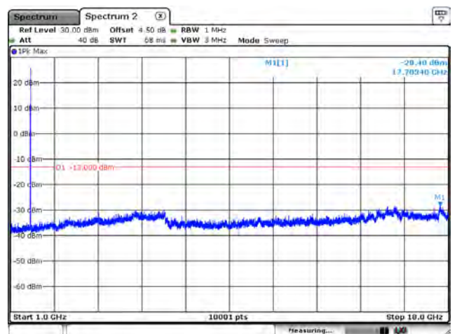
B66_CH132597_15M_1RB0_QPSK_Above 1G
