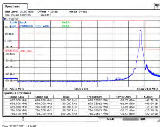
B12_CH23130_10M_QPSK_1RB49
