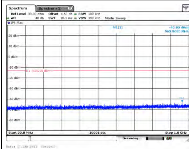
B30_CH27710_5M_1RB0_QPSK_Below 1G
