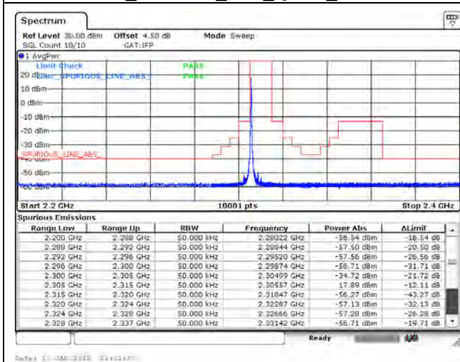
B30_CH27710_10M_QPSK_1RB0
