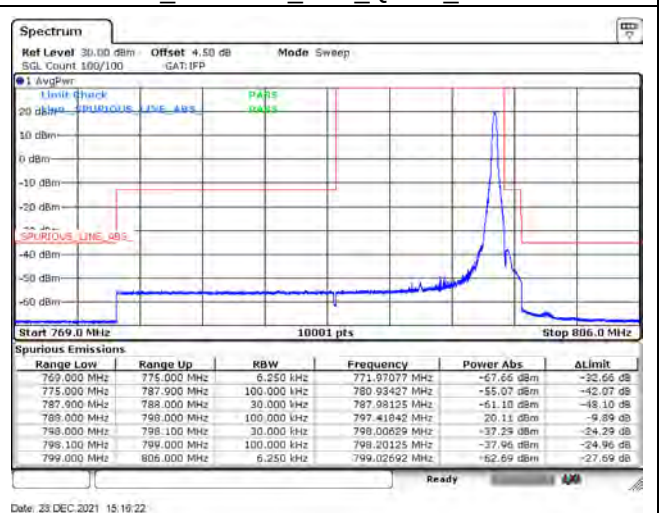
B14_CH23330_10M_QPSK_1RB49
