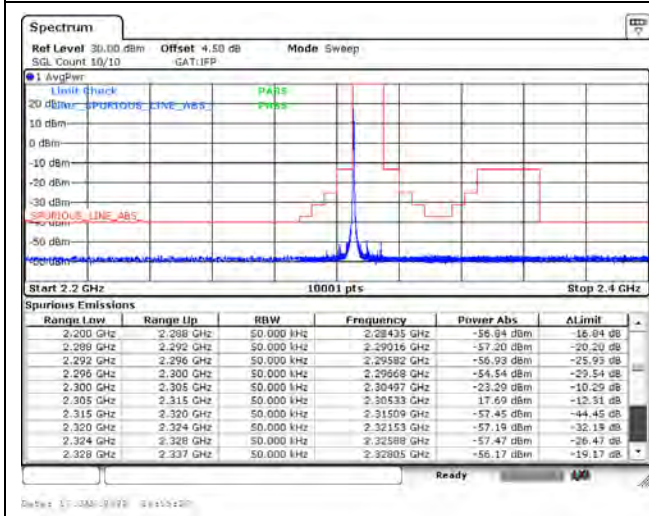
B30_CH27735_5M_QPSK_1RB24
