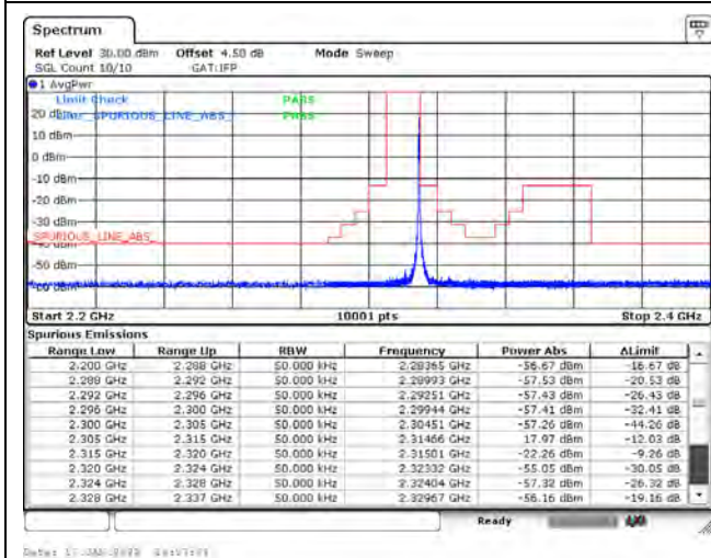
B30_CH27710_10M_QPSK_1RB0
