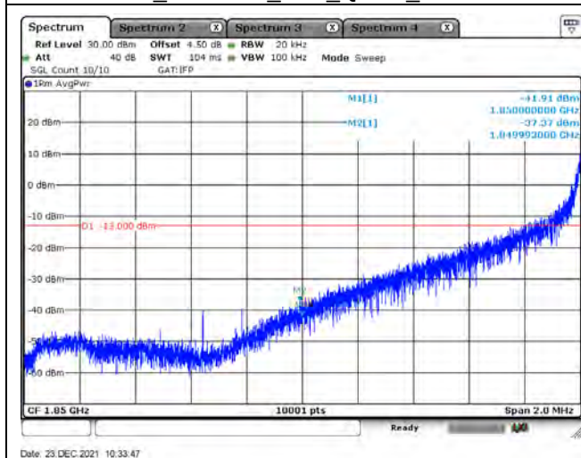
B2_CH19100_20M_QPSK_1RB99
