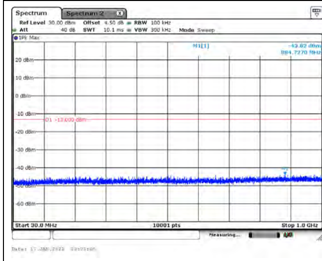
B30_CH27710_10M_1RB0_QPSK_Below 1G
