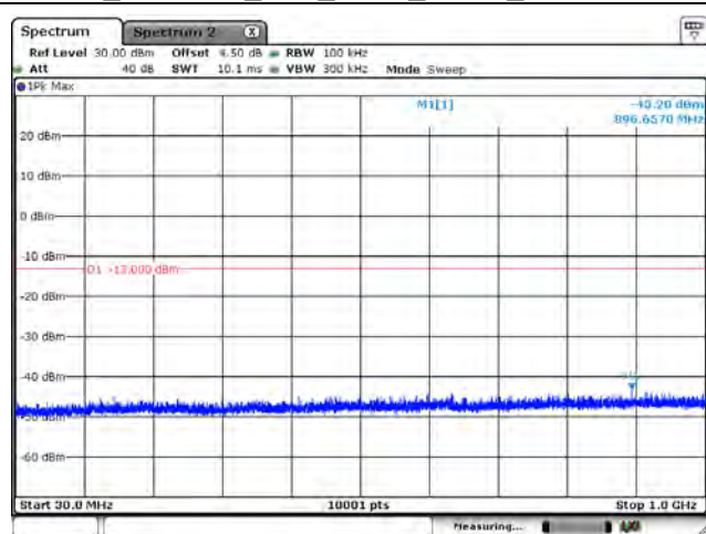
B2_CH19100_20M_1RB0_QPSK_Below 1G
