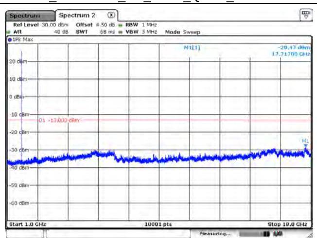
B66_CH132657_3M_1RB0_QPSK_Above 1G
