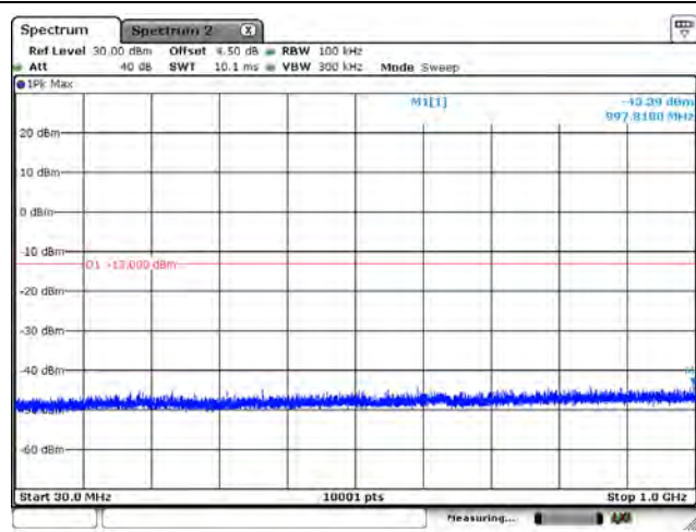
B66_CH131987_3M_1RB0_QPSK_Below 1G
