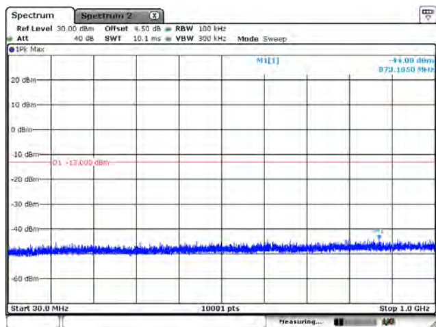
B66_CH132047_15M_1RB0_QPSK_Below 1G
