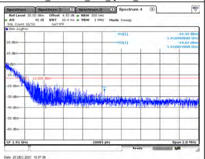
B2_CH19100_20M_QPSK_100RB0
