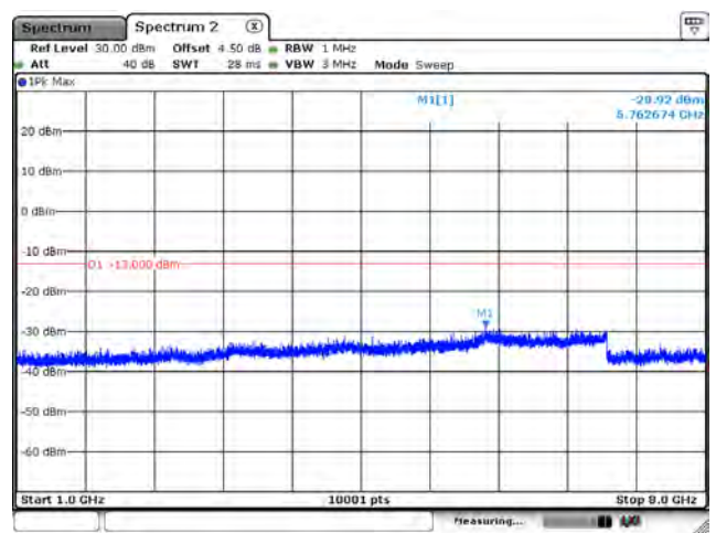
B12_CH23025_3M_1RB0_QPSK_Above 1G
