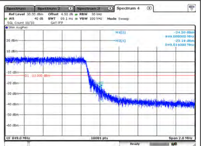
B5_CH20635_3M_QPSK_25RB0
