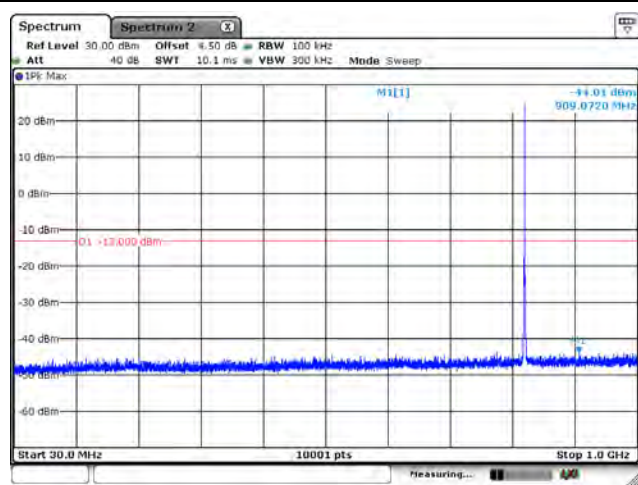
B5_CH20407_1.4M_1RB0_QPSK_Below 1G
