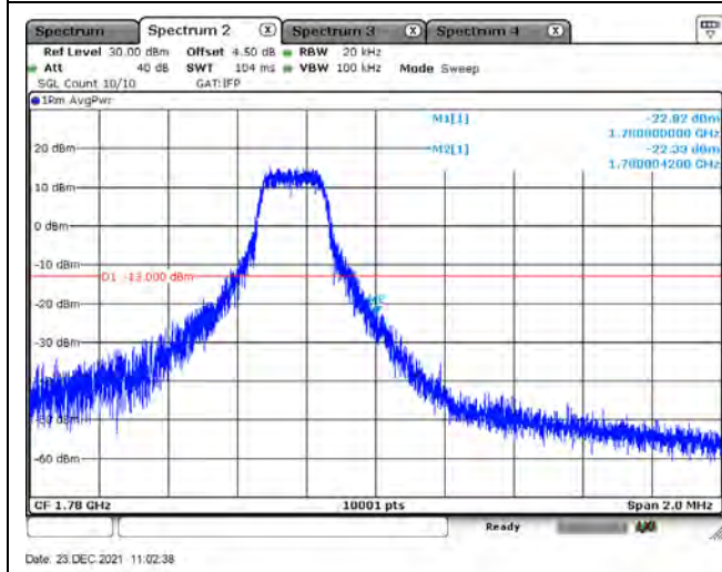
B66_CH131997_5M_QPSK_1RB0
