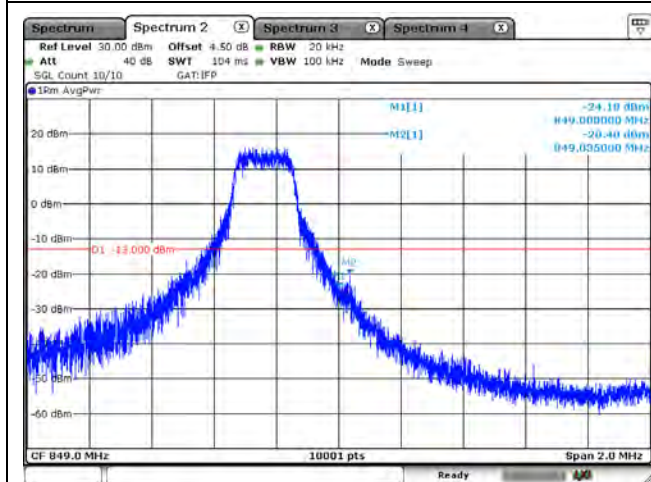
B5_CH20635_3M_QPSK_1RB0
