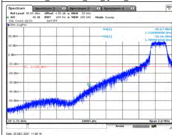
B66_CH132047_15M_QPSK_1RB0
