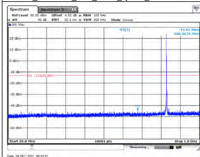
B5_CH20600_10M_1RB0_QPSK_Below 1G
