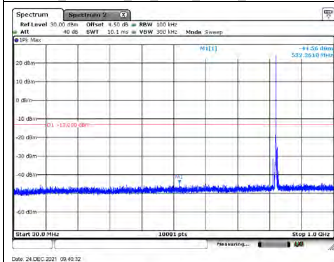
B5_CH20525_5M_1RB0_QPSK_Below 1G
