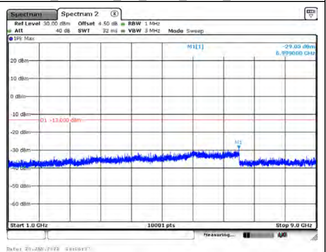
B5_CH20525_5M_1RB0_QPSK_Above 1G
