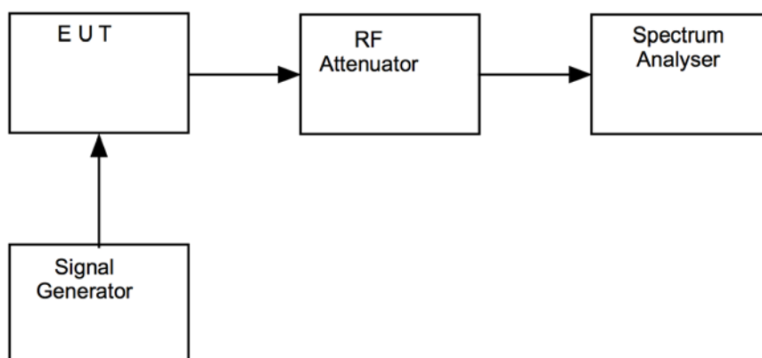
Figure vi Test Setup
