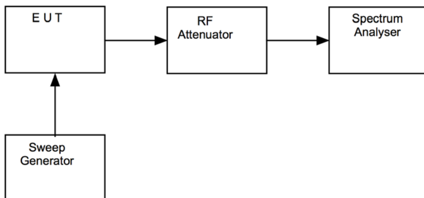
Figure v Test Setup
