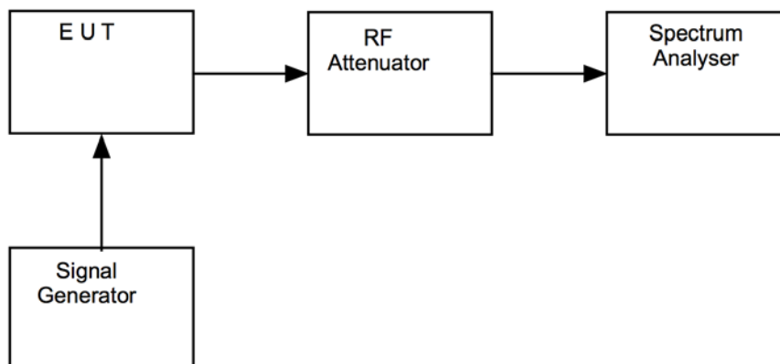
Figure iv Test Setup
