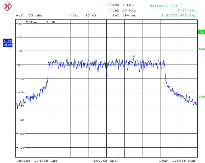
Power Spectral Density, Chain 0, 1.4MHz Low Channel
