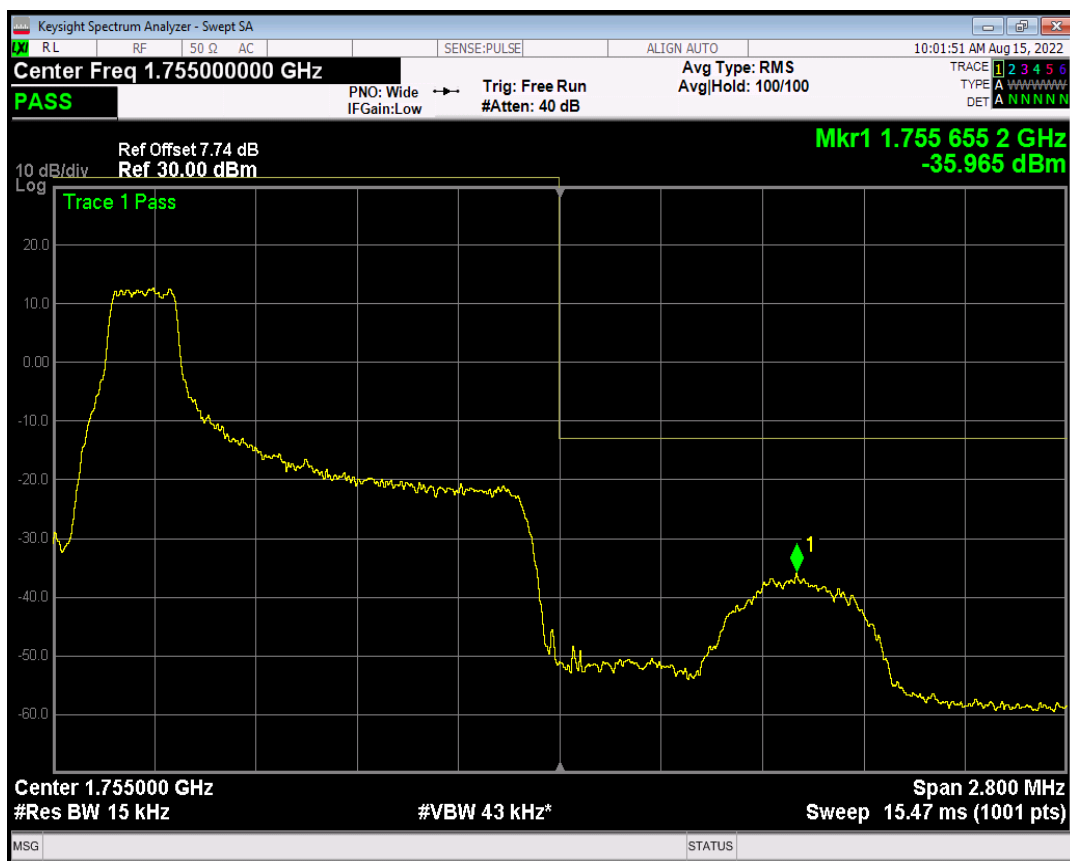
Band4 QAM16 BW=1.4MHz Channel=20393 RB Size=1 Position=#Max
