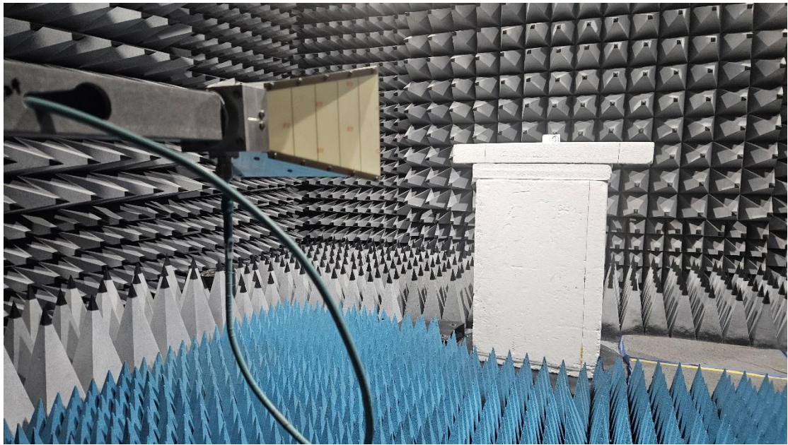
Radiated Emissions 1GHz -18GHz
