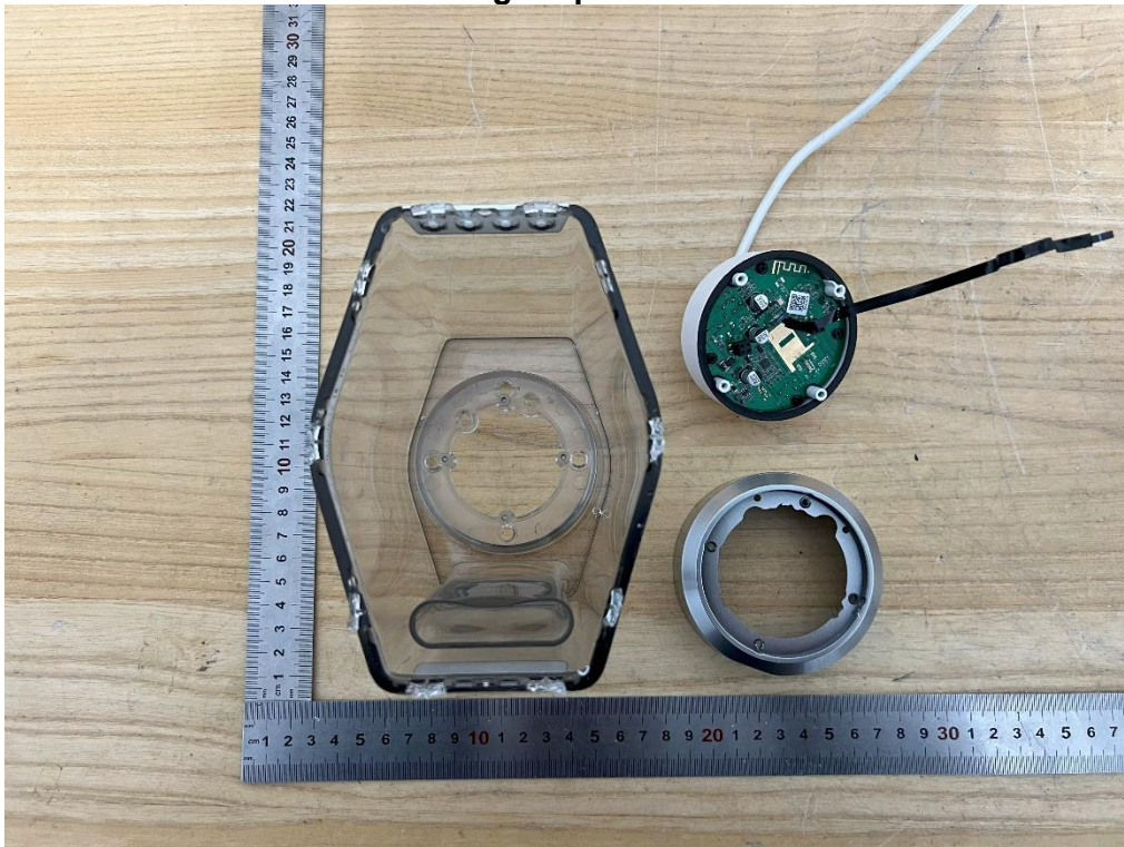
Internal View of EUT-26 Right Speaker
