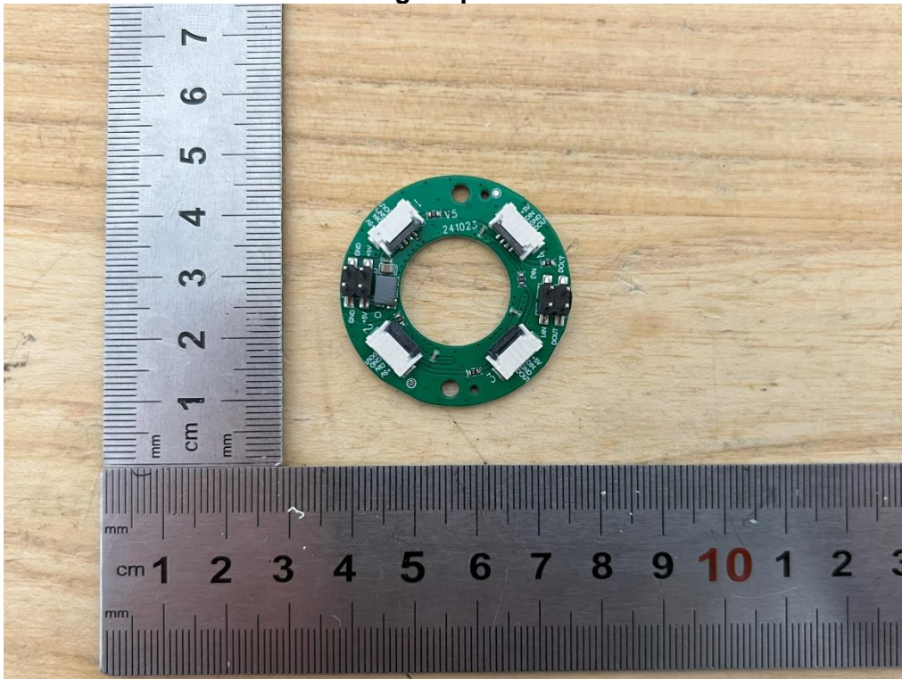
Internal View of EUT-24 Right Speaker
