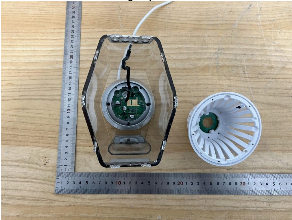
Internal View of EUT-20 Right Speaker
