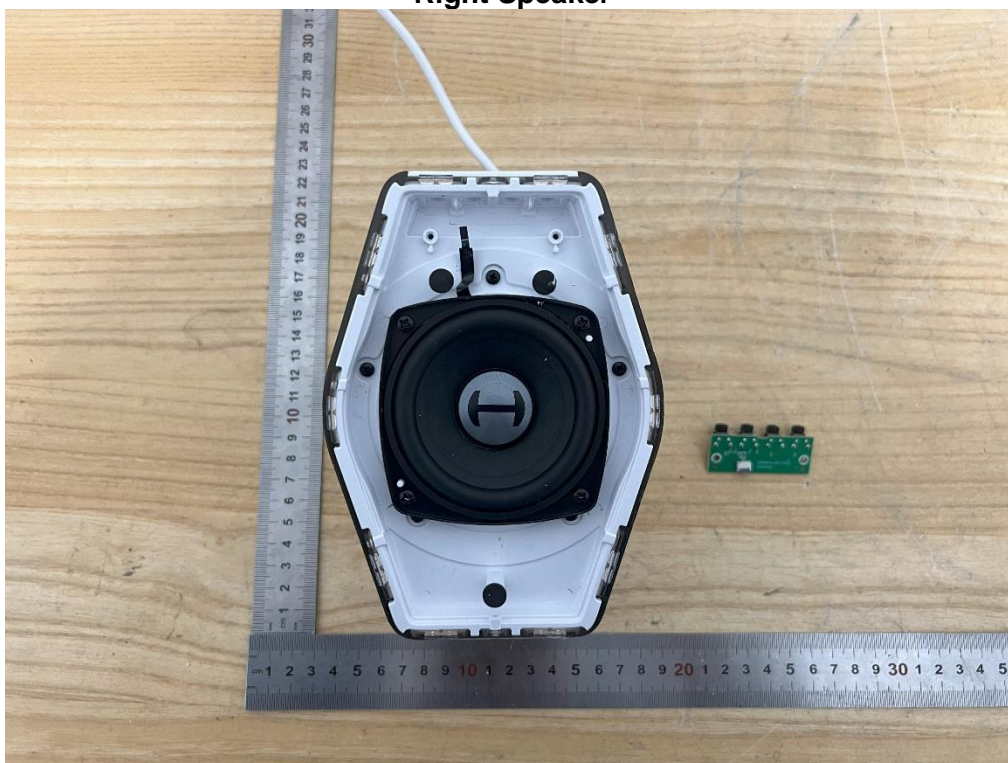
Internal View of EUT-14 Right Speaker
