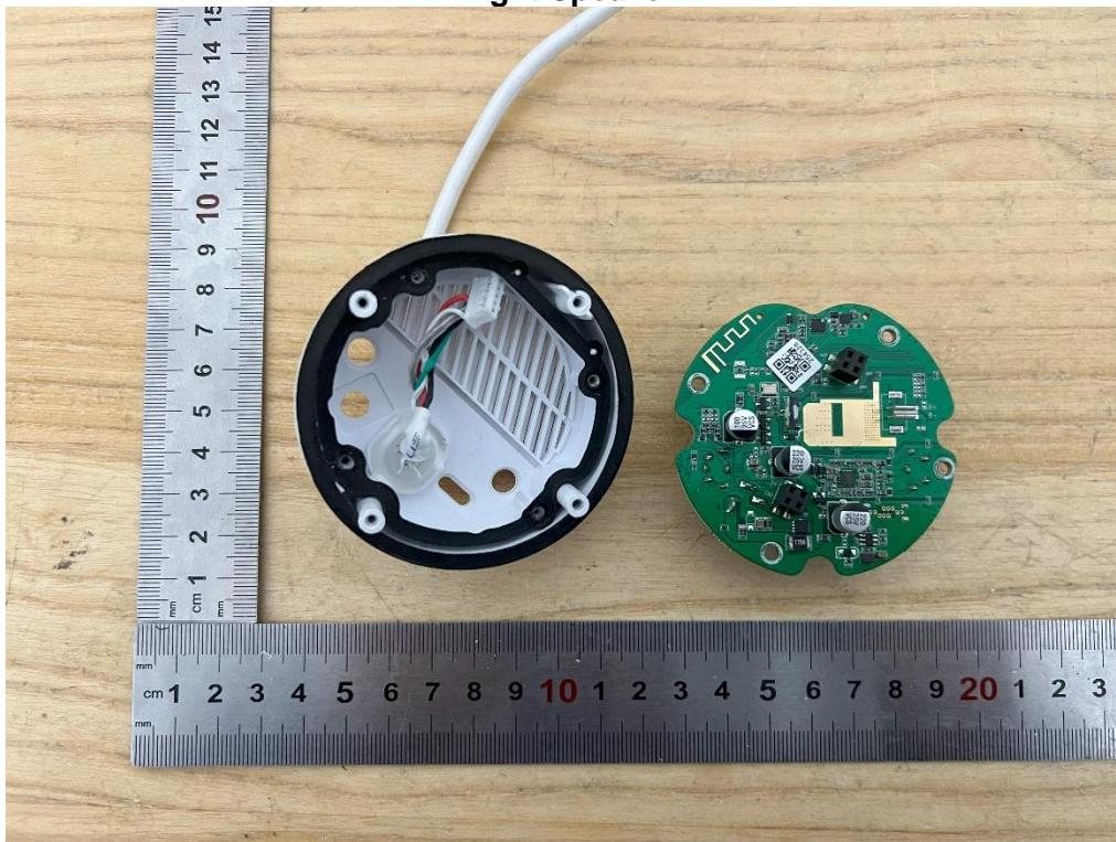
Internal View of EUT-28 Right Speaker
