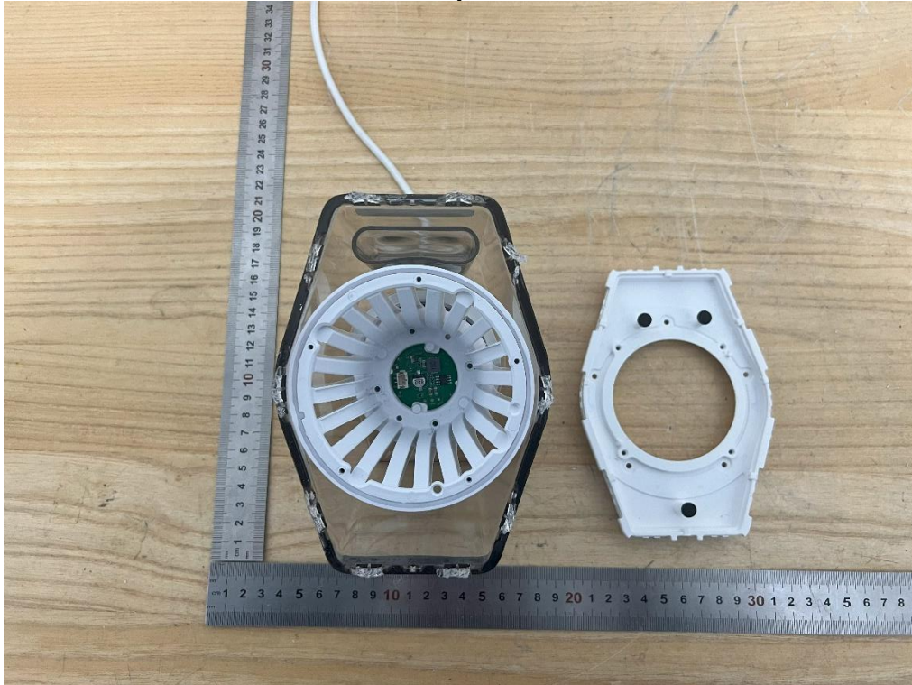
Internal View of EUT-5 Left Speaker
