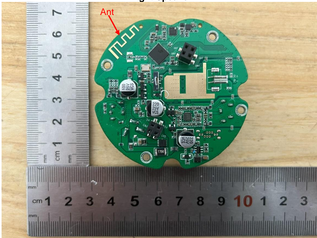
Internal View of EUT-30 Right Speaker
