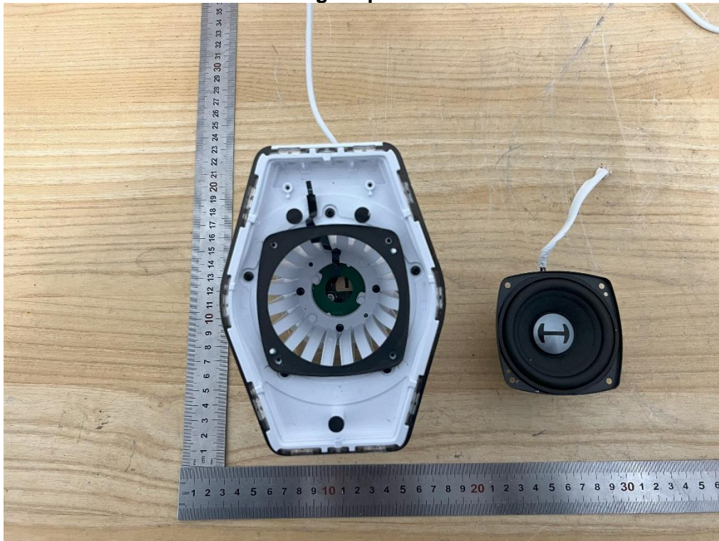
Internal View of EUT-16 Right Speaker
