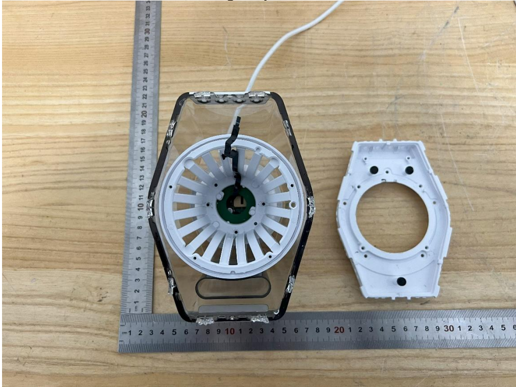
Internal View of EUT-19 Right Speaker
