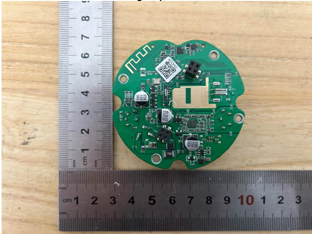
Internal View of EUT-29 Right Speaker
