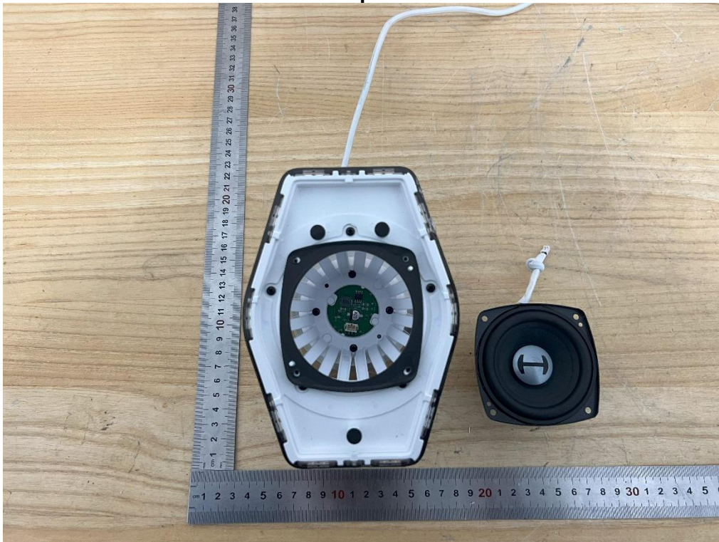
Internal View of EUT-2 Left Speaker
