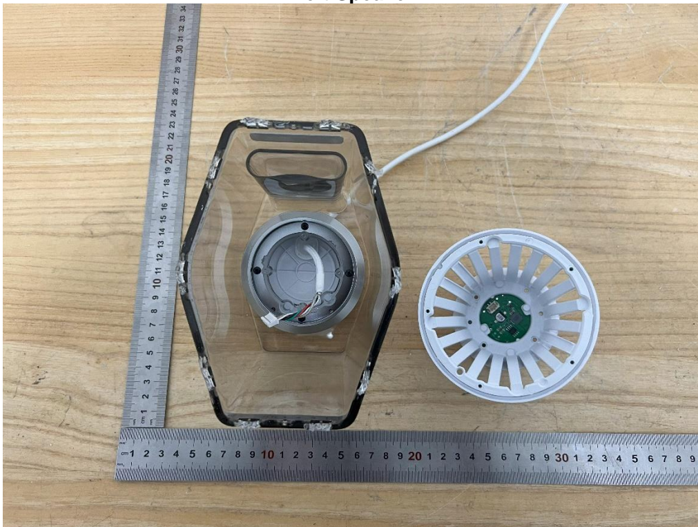
Internal View of EUT-6 Left Speaker
