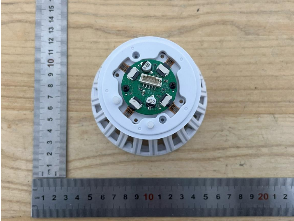
Internal View of EUT-7 Left Speaker
