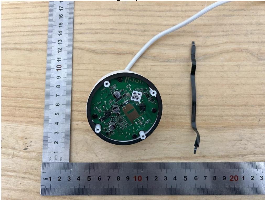
Internal View of EUT-27 Right Speaker
