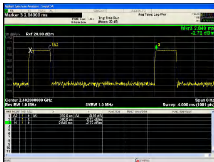
Test Mode: BDR---DH1
