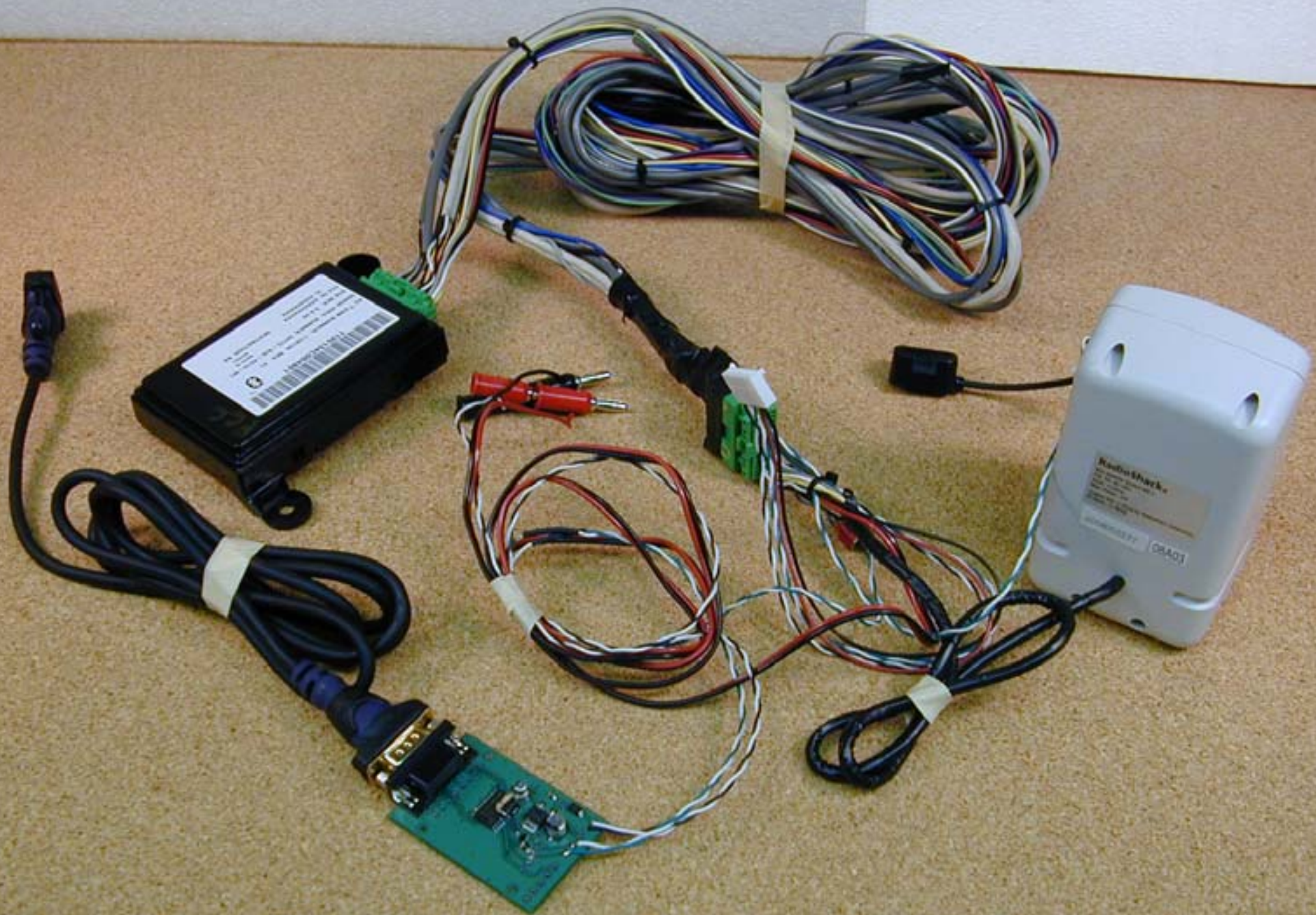
DUT with Harness
