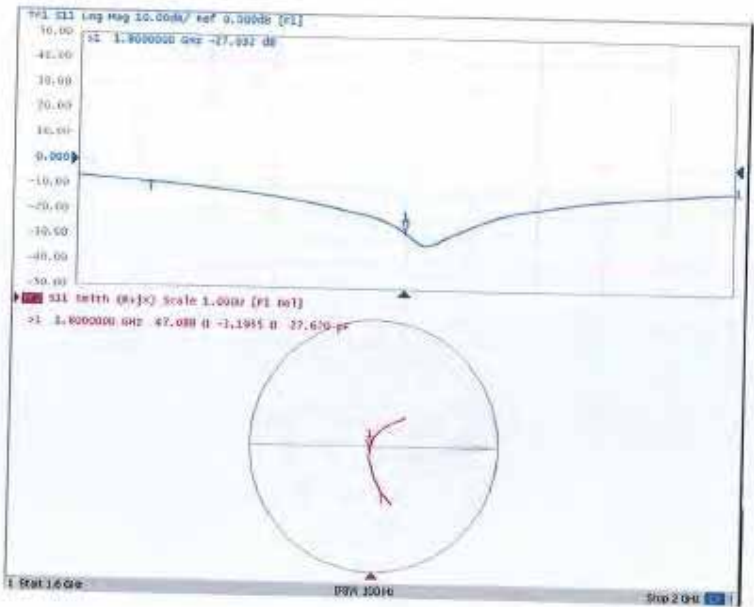
Impedance Measurement Plot for Head TSL
