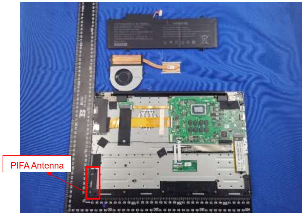
EUT UNCOVER VIEW
