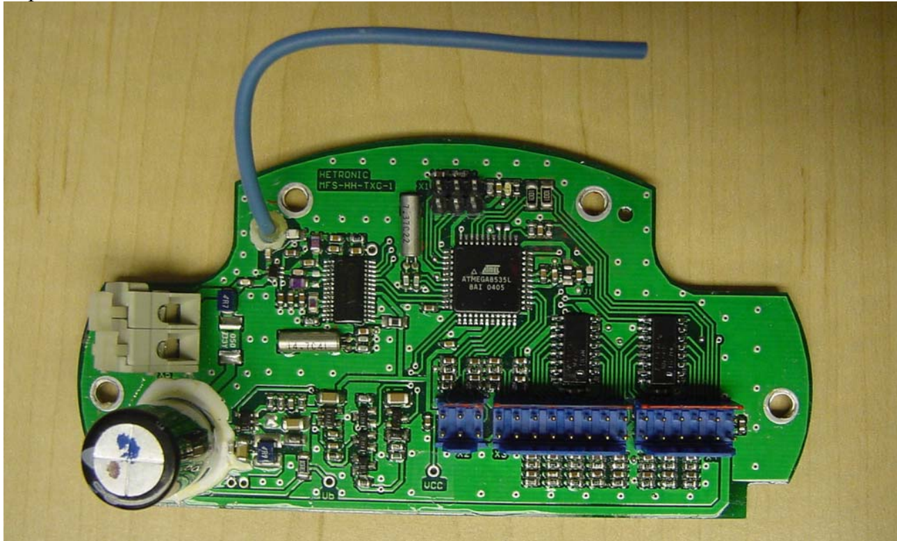
3. Coder board. Top view
