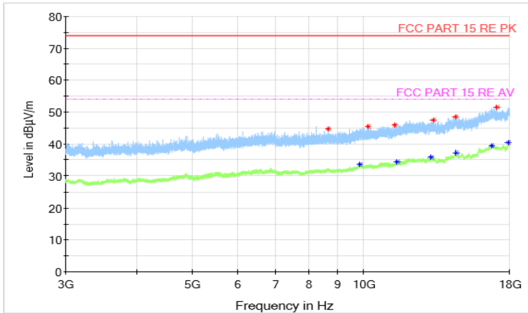
Figure A.1.21. Radiated Emission (Video Player, 3GHz to 18GHz)
