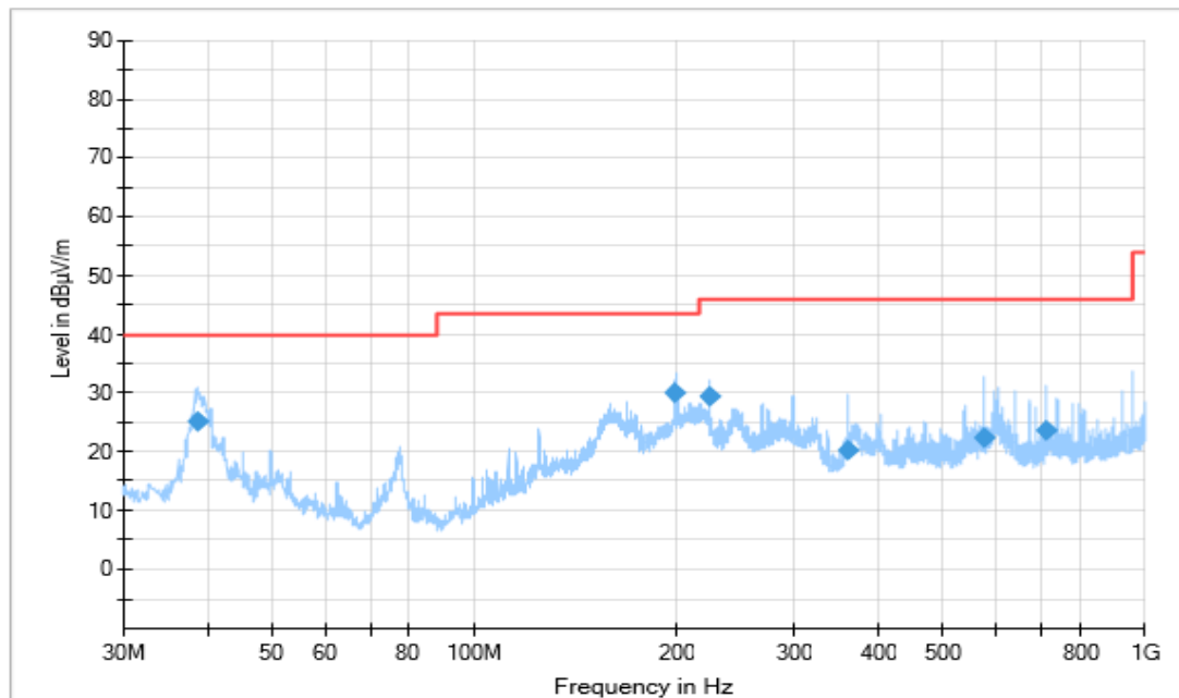
Figure A.1.22. Radiated Emission (Data Transfer : EUT to PC, 30MHz to 1GHz)
