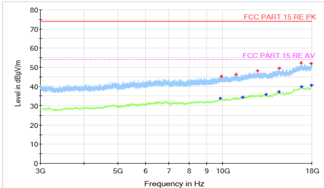
Figure A.1.36. Radiated Emission (Data Transfer : PC to TF Card, 3GHz to 18GHz) Final_Results_PK
