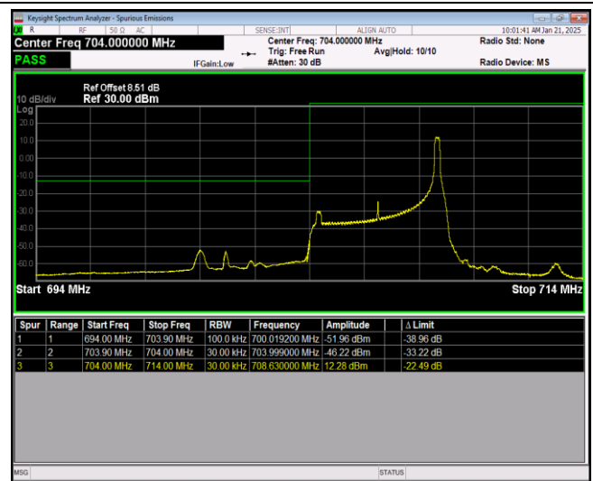
Band17-5MHz-16QAM-23825-1RB#0
