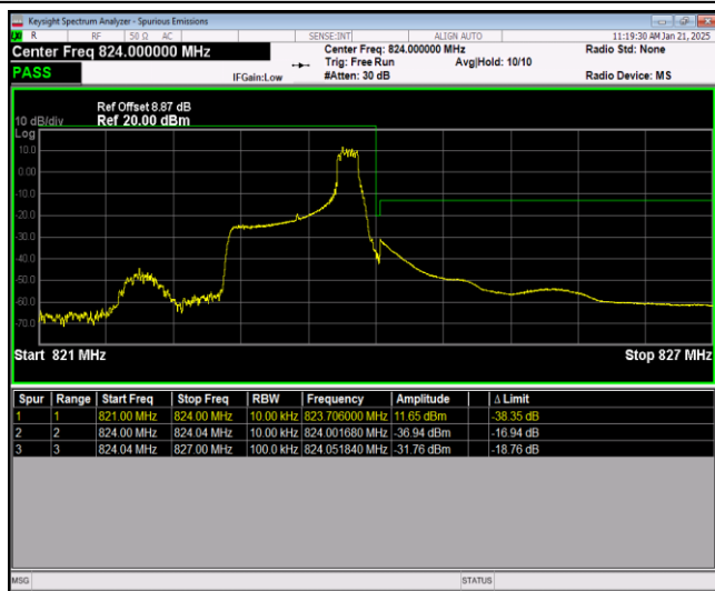
Band26-1.4MHz-64QAM-26797-1RB#0
