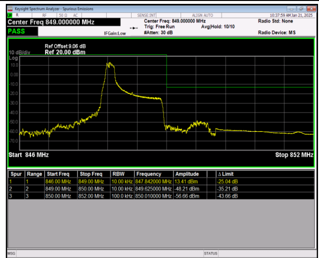
Band26-1.4MHz-QPSK-27033-6RB#0
