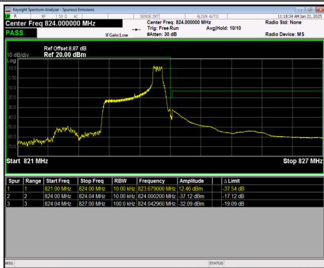
Band26-1.4MHz-QPSK-26797-1RB#0
