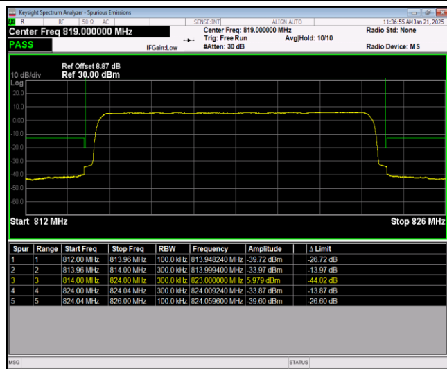
Band26-10MHz-16QAM-26740-1RB#49
