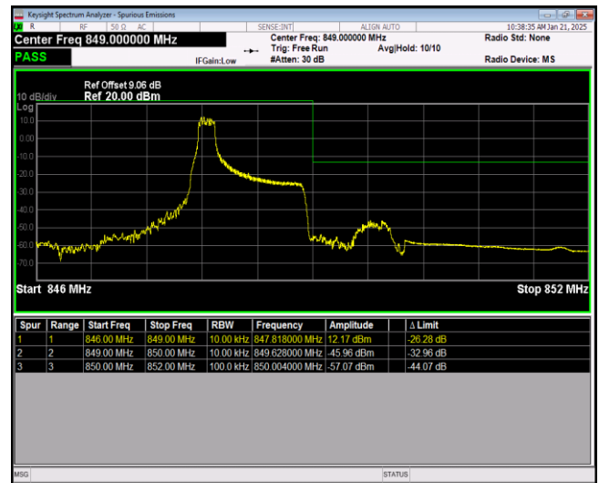
Band26-1.4MHz-64QAM-27033-6RB#0
