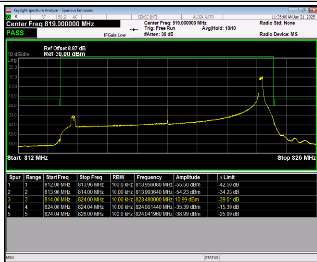
Band26-10MHz-64QAM-26740-1RB#0
