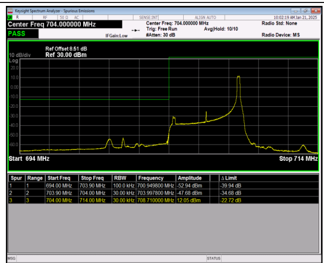
Band17-5MHz-64QAM-23825-1RB#0
