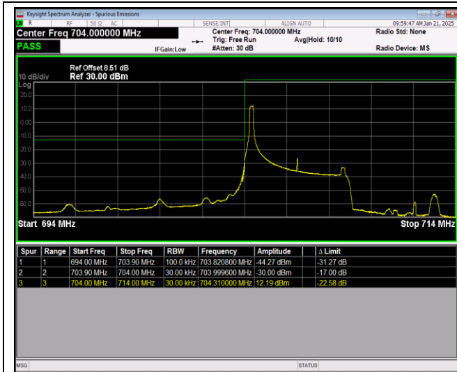
Band17-5MHz-16QAM-23755-25RB#0
