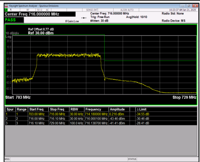
Band17-10MHz-64QAM-23780-1RB#49
