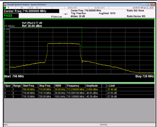
Band17-10MHz-QPSK-23780-1RB#49
