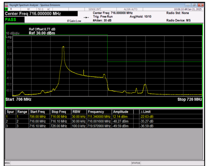
Band17-5MHz-64QAM-23825-25RB#0
