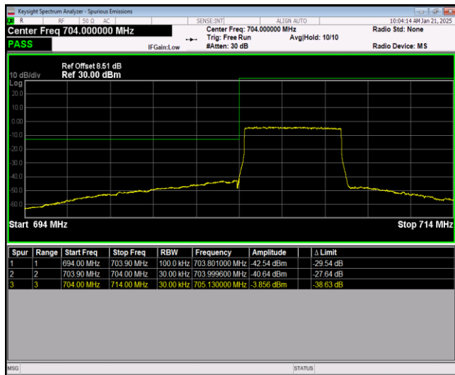
Band17-5MHz-64QAM-23825-1RB#24
