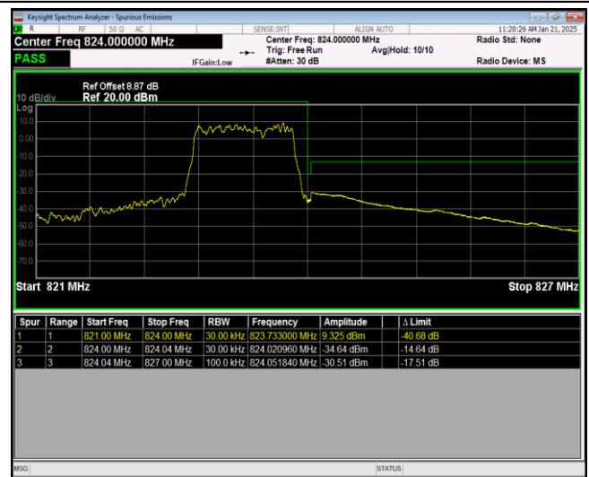
Band26-1.4MHz-16QAM-26797-1RB#5
