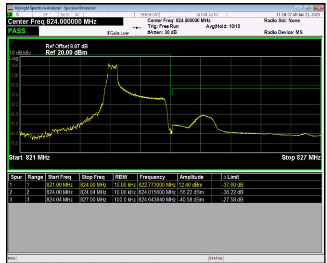
Band26-1.4MHz-64QAM-26783-6RB#0
