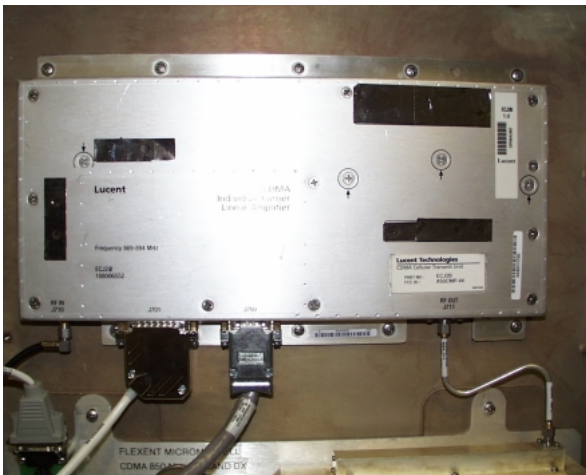
Photograph 1. ICLA installed in RFU cabinet
