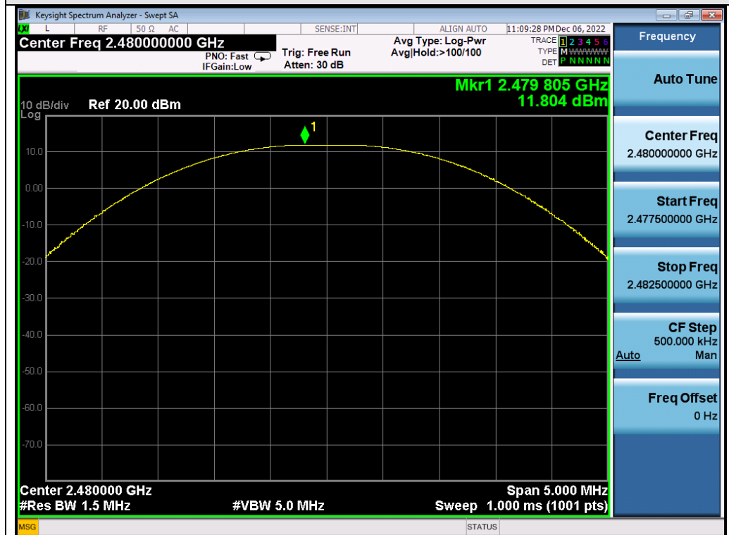
Test_Graph_2.4G_ANT2_2480_1Mbps_Peak Power
