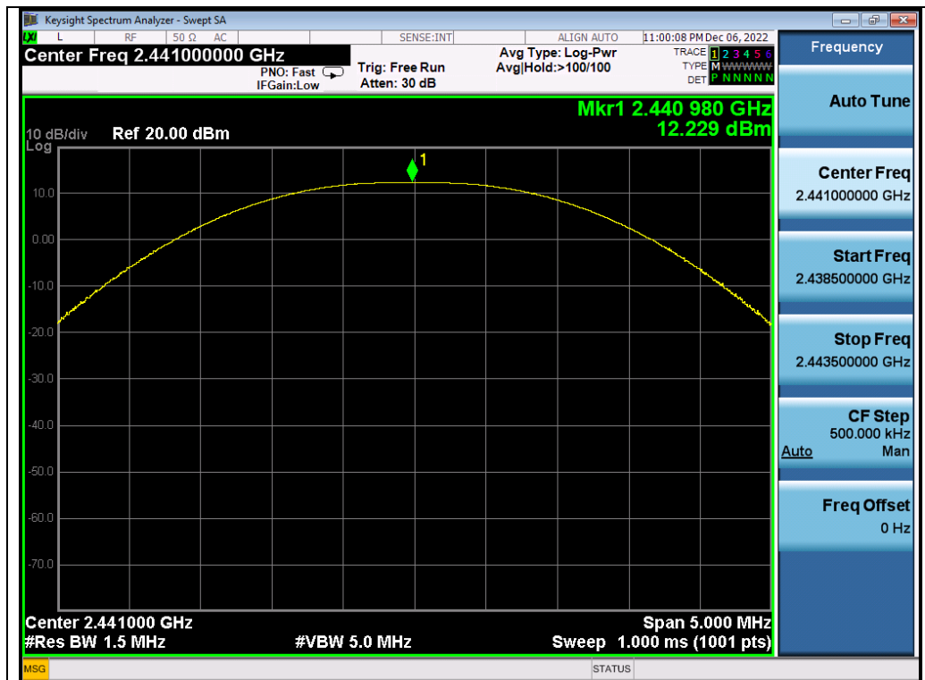
Test_Graph_2.4G_ANT2_2441_1Mbps_Peak Power
