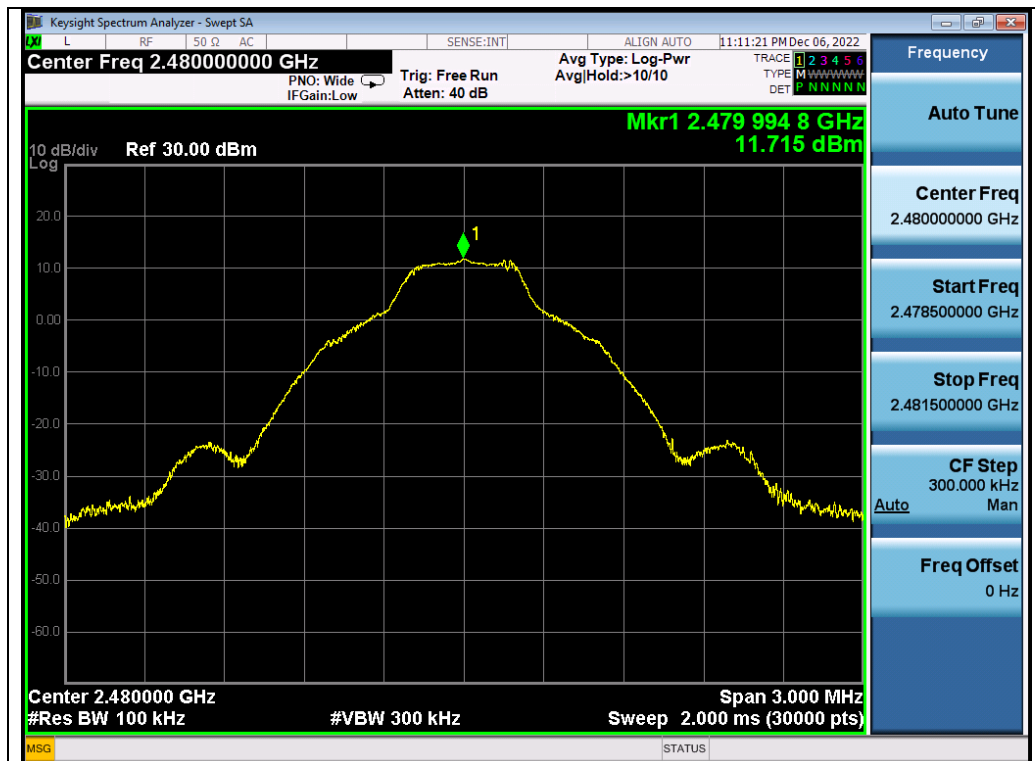
Test_Graph_2.4G_ANT2_2480_1Mbps_Reference Level
