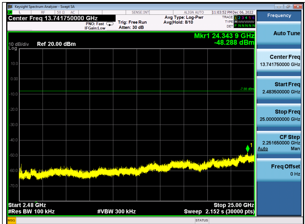
Test_Graph_2.4G_ANT2_2404_1Mbps_Higher Band Emissions
