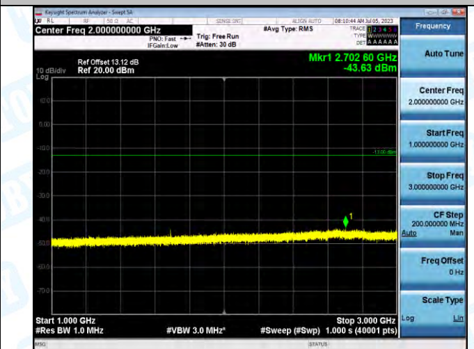
Band5_Band5_5MHz_QPSK_20625_1RB#0_1000~3000_1000~3000
