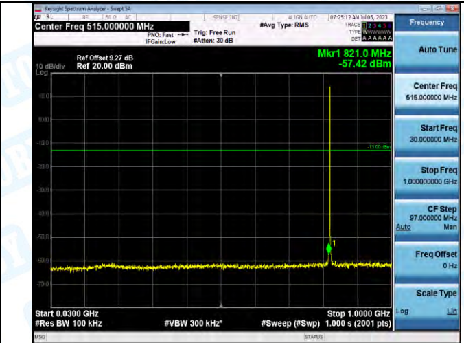
Band5_Band5_1.4MHz_16QAM_20407_1RB#0_30~1000_30~1000
