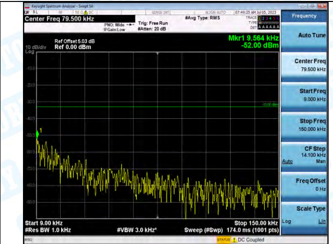
Band5_Band5_3MHz_16QAM_20635_1RB#0_0.009~0.15_0.009~0.15
