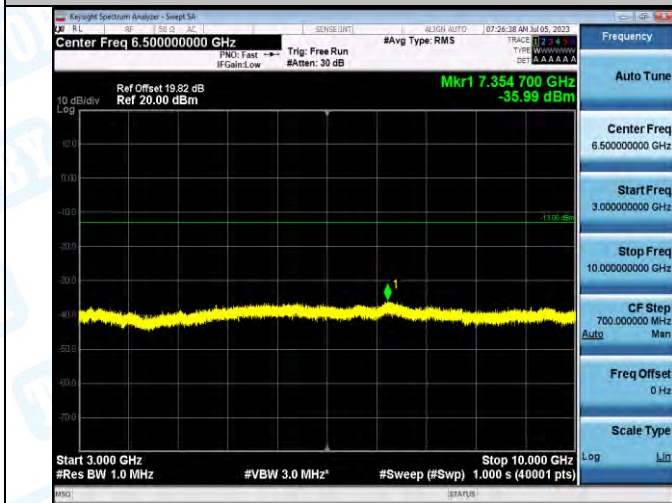
Band5_Band5_1.4MHz_QPSK_20525_1RB#0_3000~10000_3000~10000
