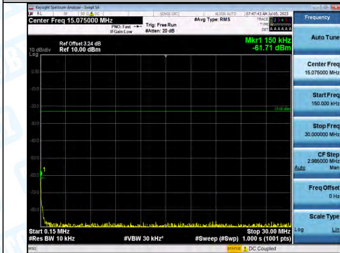
Band5_Band5_3MHz_16QAM_20525_1RB#0_0.15~30_0.15~30
