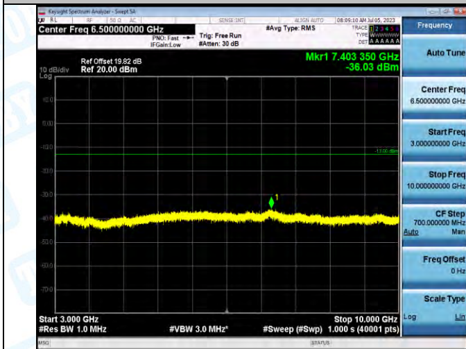
Band5_Band5_5MHz_QPSK_20525_1RB#0_3000~10000_3000~10000
