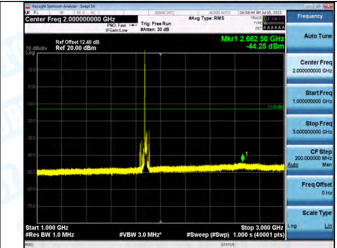
Band2_Band2_20MHz_QPSK_18900_1RB#0_1000~3000_1000~3000
