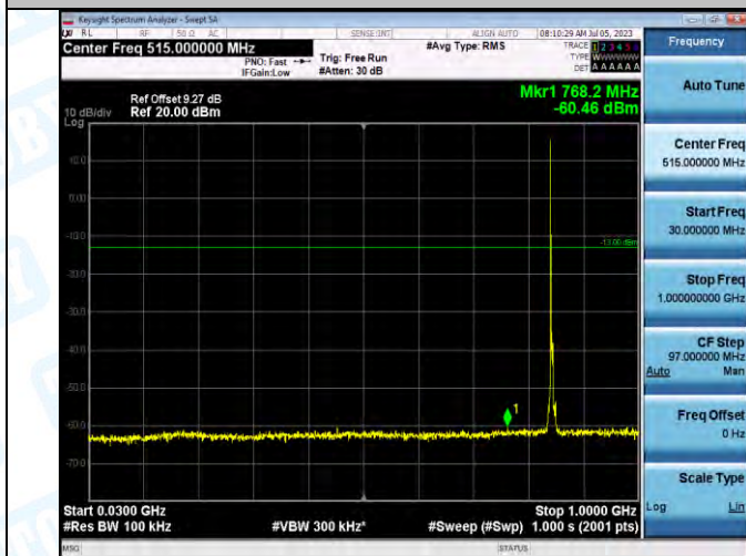
Band5_Band5_5MHz_QPSK_20625_1RB#0_30~1000_30~1000
