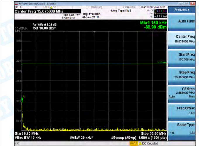
Band5_Band5_3MHz_QPSK_20415_1RB#0_0.15~30_0.15~30
