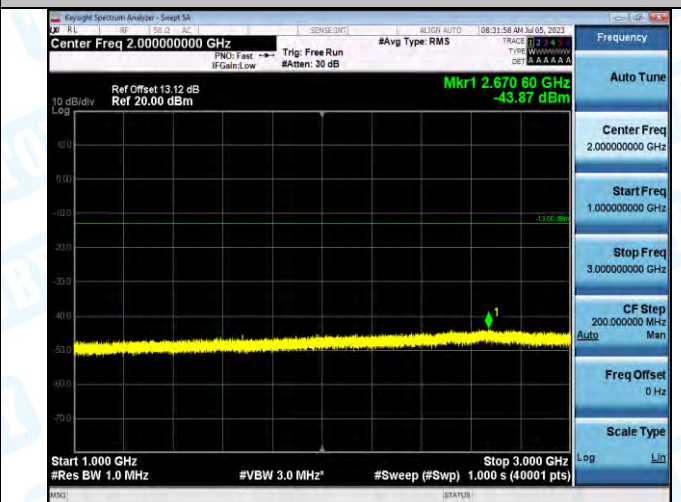
Band5_Band5_10MHz_QPSK_20600_1RB#0_1000~3000_1000~3000
