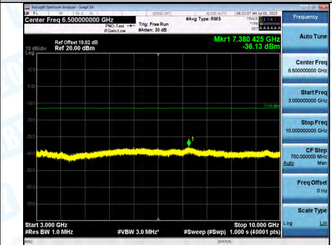
Band5_Band5_10MHz_16QAM_20600_1RB#0_3000~10000_3000~10000
