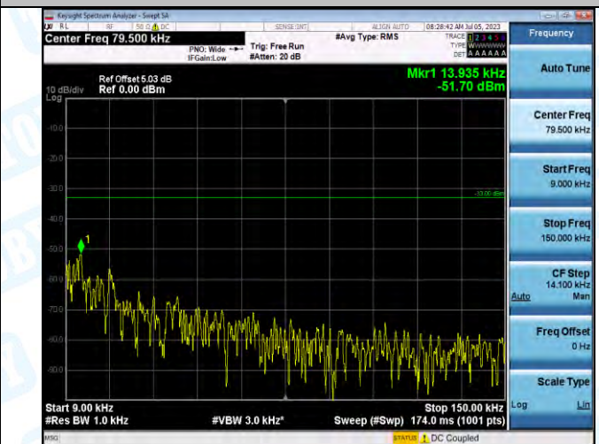
Band5_Band5_10MHz_16QAM_20450_1RB#0_0.009~0.15_0.009~0.15
