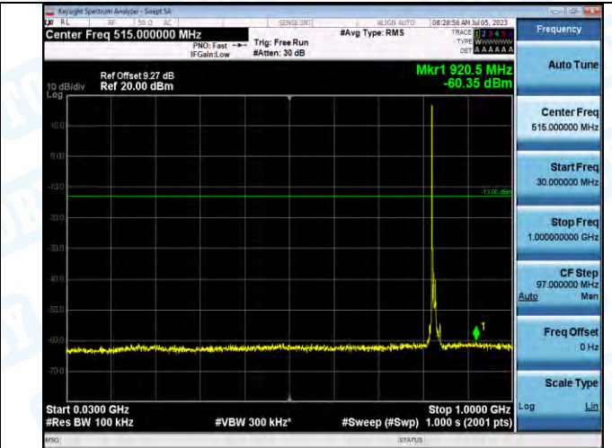
Band5_Band5_10MHz_16QAM_20450_1RB#0_30~1000_30~1000
