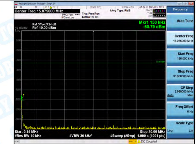
Band5_Band5_1.4MHz_QPSK_20407_1RB#0_0.15~30_0.15~30
