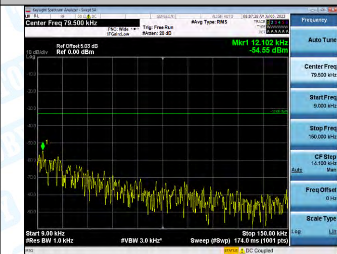
Band5 Band5 5MHz 16QAM 20425 1RB#0 0.009~0.15 0.009~0.15
