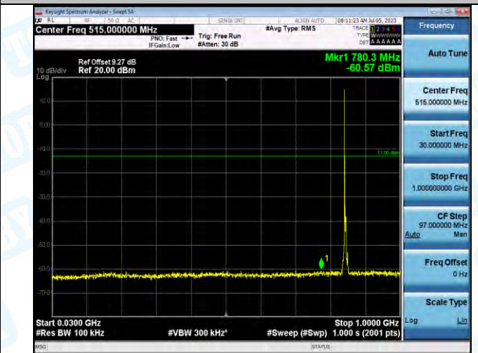
Band5_Band5_5MHz_16QAM_20625_1RB#0_30~1000_30~1000
