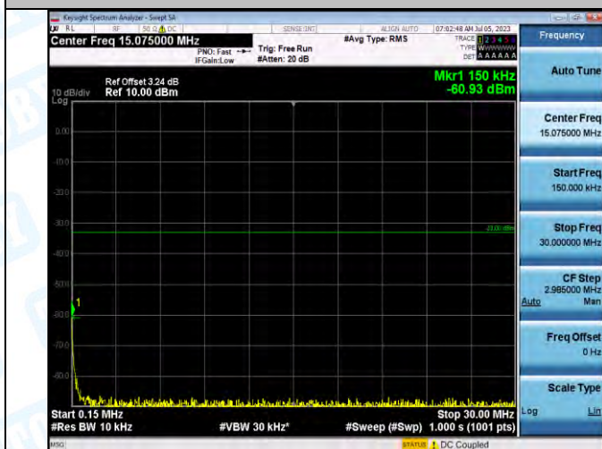
Band2_Band2_20MHz_16QAM_18900_1RB#0_0.15~30_0.15~30
