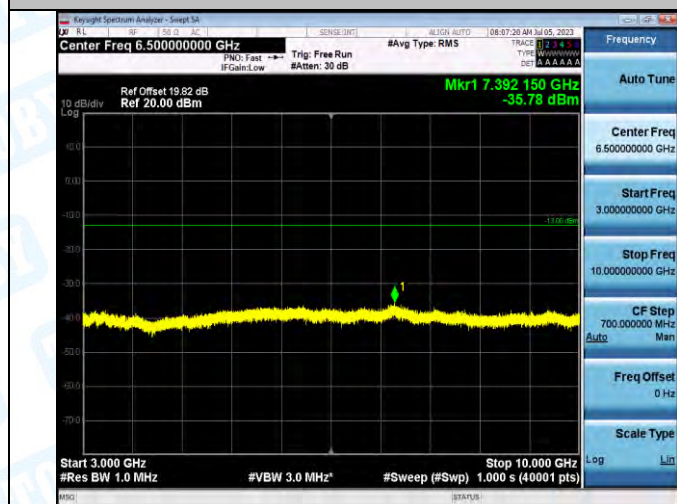
Band5 Band5 5MHz QPSK 20425 1RB#0 3000~10000 3000~10000
