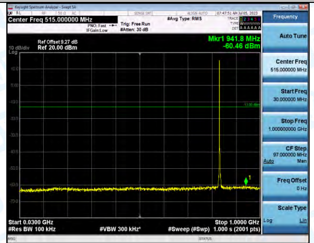
Band5_Band5_3MHz_16QAM_20525_1RB#0_30~1000_30~1000
