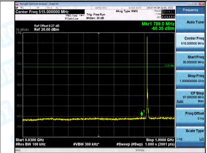
Band5_Band5_5MHz_16QAM_20425_1RB#0_30~1000_30~1000
