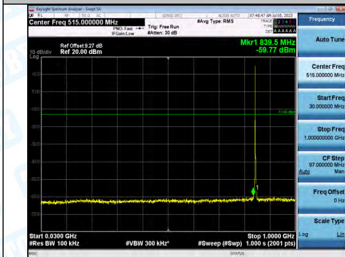
Band5_Band5_3MHz_QPSK_20635_1RB#0_30~1000_30~1000
