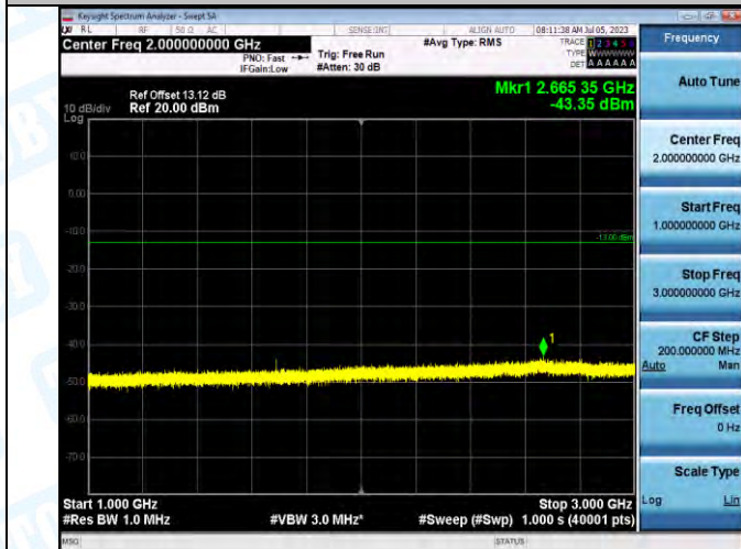
Band5_Band5_5MHz_16QAM_20625_1RB#0_1000~3000_1000~3000
