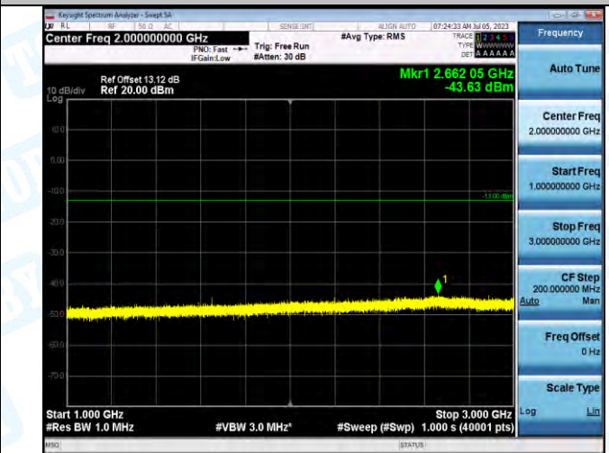
Band5_Band5_1.4MHz_QPSK_20407_1RB#0_1000~3000_1000~3000
