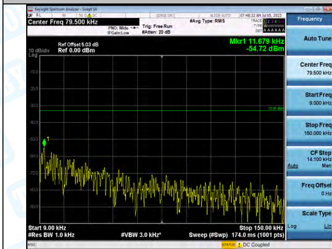
Band5_Band5_3MHz_QPSK_20635_1RB#0_0.009~0.15_0.009~0.15
