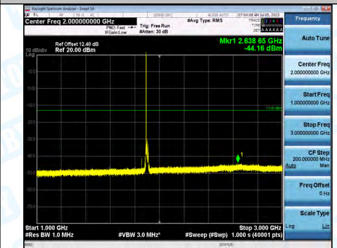
Band2_Band2_20MHz_QPSK_19100_1RB#0_1000~3000_1000~3000
