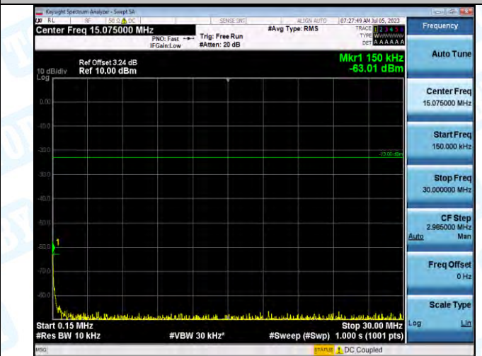
Band5_Band5_1.4MHz_QPSK_20643_1RB#0_0.15~30_0.15~30
