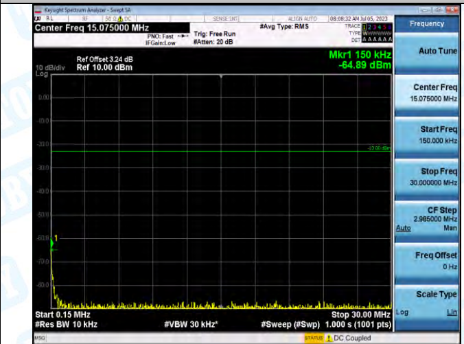
Band5_Band5_5MHz_QPSK_20525_1RB#0_0.15~30_0.15~30
