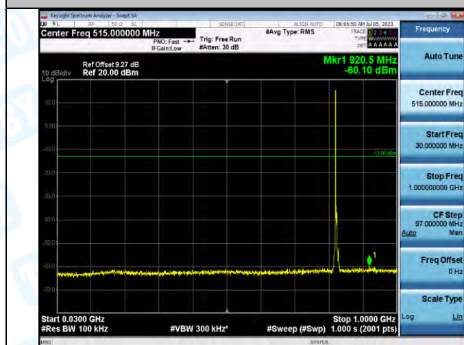
Band5 Band5 5MHz QPSK 20425 1RB#0 30~1000 30~1000
