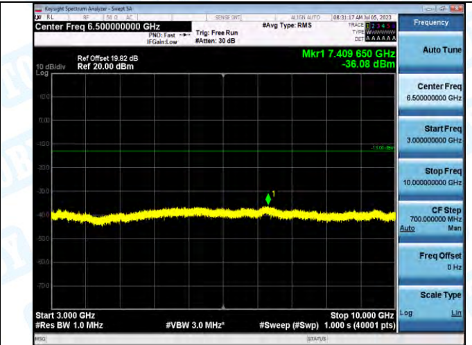
Band5_Band5_10MHz_16QAM_20525_1RB#0_3000~10000_3000~10000
