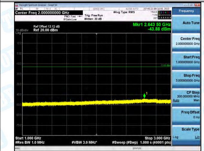
Band5_Band5_3MHz_QPSK_20415_1RB#0_1000~3000_1000~3000
