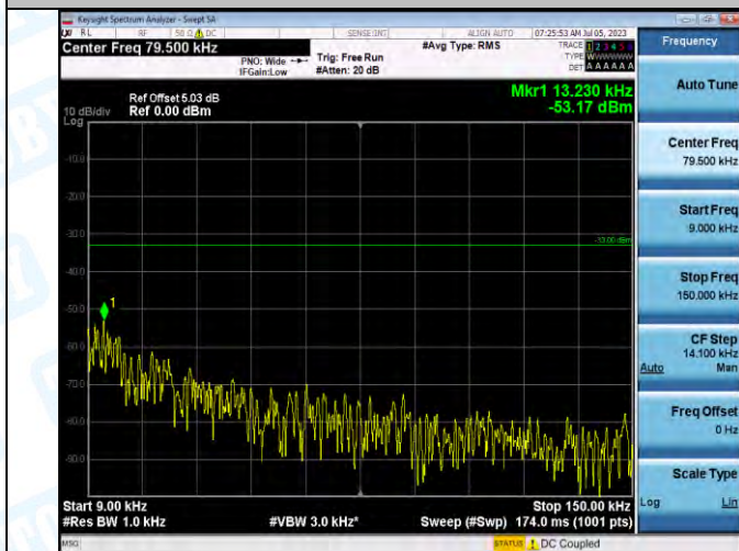
Band5_Band5_1.4MHz_QPSK_20525_1RB#0_0.009~0.15_0.009~0.15
