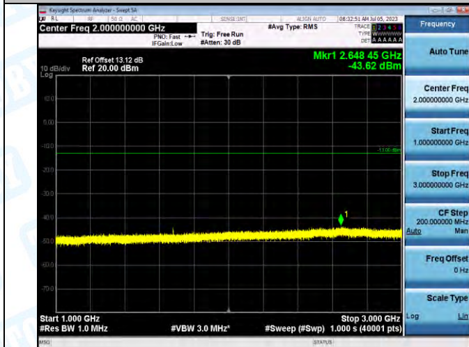
Band5_Band5_10MHz_16QAM_20600_1RB#0_1000~3000_1000~3000
