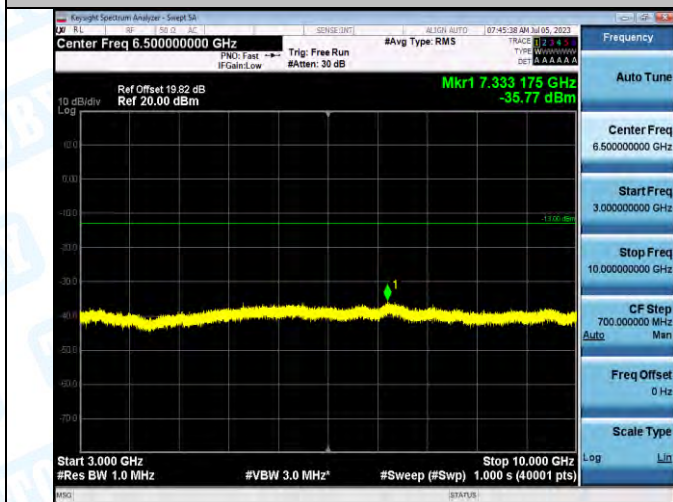
Band5_Band5_3MHz_QPSK_20415_1RB#0_3000~10000_3000~10000
