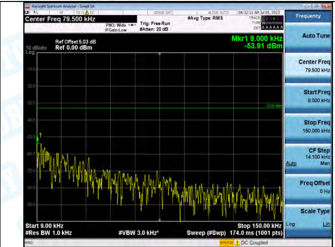
Band5_Band5_10MHz_16QAM_20600_1RB#0_0.009~0.15_0.009~0.15
