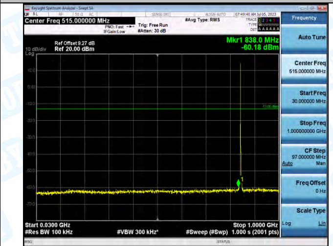
Band5_Band5_3MHz_16QAM_20635_1RB#0_30~1000_30~1000
