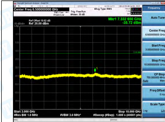
Band5_Band5_5MHz_QPSK_20625_1RB#0_3000~10000_3000~10000
