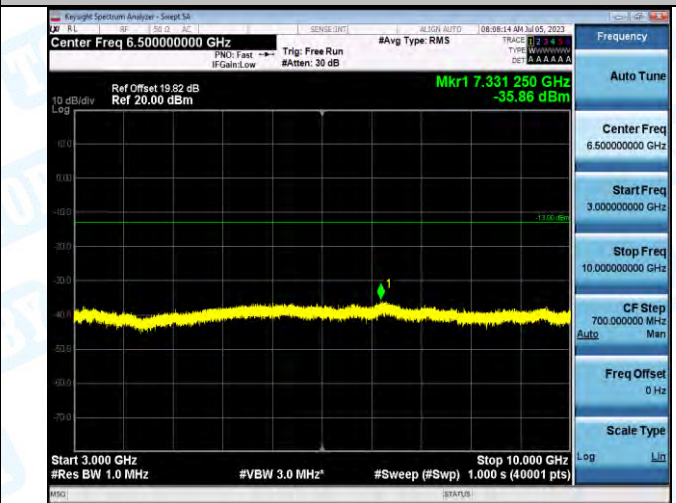
Band5_Band5_5MHz_16QAM_20425_1RB#0_3000~10000_3000~10000
