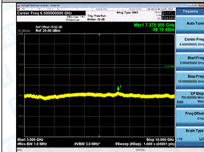
Band5_Band5_10MHz_QPSK_20450_1RB#0_3000~10000_3000~10000
