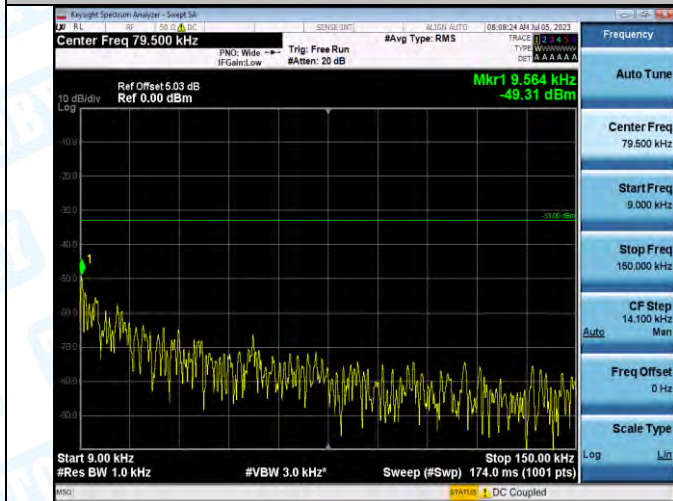
Band5_Band5_5MHz_QPSK_20525_1RB#0_0.009~0.15_0.009~0.15
