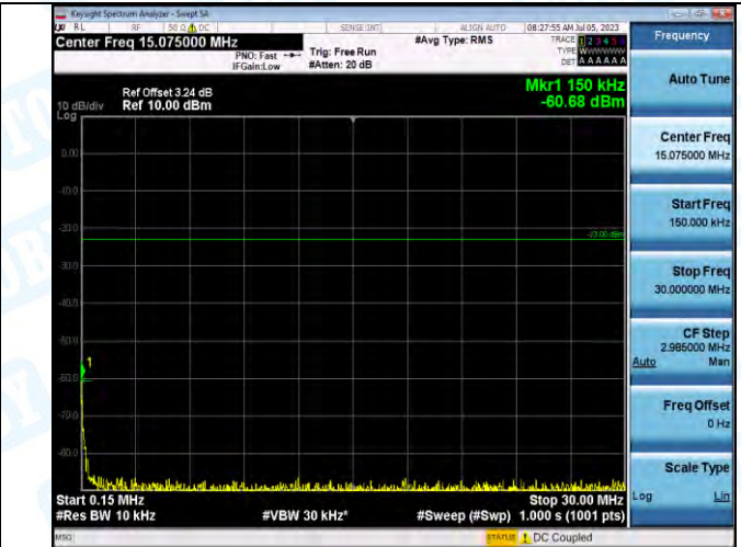
Band5_Band5_10MHz_QPSK_20450_1RB#0_0.15~30_0.15~30
