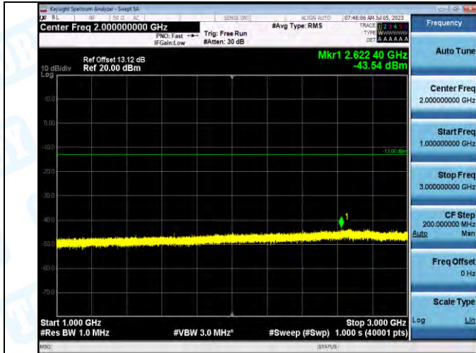
Band5_Band5_3MHz_16QAM_20525_1RB#0_1000~3000_1000~3000
