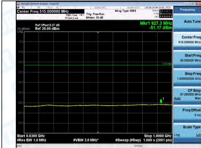
Band2_Band2_20MHz_QPSK_18900_1RB#0_30~1000_30~1000
