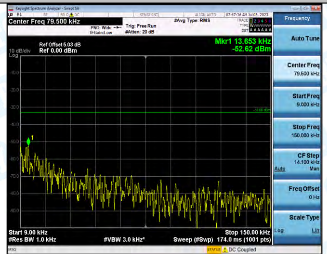
Band5_Band5_3MHz_16QAM_20525_1RB#0_0.009~0.15_0.009~0.15
