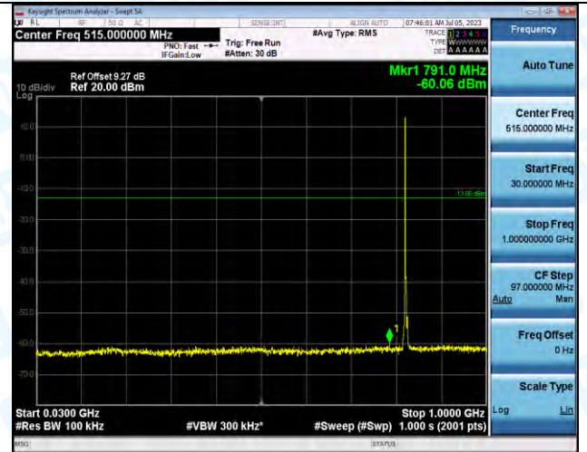
Band5_Band5_3MHz_16QAM_20415_1RB#0_30~1000_30~1000
