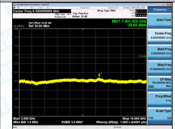
Band5_Band5_3MHz_16QAM_20635_1RB#0_3000~10000_3000~10000
