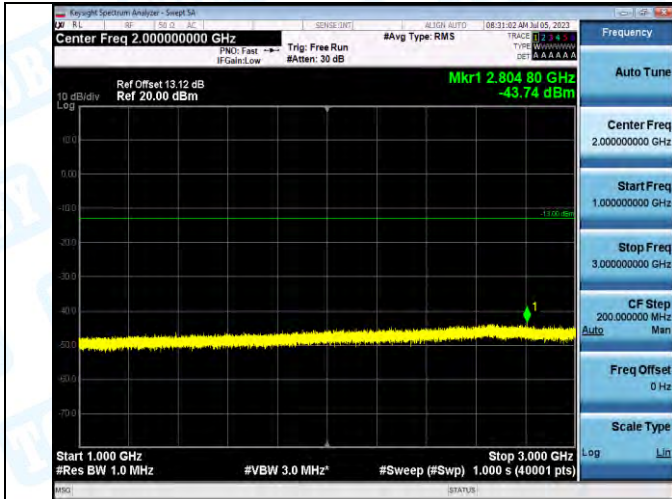
Band5_Band5_10MHz_16QAM_20525_1RB#0_1000~3000_1000~3000
