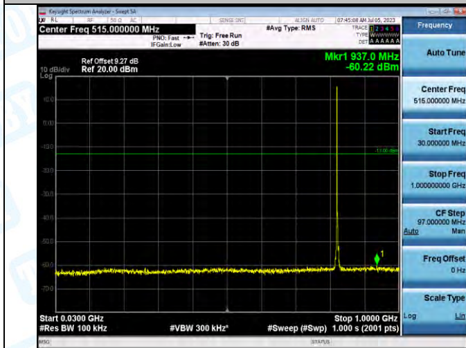
Band5_Band5_3MHz_QPSK_20415_1RB#0_30~1000_30~1000
