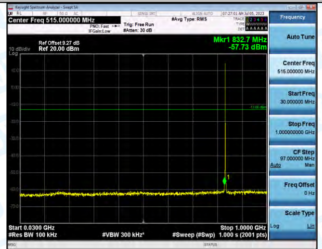
Band5_Band5_1.4MHz_16QAM_20525_1RB#0_30~1000_30~1000
