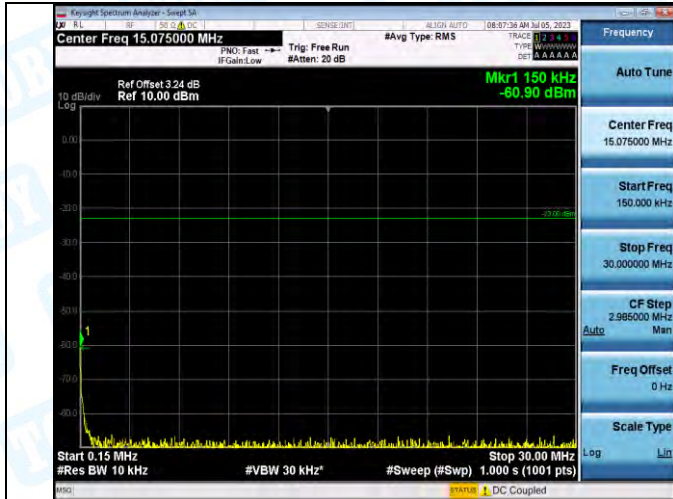
Band5_Band5_5MHz_16QAM_20425_1RB#0_0.15~30_0.15~30
