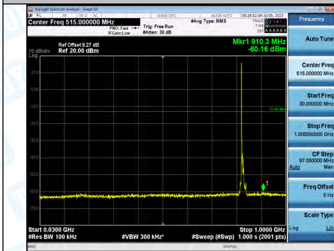
Band5_Band5_10MHz_QPSK_20450_1RB#0_30~1000_30~1000
