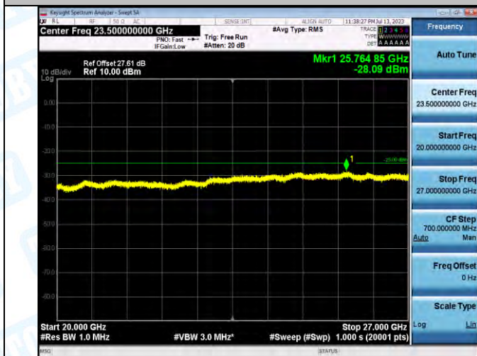
Band7_Band7_5MHz_QPSK_20775_1RB#0_20000-27000_20000-27000
