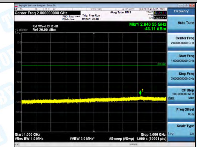
Band5_Band5_10MHz_QPSK_20450_1RB#0_1000~3000_1000~3000
