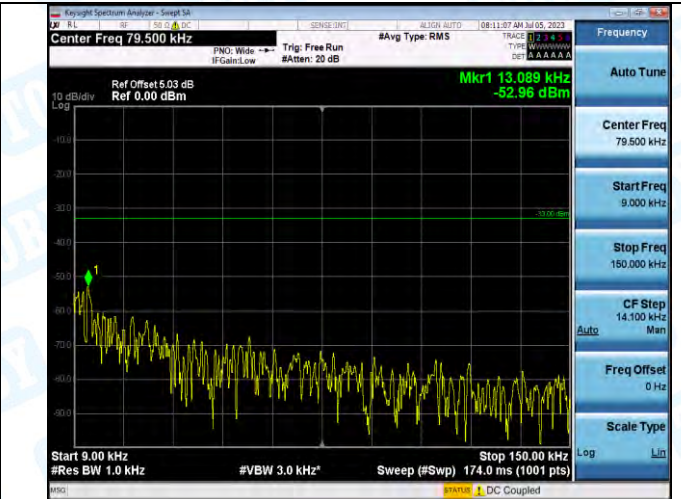
Band5_Band5_5MHz_16QAM_20625_1RB#0_0.009~0.15_0.009~0.15
