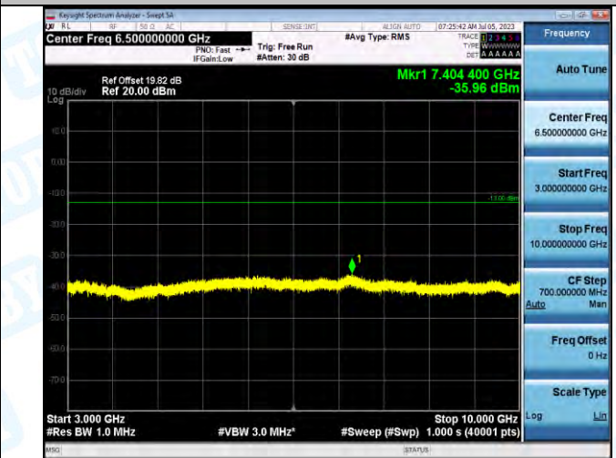
Band5_Band5_1.4MHz_16QAM_20407_1RB#0_3000~10000_3000~10000
