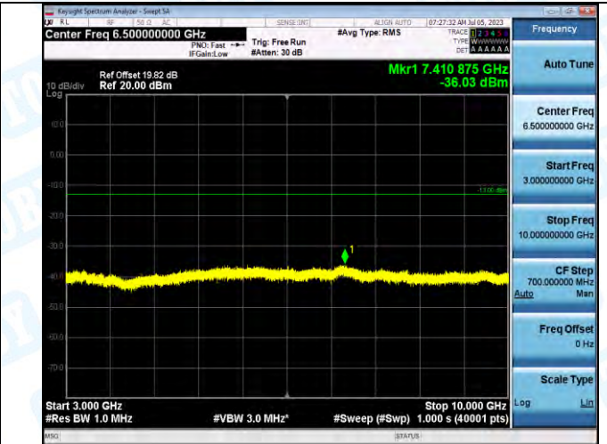
Band5_Band5_1.4MHz_16QAM_20525_1RB#0_3000~10000_3000~10000
