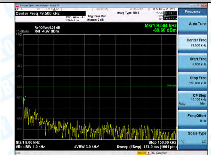
Band7_Band7_5MHz_16QAM_20775_1RB#0_0.009-0.15_0.009-0.15
