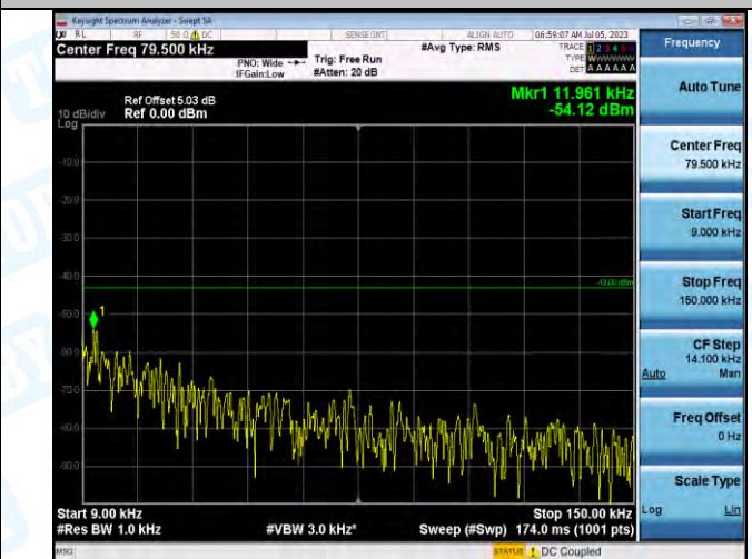
Band2_Band2_20MHz_16QAM_18900_1RB#0_0.009~0.15_0.009~0.15
