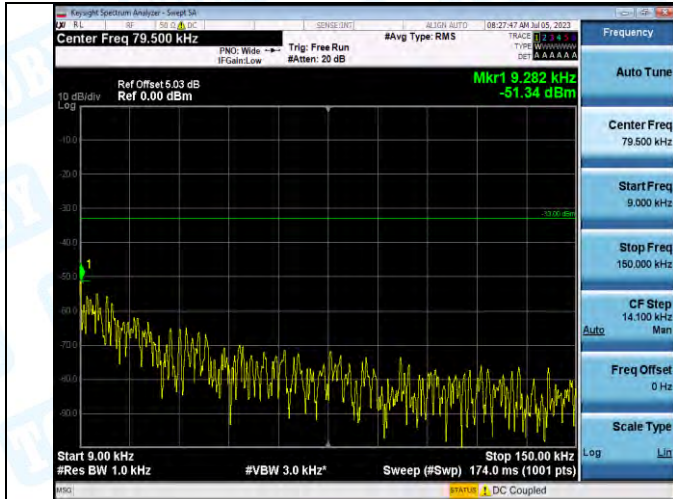
Band5_Band5_10MHz_QPSK_20450_1RB#0_0.009~0.15_0.009~0.15
