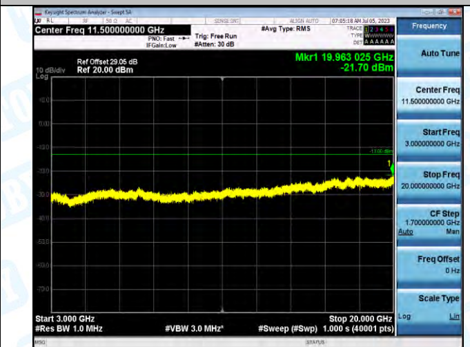
Band2_Band2_20MHz_16QAM_19100_1RB#0_3000~20000_3000~20000
