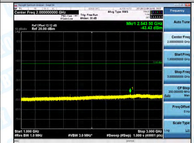
Band5_Band5_1.4MHz_QPSK_20643_1RB#0_1000~3000_1000~3000
