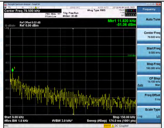
Band5_Band5_1.4MHz_16QAM_20525_1RB#0_0.009~0.15_0.009~0.15
