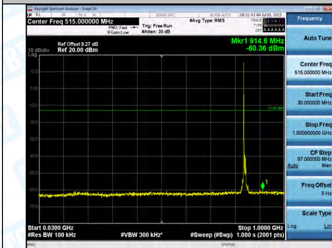
Band5_Band5_10MHz_QPSK_20600_1RB#0_30~1000_30~1000
