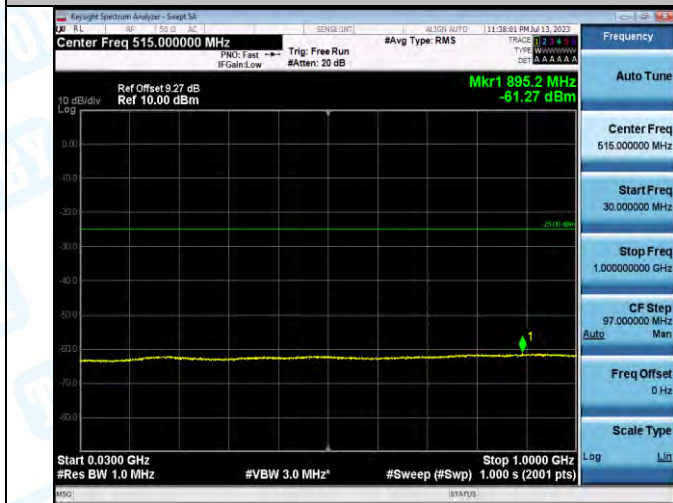
Band7_Band7_5MHz_QPSK_20775_1RB#0_30-1000_30-1000
