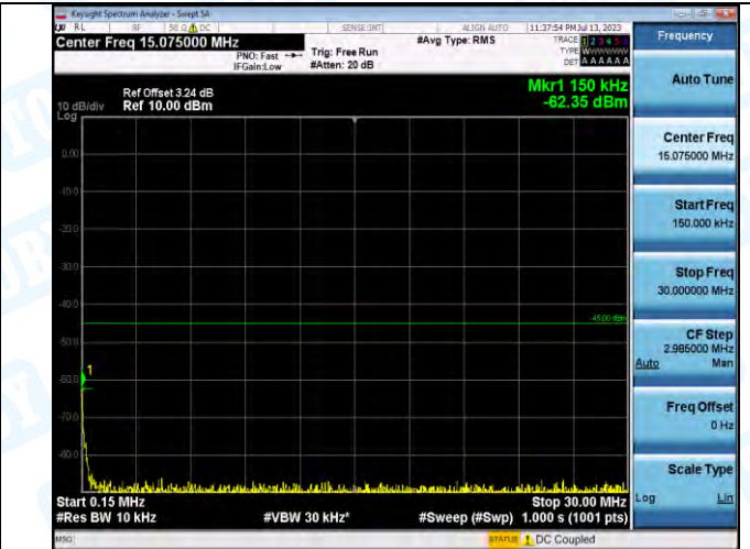
Band7_Band7_5MHz_QPSK_20775_1RB#0_0.15-30_0.15-30
