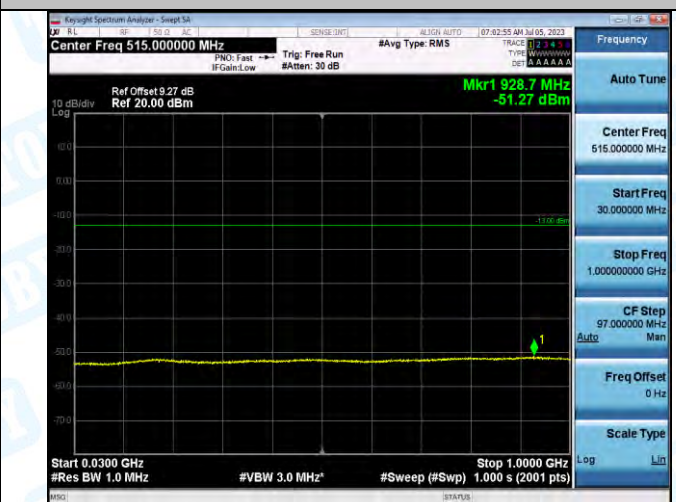
Band2_Band2_20MHz_16QAM_18900_1RB#0_30~1000_30~1000
