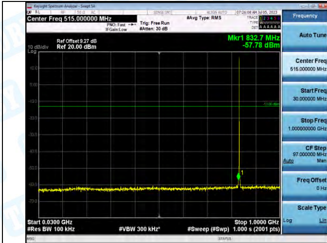
Band5_Band5_1.4MHz_QPSK_20525_1RB#0_30~1000_30~1000
