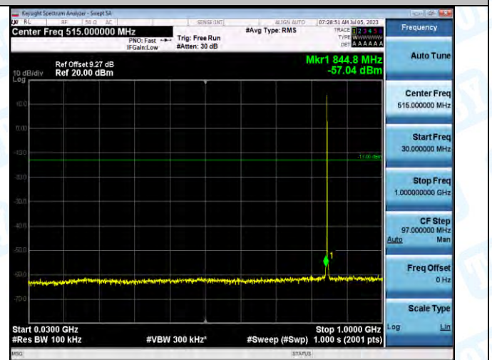
Band5_Band5_1.4MHz_16QAM_20643_1RB#0_30~1000_30~1000
