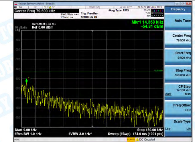
Band2_Band2_20MHz_16QAM_19100_1RB#0_0.009~0.15_0.009~0.15
