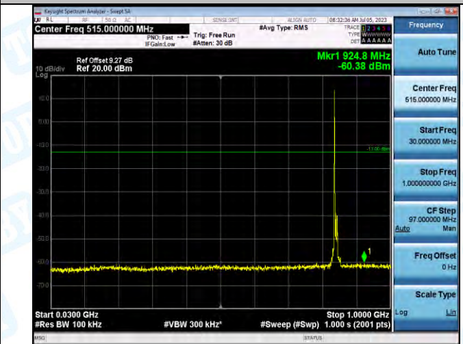
Band5_Band5_10MHz_16QAM_20600_1RB#0_30~1000_30~1000
