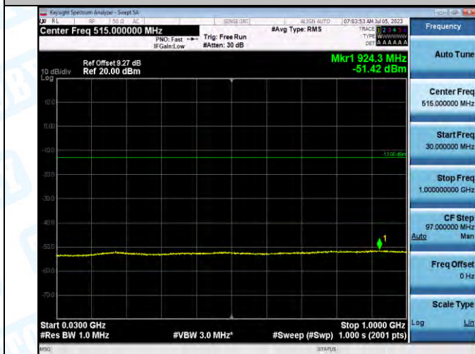
Band2_Band2_20MHz_QPSK_19100_1RB#0_30~1000_30~1000
