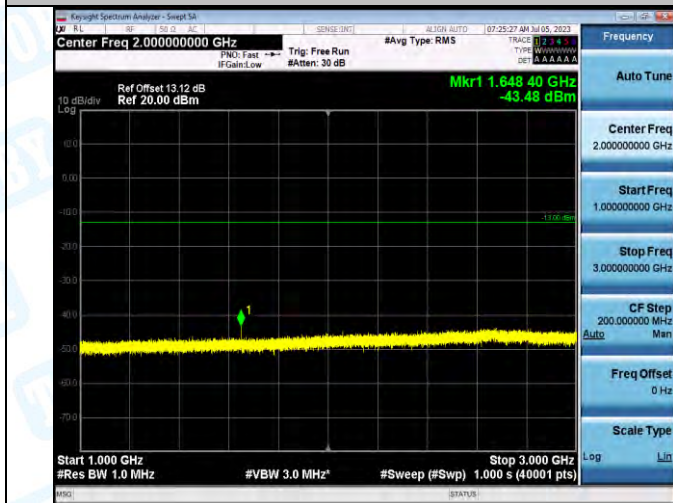
Band5_Band5_1.4MHz_16QAM_20407_1RB#0_1000~3000_1000~3000
