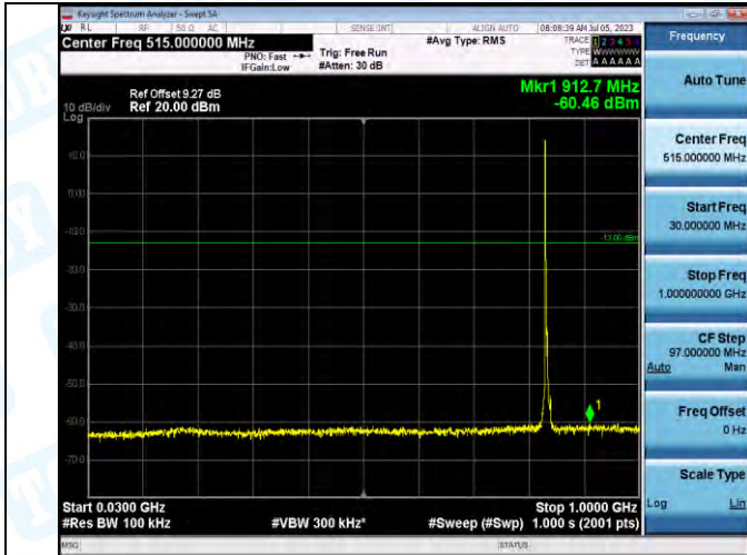
Band5_Band5_5MHz_QPSK_20525_1RB#0_30~1000_30~1000
