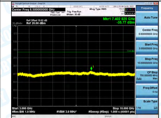
Band5_Band5_5MHz_16QAM_20625_1RB#0_3000~10000_3000~10000
