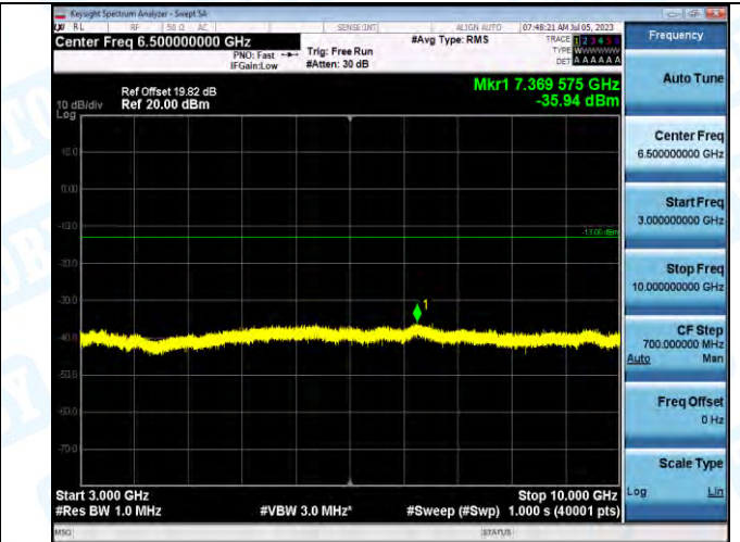
Band5_Band5_3MHz_16QAM_20525_1RB#0_3000~10000_3000~10000
