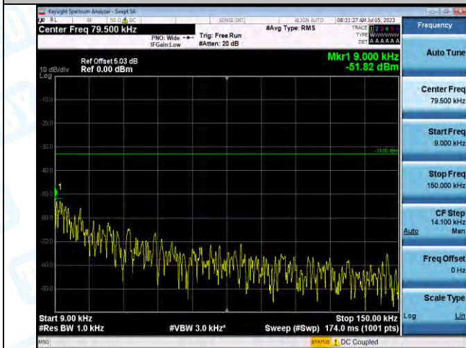
Band5_Band5_10MHz_QPSK_20600_1RB#0_0.009~0.15_0.009~0.15
