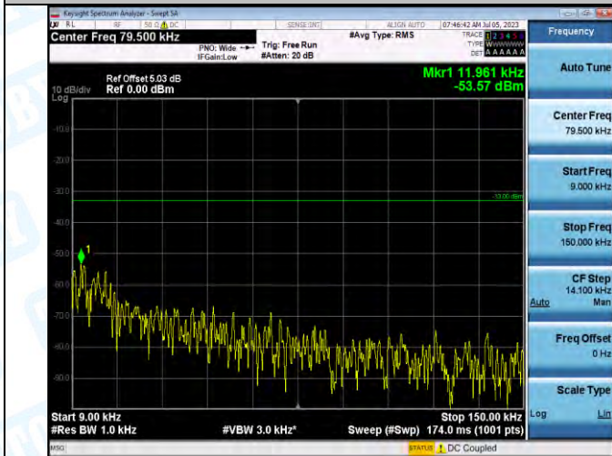
Band5_Band5_3MHz_QPSK_20525_1RB#0_0.009~0.15_0.009~0.15
