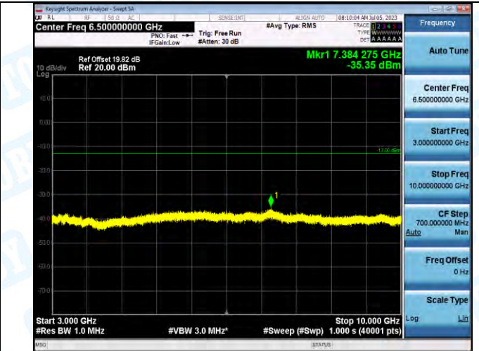
Band5_Band5_5MHz_16QAM_20525_1RB#0_3000~10000_3000~10000
