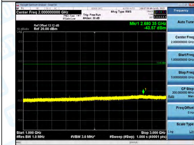
Band5_Band5_5MHz_16QAM_20425_1RB#0_1000~3000_1000~3000
