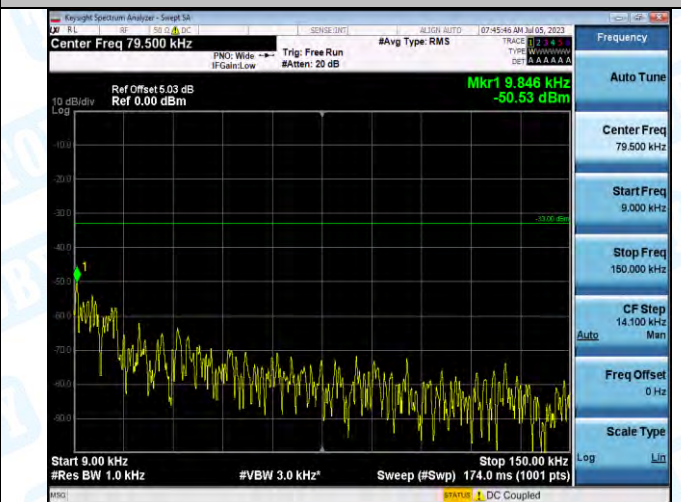
Band5_Band5_3MHz_16QAM_20415_1RB#0_0.009~0.15_0.009~0.15
