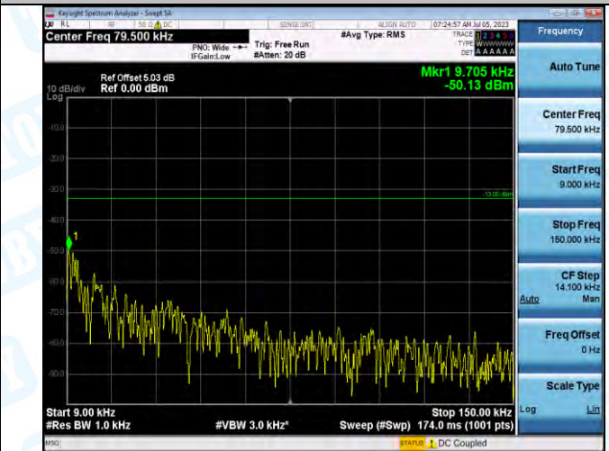
Band5_Band5_1.4MHz_16QAM_20407_1RB#0_0.009~0.15_0.009~0.15
