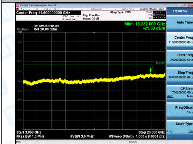
Band2_Band2_20MHz_QPSK_18900_1RB#0_3000~20000_3000~20000
