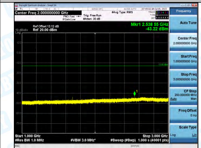
Band5_Band5_3MHz_QPSK_20635_1RB#0_1000~3000_1000~3000
