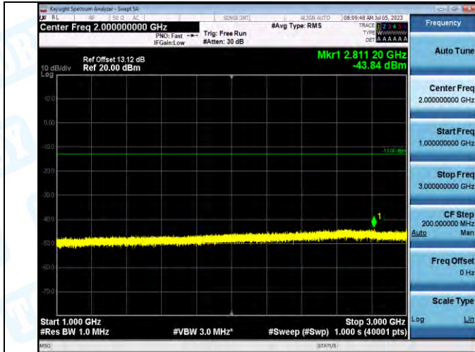
Band5_Band5_5MHz_16QAM_20525_1RB#0_1000~3000_1000~3000
