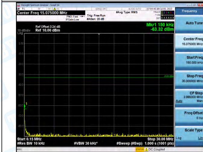
Band2_Band2_20MHz_16QAM_19100_1RB#0_0.15~30_0.15~30
