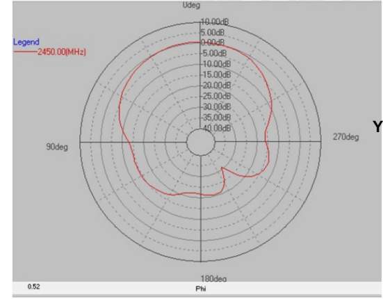
X-Y Plane (E-total)
