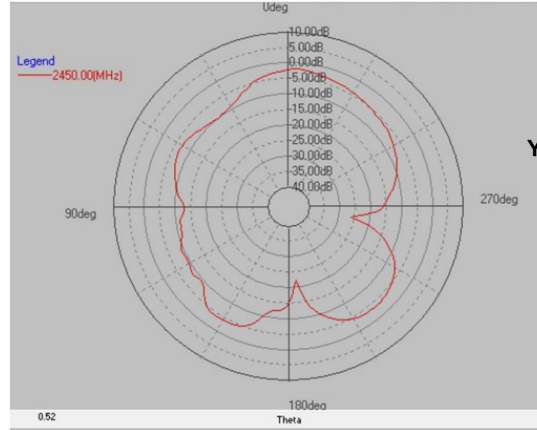
Y-Z Plane (E-total)
