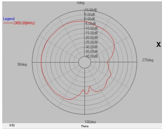
X-Z Plane (E-total)
