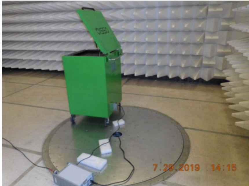
Test setup
