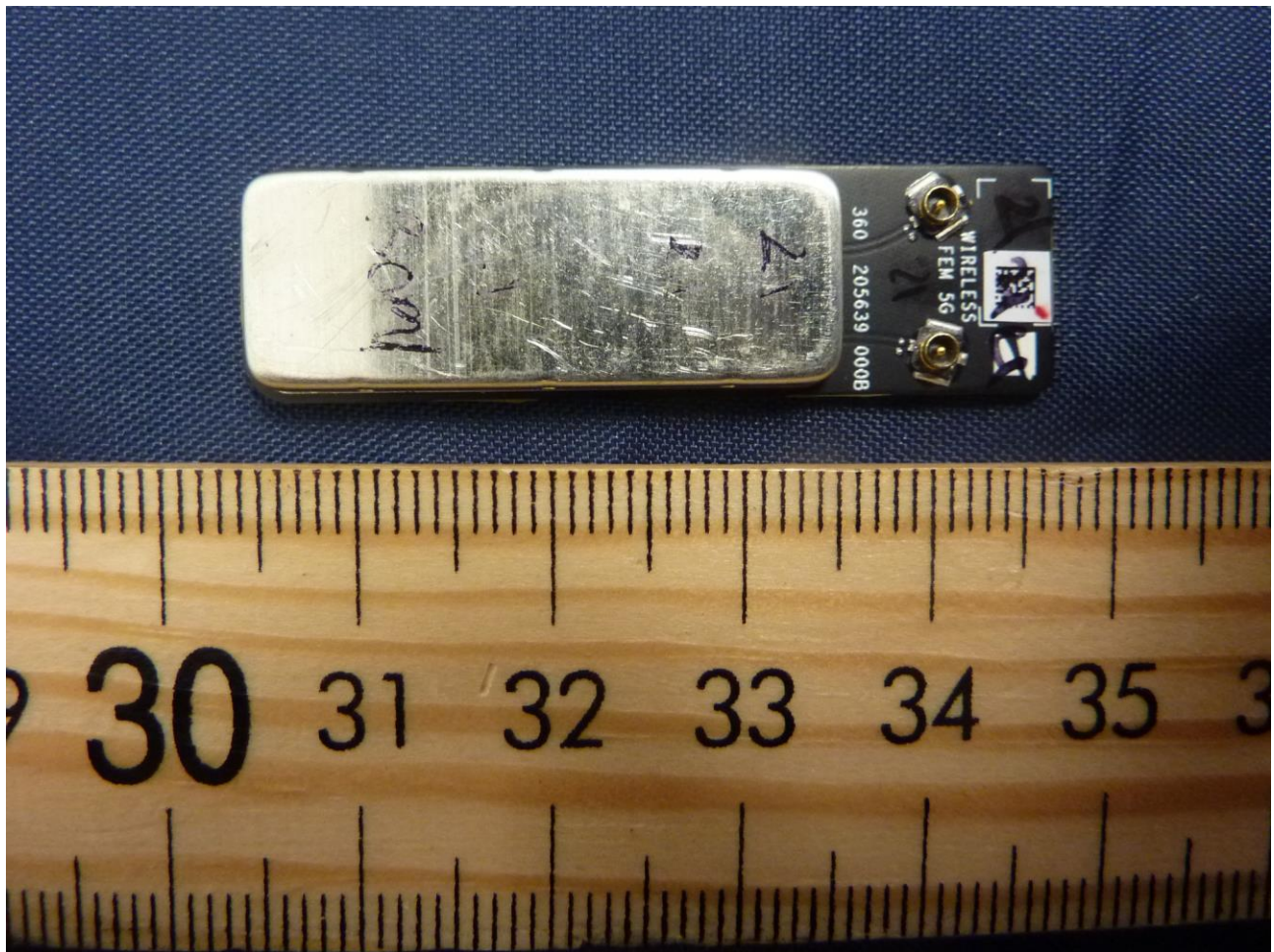
Figure 1 - External Photo of EUT- Front View
