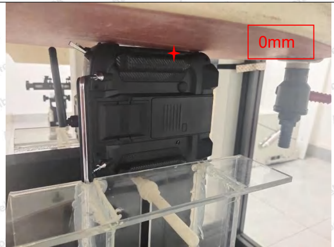
Right(0mm) Antenna bends 90 degrees
