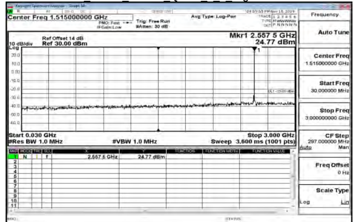
30MHz~3GHz Band7 15MHz QPSK 1 0 HighCH21375-2562.5
