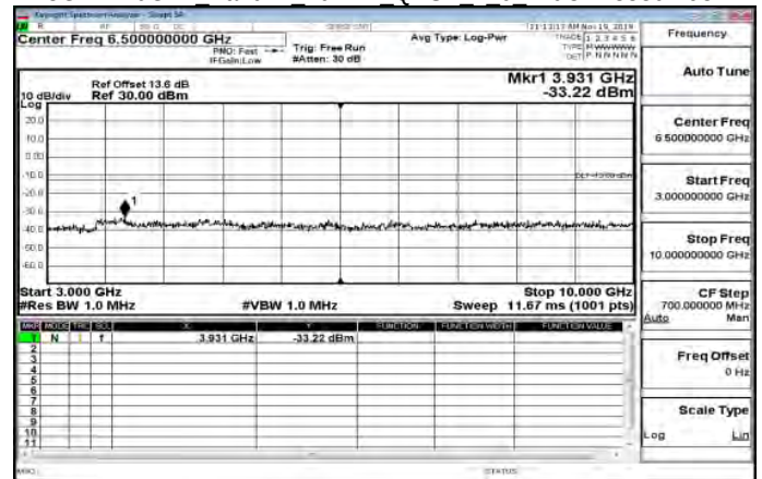
3GHz~10GHz Band14 10MHz QPSK 1 0 MidCH23330-793
