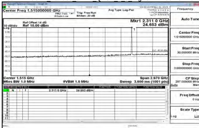
30MHz~3GHz Band30 5MHz QPSK 1 0 HighCH27735-2312.5
