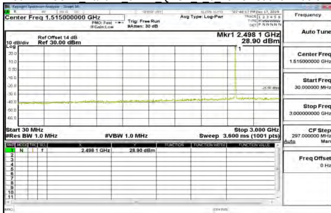
30MHz~3GHz Band41 5MHz QPSK 1 0 LowCH39675-2498.5
