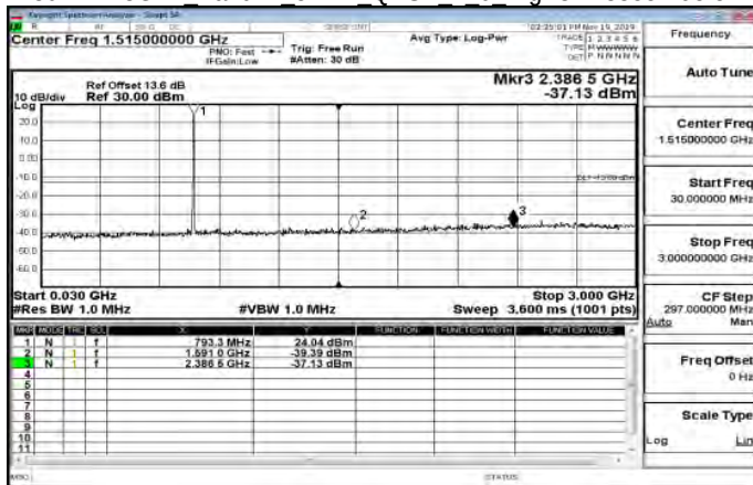
30MHz~3GHz Band14 5MHz QPSK 1 0 HighCH23355-795.5
