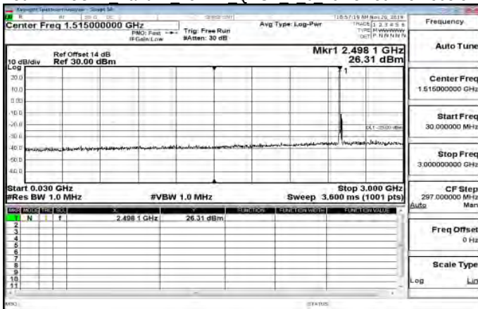
30MHz~3GHz Band41 15MHz QPSK 1 0 LowCH39725-2503.5
