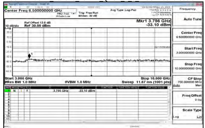
3GHz~10GHz Band26 15MHz QPSK 1 0 MidCH26915-836.5
