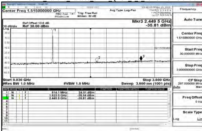
30MHz~3GHz Band26 Part90s 5MHz QPSK 1 0 LowCH26715-816.5
