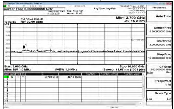
3GHz~10GHz Band26 Part90s 5MHz QPSK 1 0 MidCH26740-819
