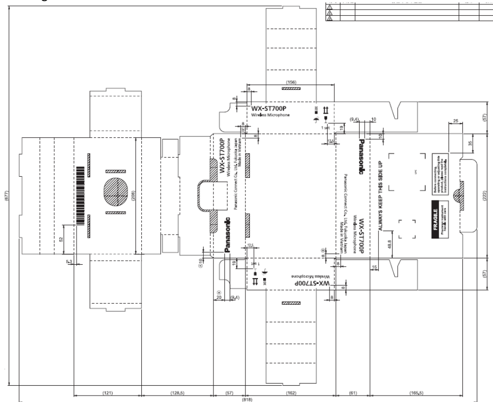
Packing box for WX-ST700P
