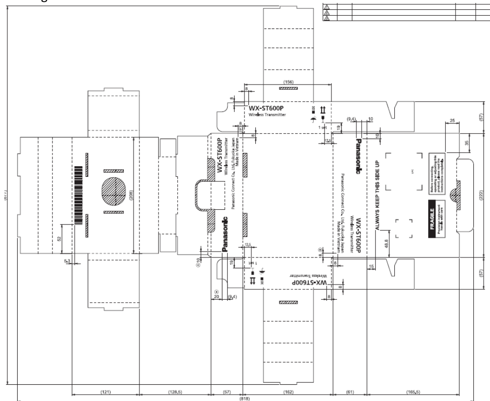
Packing box for WX-ST600P
