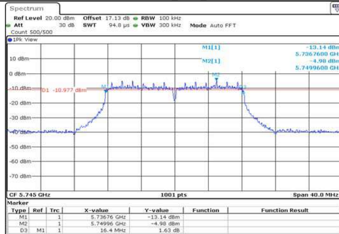
11AMIMO Ant2_5745
