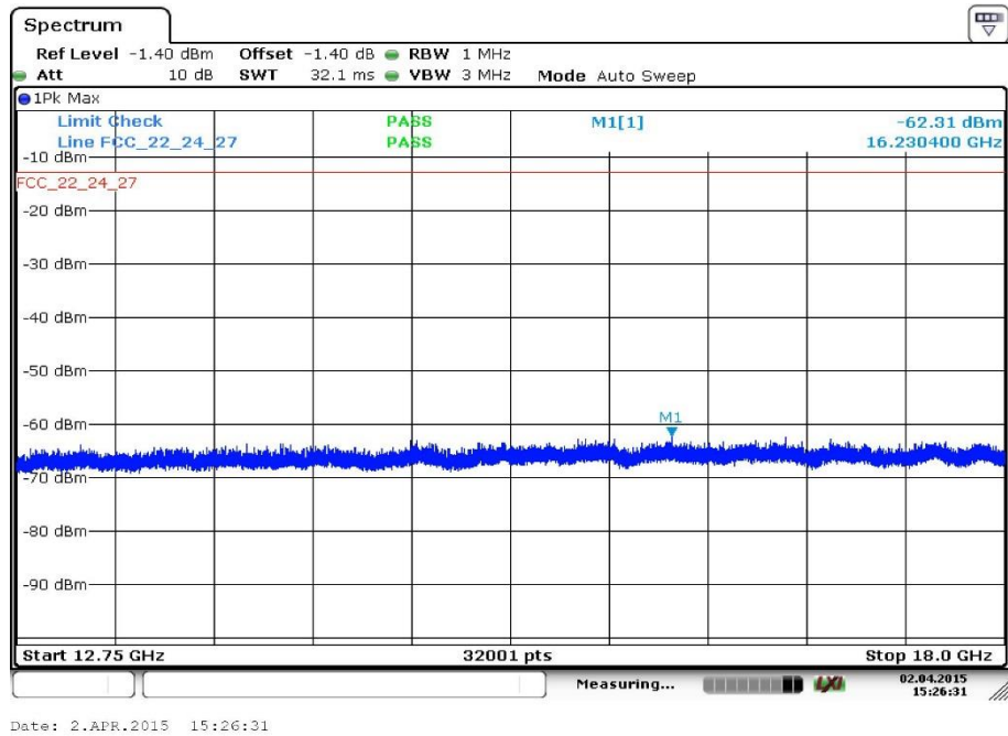
Plot 11: Middle channel, 12.75 GHz to 18 GHz
