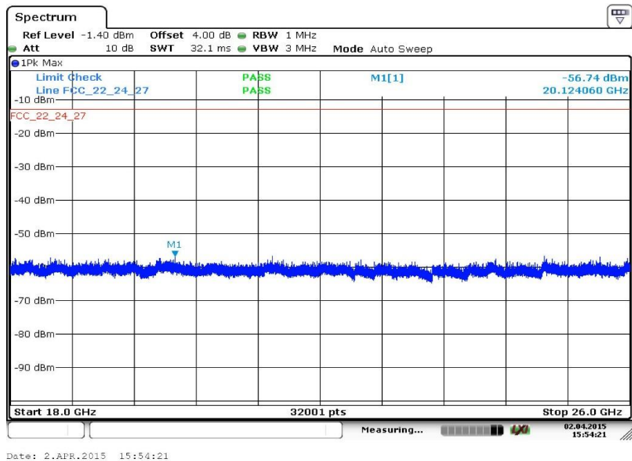
Plot 12: Middle channel, 18 GHz to 26 GHz
