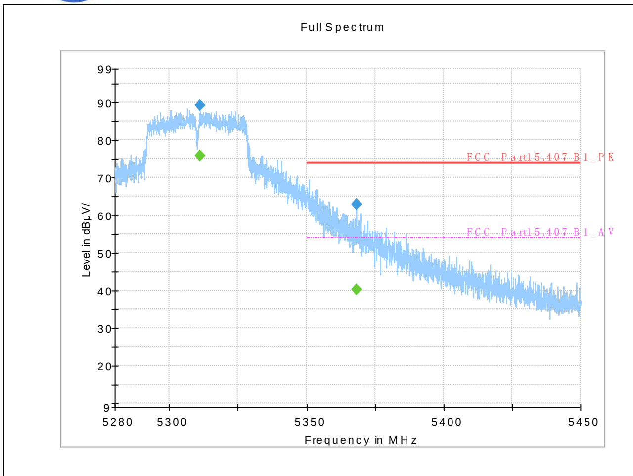
(802.11n (HT40) _5310MHz, Antenna Horizontal)
