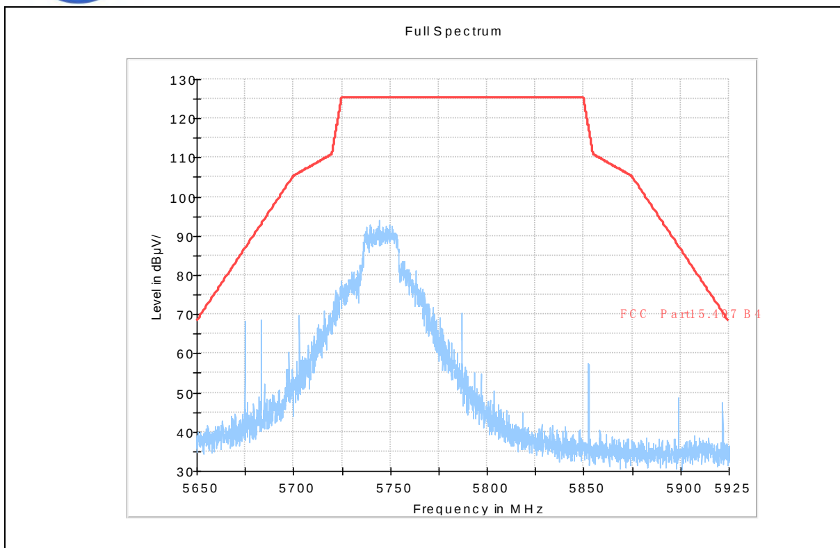
(802.11n(HT20) _5745MHz, Antenna Horizontal)
