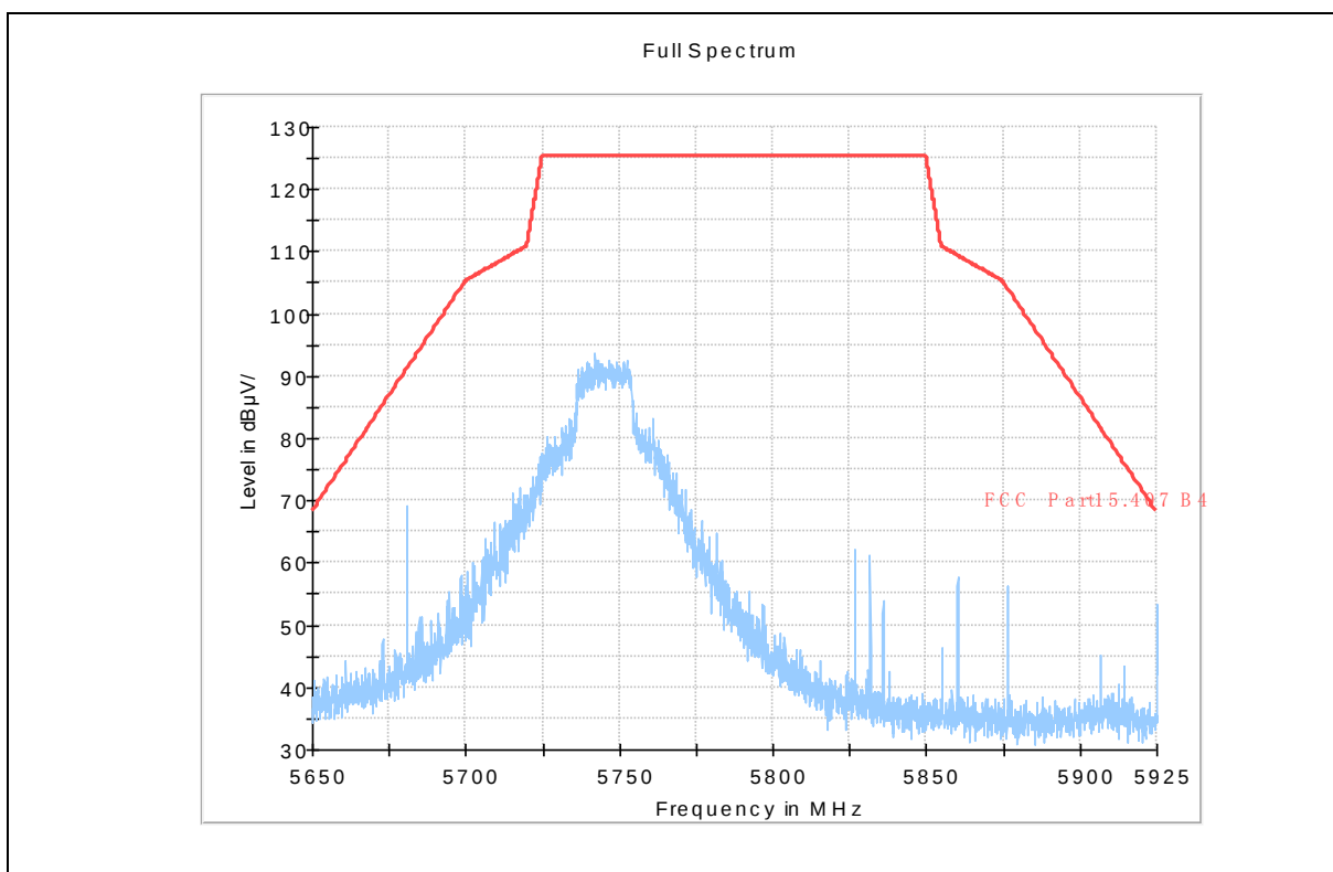
(802.11n(HT20) _5745MHz, Antenna Vertical)
