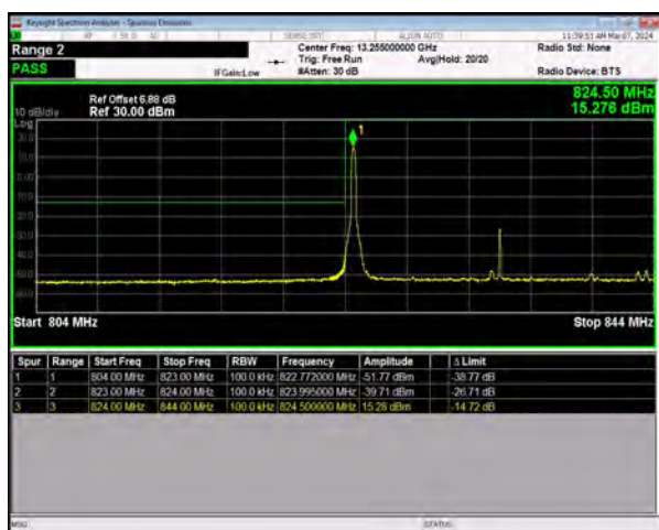
n5 SCS=15kHz DFT_256QAM BW=20MHz LowChannel=166800 RB=1@0
