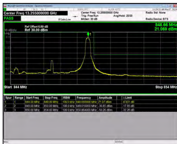
n5 SCS=15kHz DFT_BPSK BW=5MHz HighChannel=169300 RB=1@24
