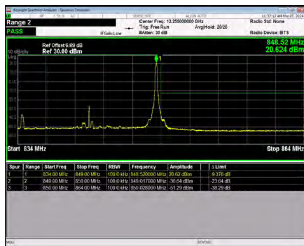
n5 SCS=15kHz DFT_BPSK BW=15MHz HighChannel=168300 RB=1@78
