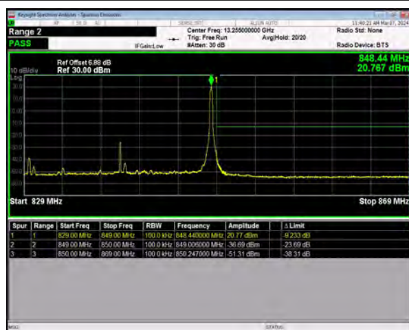
n5 SCS=15kHz DFT_BPSK BW=20MHz HighChannel=167800 RB=1@105
