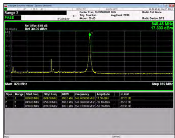
n5 SCS=15kHz DFT_64QAM BW=20MHz HighChannel=167800 RB=1@105
