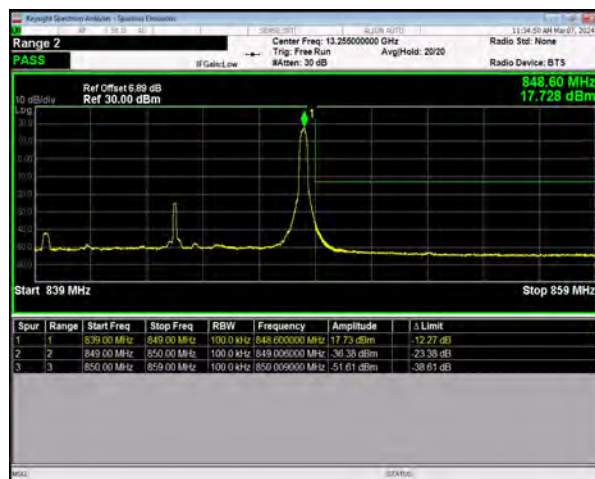
n5 SCS=15kHz DFT_64QAM BW=10MHz HighChannel=168800 RB=1@51
