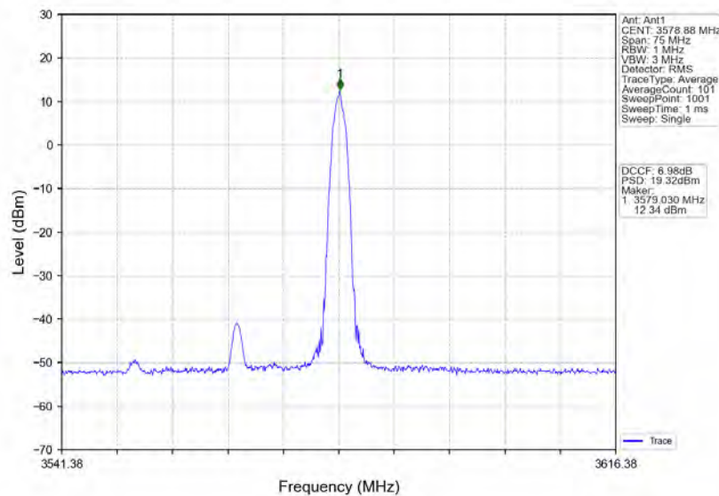
n78d_30kHz_MIMO_NTNV_30MHz_CP-OFDM_16_QAM_3565.02MHz_Edge_1RB_Right
