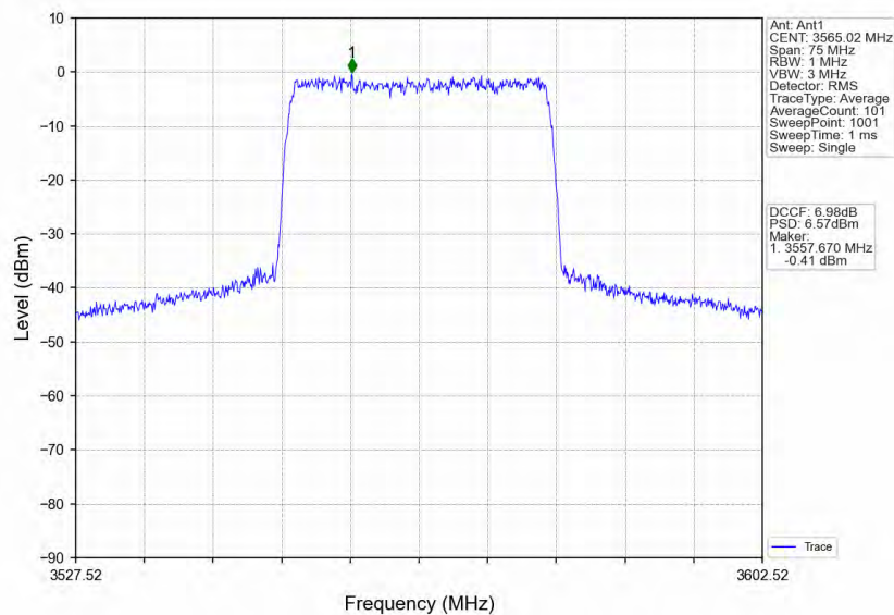
n78d_30kHz_MIMO_NTNV_30MHz_CP-OFDM_16_QAM_3565.02MHz_Inner_Full
