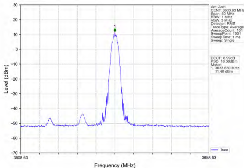
n78d_30kHz_MIMO_NTNV_20MHz_CP-OFDM 64 QAM_3624.99MHz_Inner_1RB_Right
