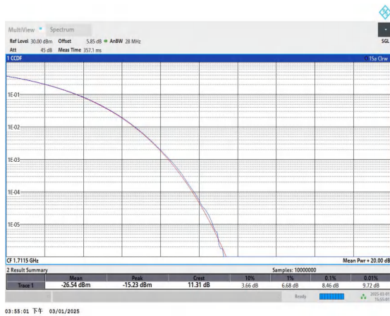
Band4-3MHz-QPSK-19965-1RB#0-PASS
