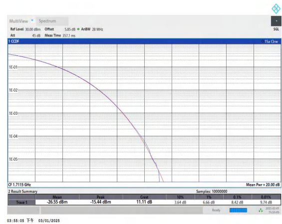
Band4-3MHz-QPSK-19965-15RB#0-PASS
