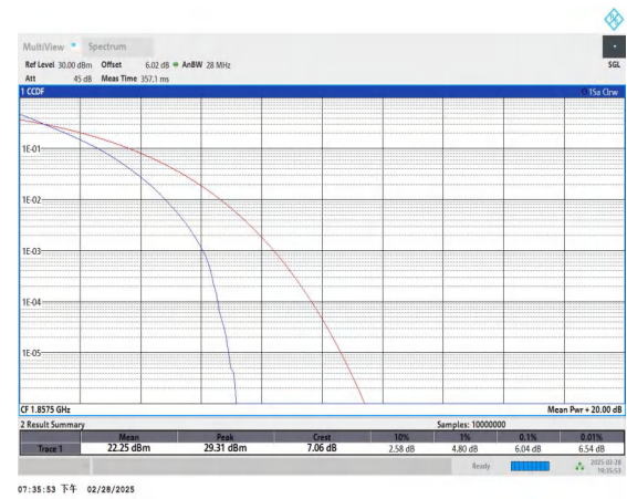
Band2-15MHz-QPSK-18675-75RB#0-PASS
