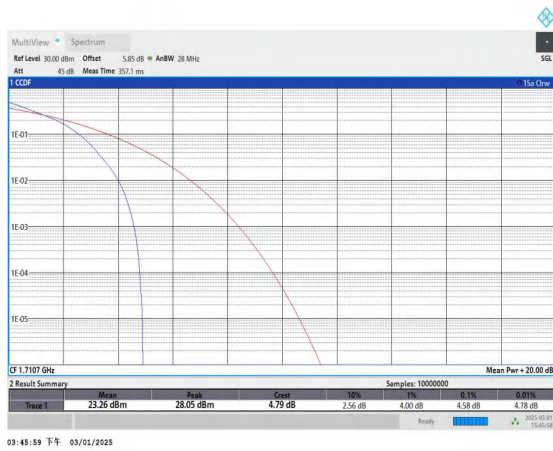
Band4-1.4MHz-QPSK-19957-1RB#0-PASS
