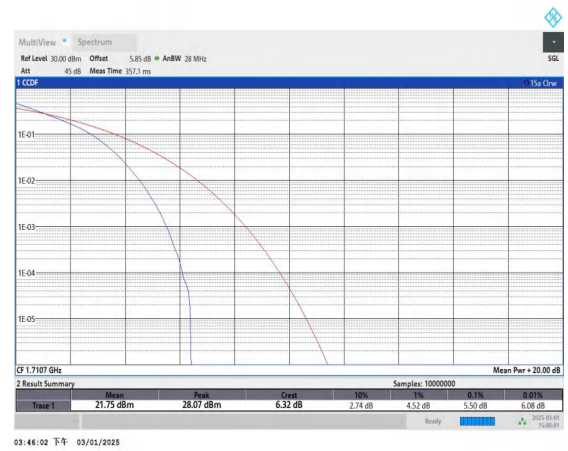
Band4-1.4MHz-QPSK-19957-6RB#0-PASS
