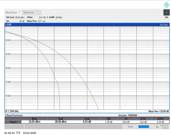
Band4-1.4MHz-QPSK-20393-6RB#0-PASS
