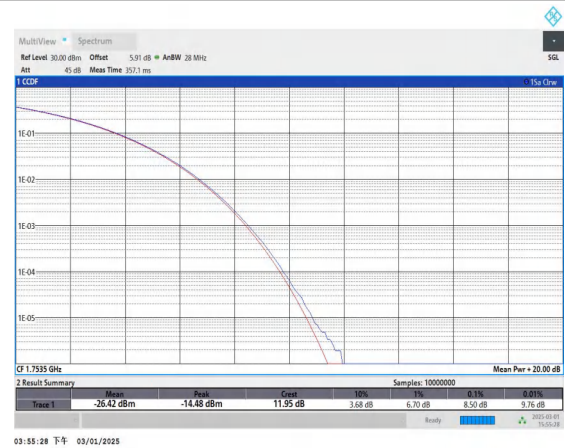
Band4-3MHz-QPSK-20385-15RB#0-PASS
