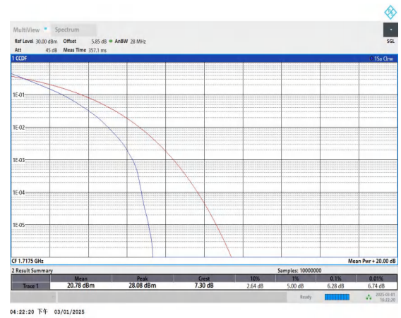
Band4-15MHz-QPSK-20025-75RB#0-PASS
