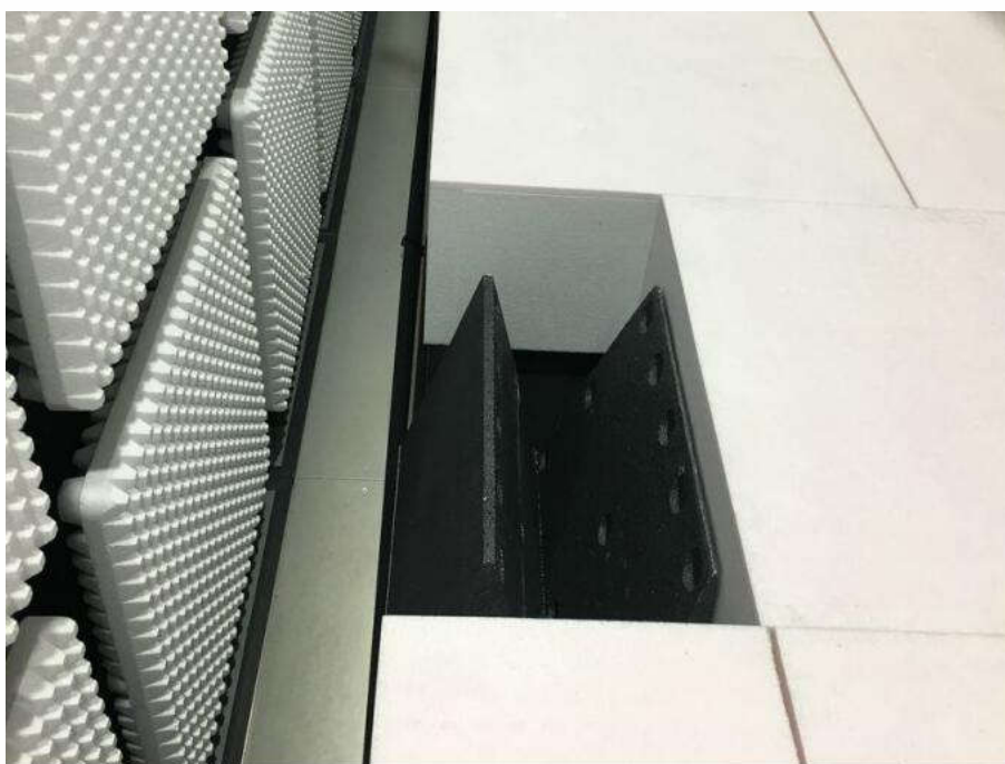
Radiated emission Test Setup-4 (above 1GHz) There are absorbing materials under the ground.
