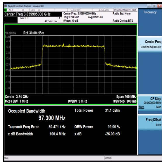
NTNV-N77-3700-3980-PC2-30-100-M-CP- 16QAM-Outer Full-Ant7-PASS
