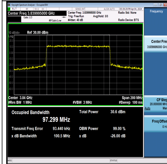
NTNV-N77-3700-3980-PC2-30-100-M-CP- 64QAM-Outer Full-Ant7-PASS
