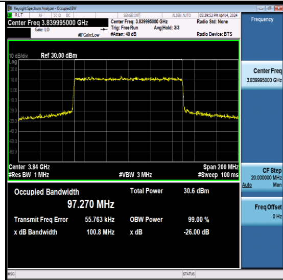
NTNV-N77-3700-3980-PC2-30-100-M-CP- 256QAM-Outer Full-Ant7-PASS
