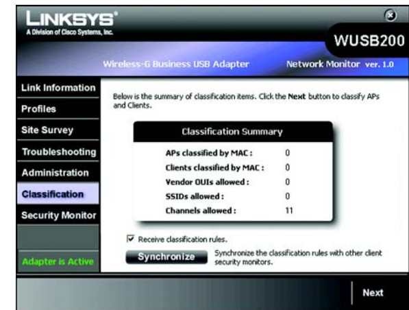
Figure 6-4: AP Classification
