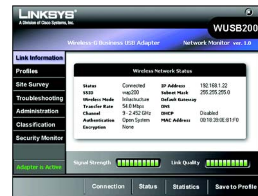
Figure 6-3: Classification
