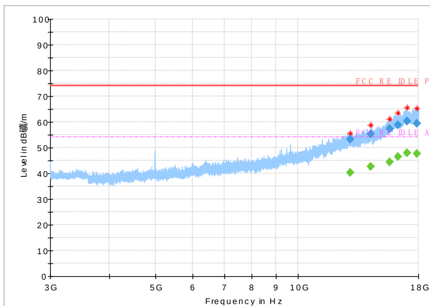
Fig 61. Radiated Spurious Emission (802.11b, Ch1, 3GHz~18GHz)
