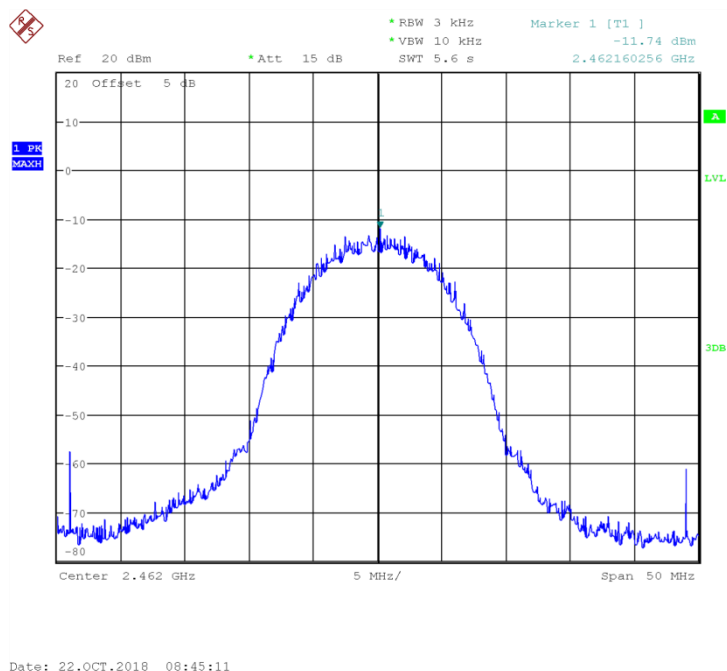
Fig 3. Power Spectral Density (802.11b, Ch11)
