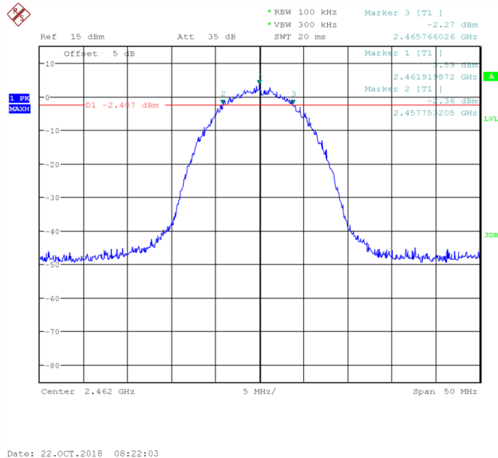
Fig 15. Occupied 6dB Bandwidth (802.11b, Ch11)
