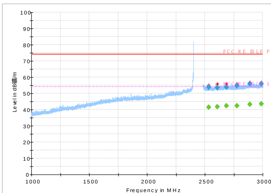
Fig 70. Radiated Spurious Emission (802.11 n-20MHz, Ch1,1GHz~3GHz)
