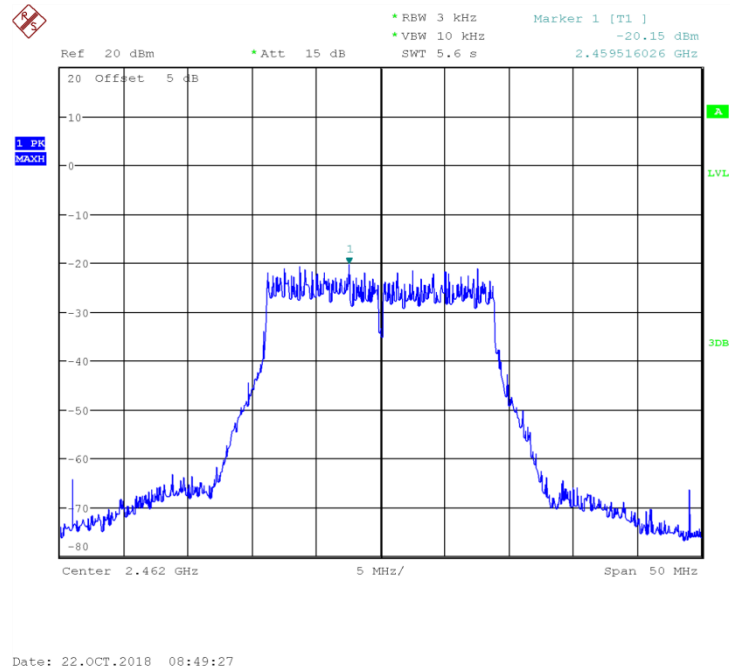
Fig 9. Power Spectral Density (802.11n-20MHz, Ch11)
