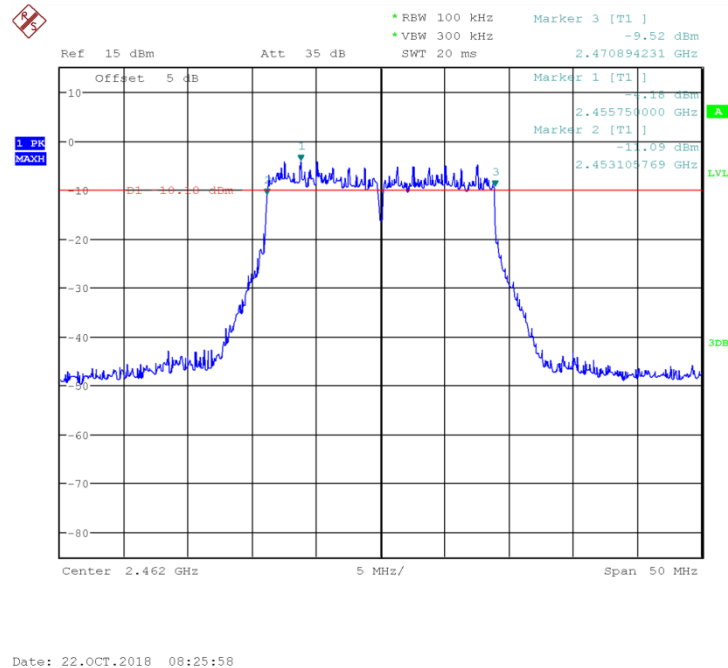
Fig 21. Occupied 6dB Bandwidth (802.11n-20MHz, Ch11)
