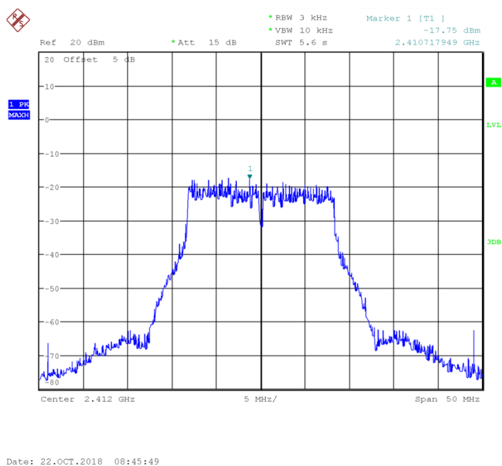
Fig 4. Power Spectral Density (802.11g, Ch1)
