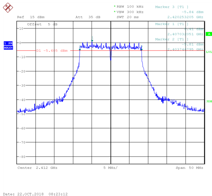
Fig 16. Occupied 6dB Bandwidth (802.11g, Ch1)
