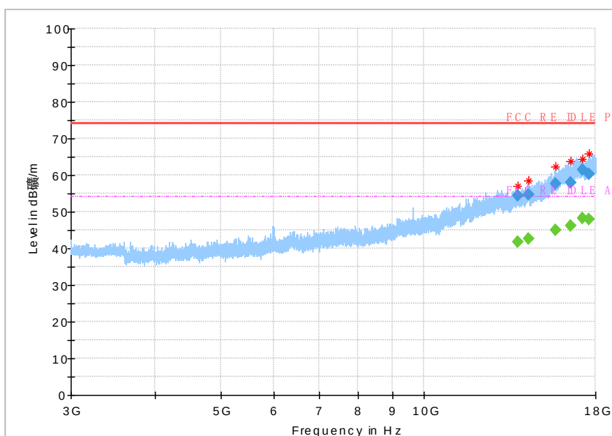
Fig 71. Radiated Spurious Emission (802.11 n-20MHz, Ch1,3GHz~18GHz)
