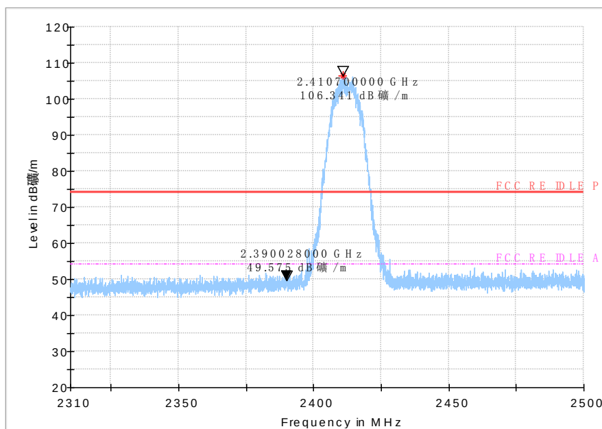
Peak detector
