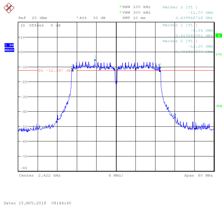
Fig 22. Occupied 6dB Bandwidth (802.11n-40MHz, Ch3)
