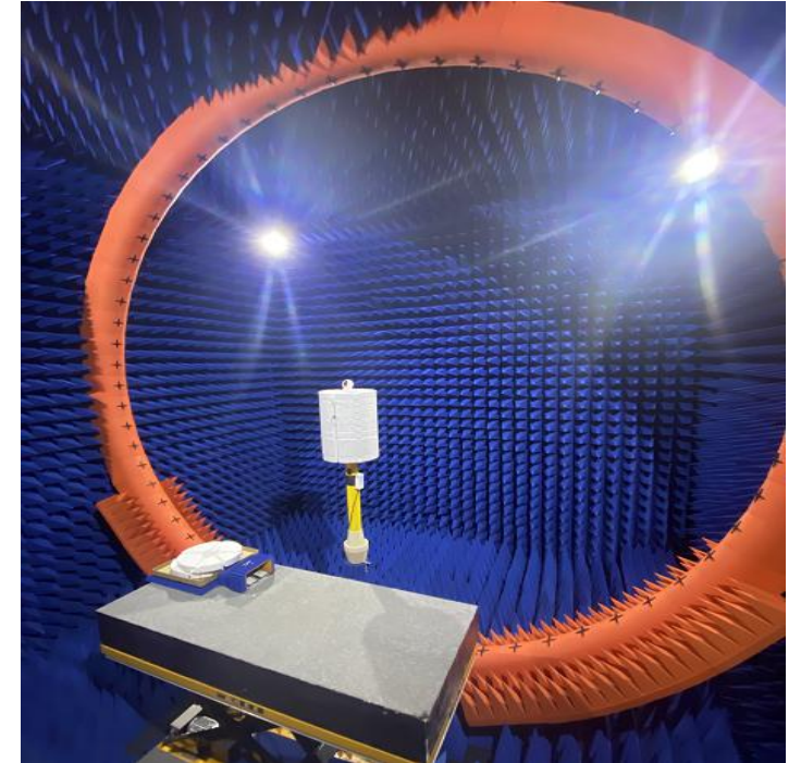
Testing 3D microwave darkroom(6m*6m*6m)
