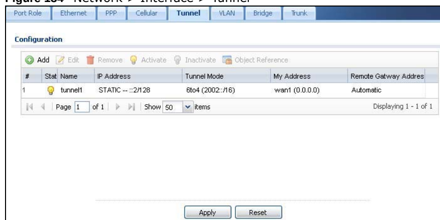
Figure 134 Network &gt; Interface &gt; Tunnel
