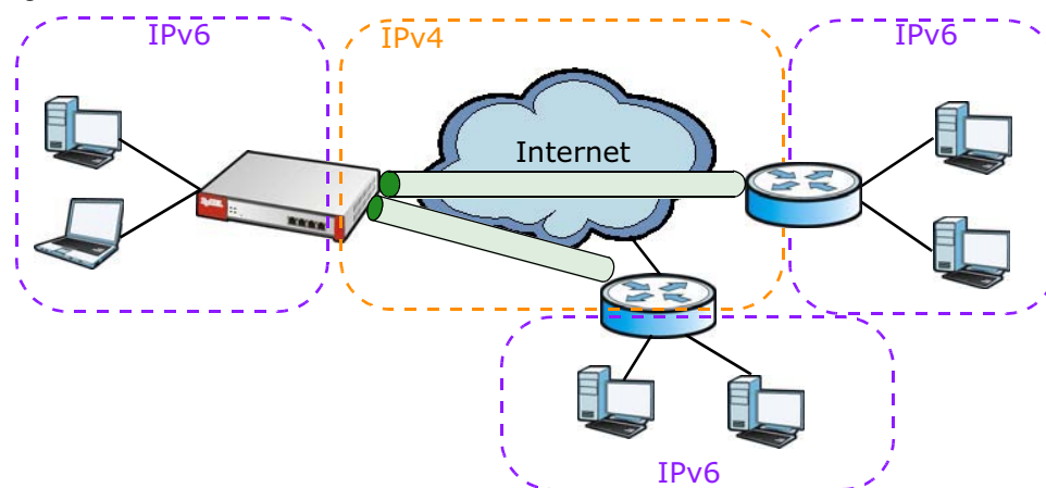
Figure 133 6to4 Tunnel
