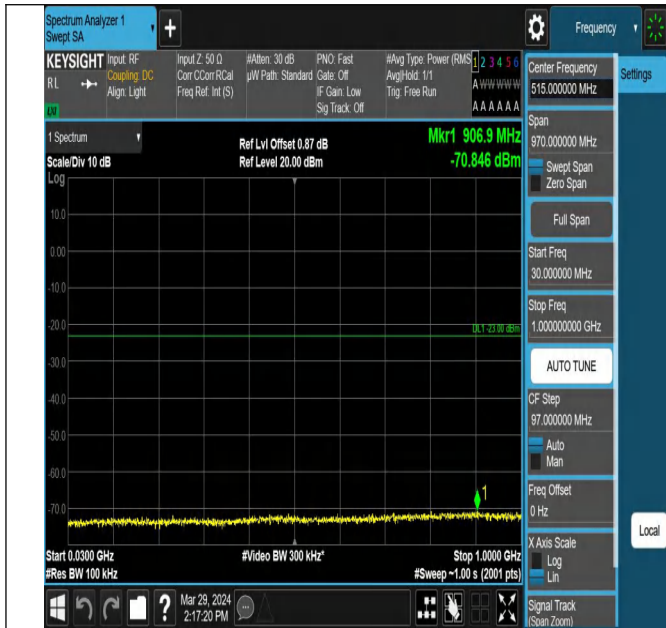
Band25_10MHz_QPSK_26365_1RB#0_30~1000_30~1000
