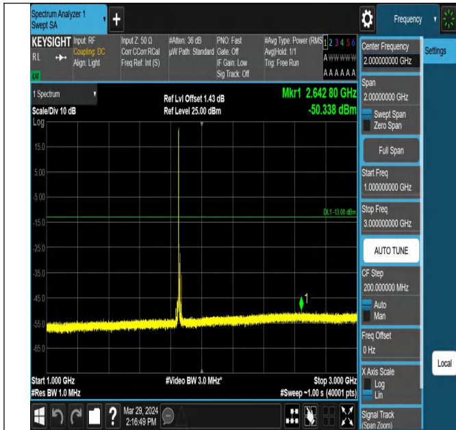
Band25_10MHz_QPSK_26090_1RB#0_1000~3000_1000~30
