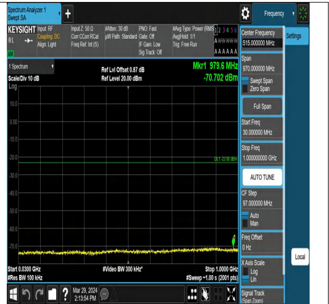
Band25_5MHz_QPSK_26365_1RB#0_30~1000_30~1000
