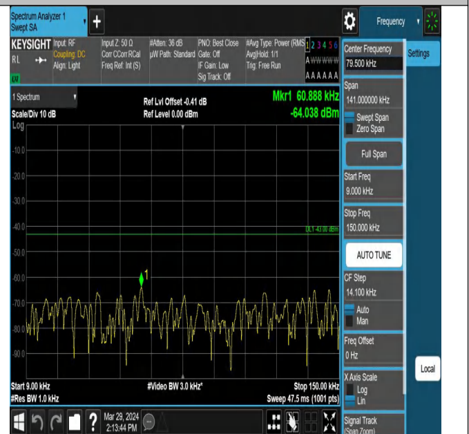
Band25_5MHz_QPSK_26365_1RB#0_0.009~0.15_0.009~0.1
