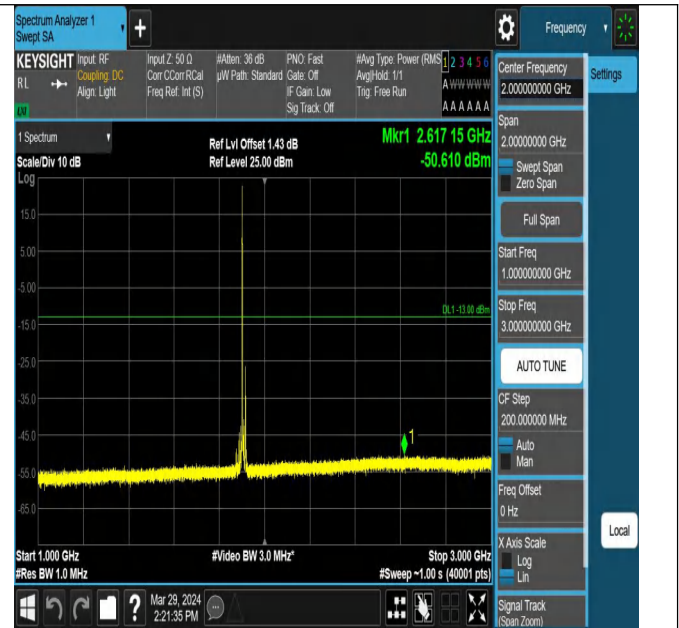
Band25_15MHz_QPSK_26615_1RB#0_1000~3000_1000~3000
