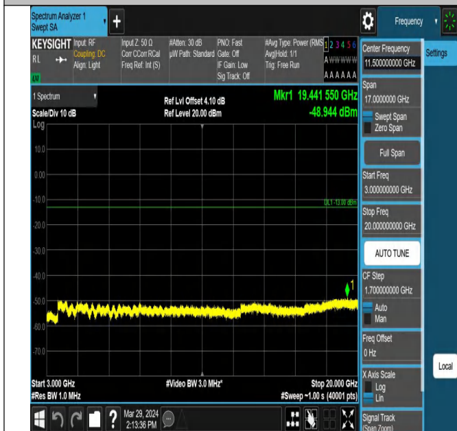
Band25_5MHz_QPSK_26065_1RB#0_3000~20000_3000~20
