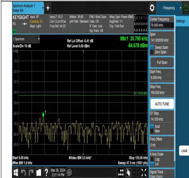
Band25_15MHz_QPSK_26615_1RB#0_0.009~0.15_0.009~0.
