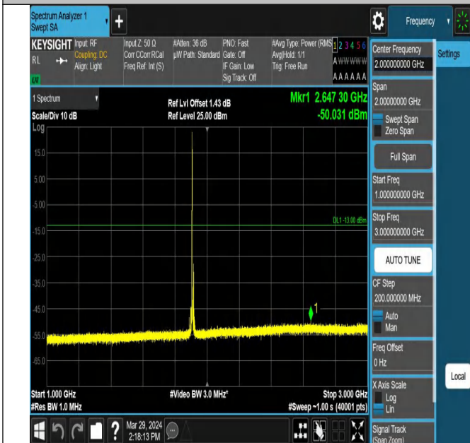
Band25_10MHz_QPSK_26640_1RB#0_1000~3000_1000~30
