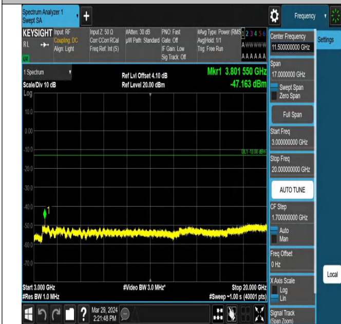
Band25_15MHz_QPSK_26615_1RB#0_3000~20000_3000~20000
