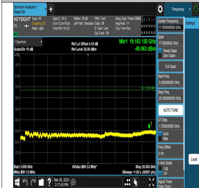
Band25_10MHz_QPSK_26365_1RB#0_3000~20000_3000~20000
