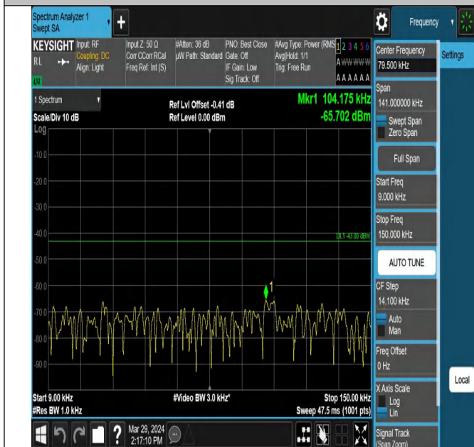
Band25_10MHz_QPSK_26365_1RB#0_0.009~0.15_0.009~0.
