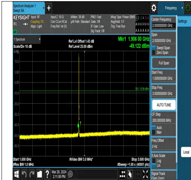
Band25_3MHz_QPSK_26675_1RB#0_1000~3000_1000~300
