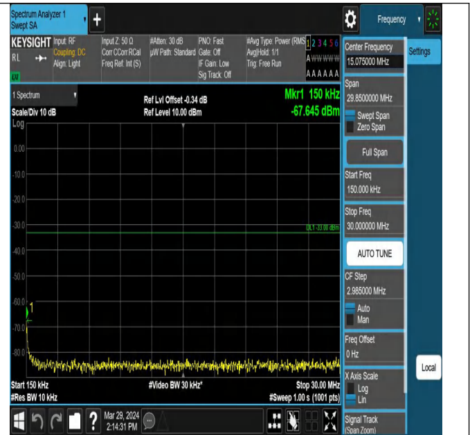
Band25_5MHz_QPSK_26665_1RB#0_0.15~30_0.15~30
