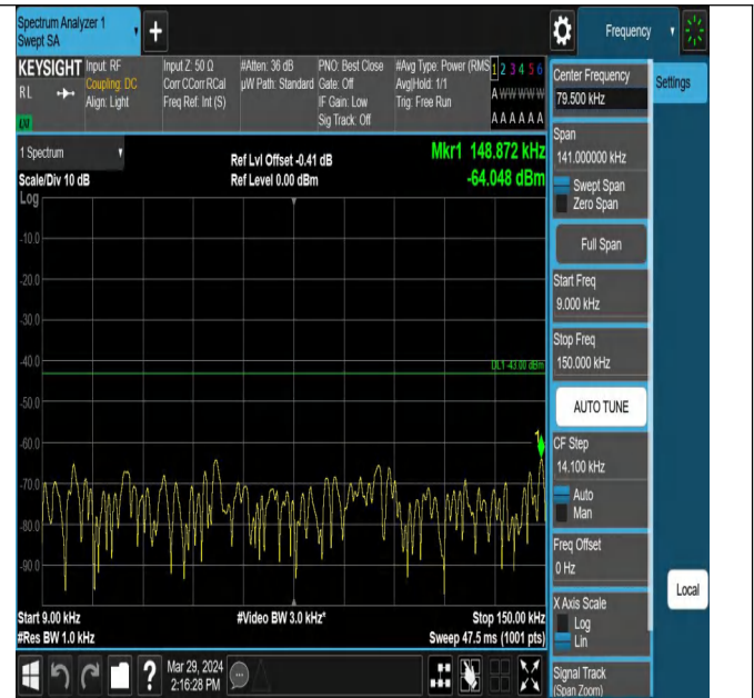
Band25_10MHz_QPSK_26090_1RB#0_0.009~0.15_0.009~0.15
