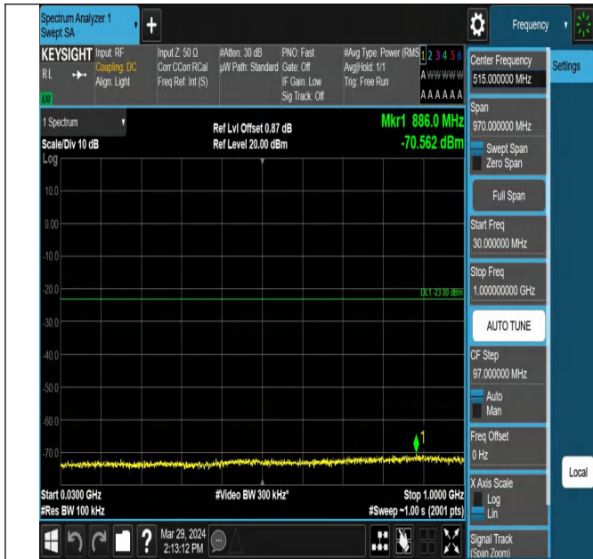
Band25_5MHz_QPSK_26065_1RB#0_30~1000_30~1000
