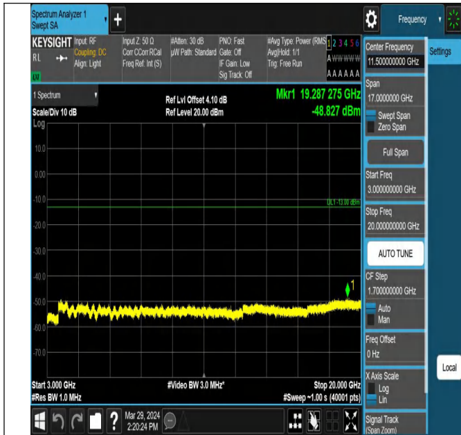
Band25_15MHz_QPSK_26115_1RB#0_3000~20000_3000~20000
