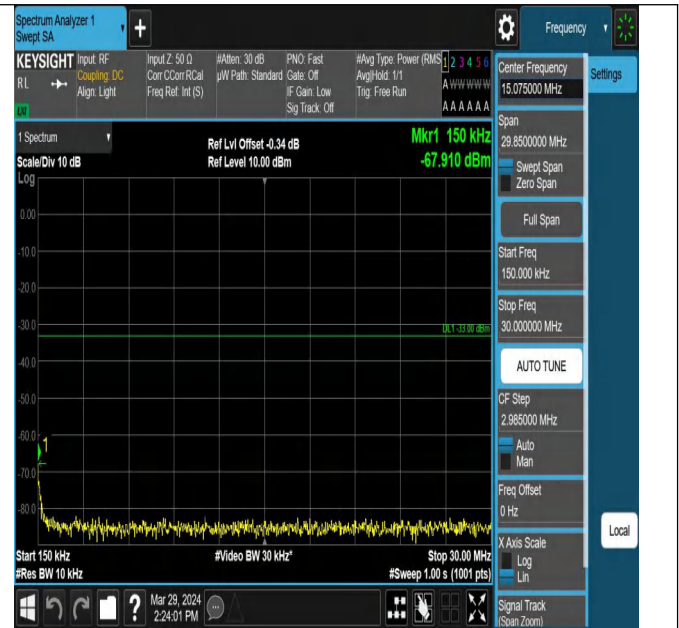
Band25_20MHz_QPSK_26365_1RB#0_0.15~30_0.15~30
