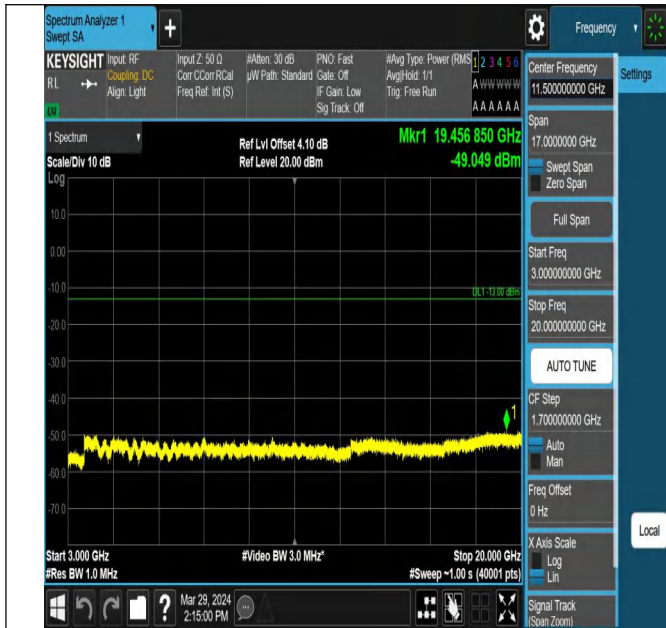
Band25_5MHz_QPSK_26665_1RB#0_3000~20000_3000~20000
