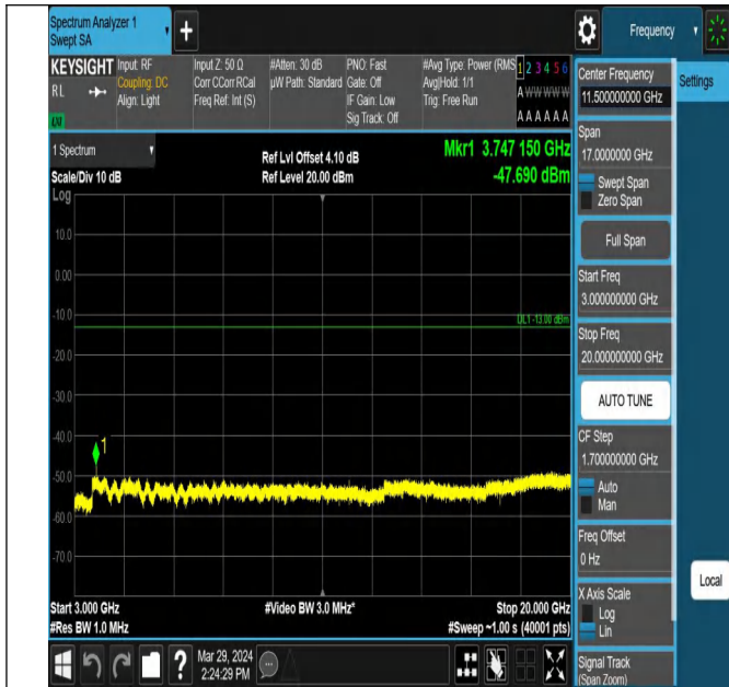
Band25_20MHz_QPSK_26365_1RB#0_3000~20000_3000~20000 0000
