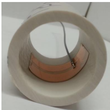
Figure 17: Concave-mounted
