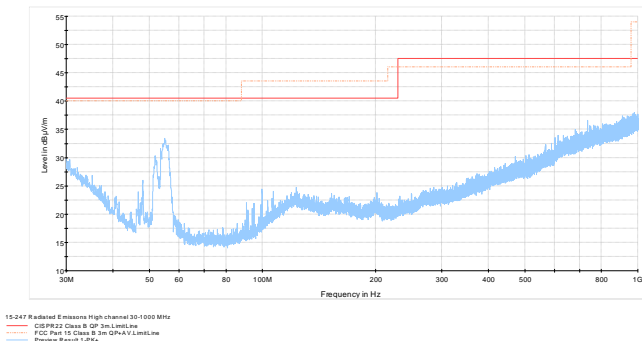
Plot 8.5-14: Radiated spurious emissions on high channel
