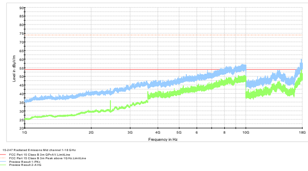
Plot 8.5-13: Radiated spurious emissions on mid channel
