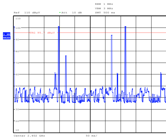
Plot 8.2-4: Number of hopping channels = 79
