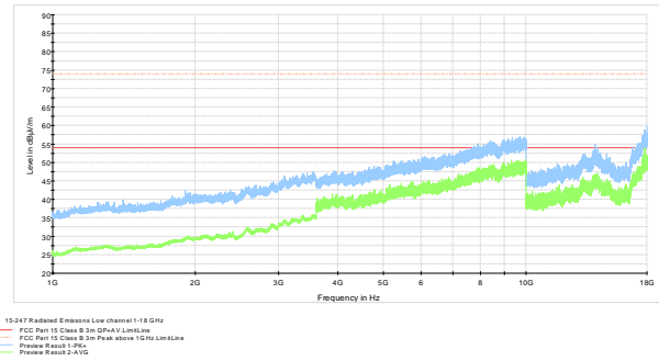
Plot 8.5-11: Radiated spurious emissions on low channel
