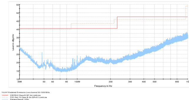
Plot 8.5-10: Radiated spurious emissions on low channel
