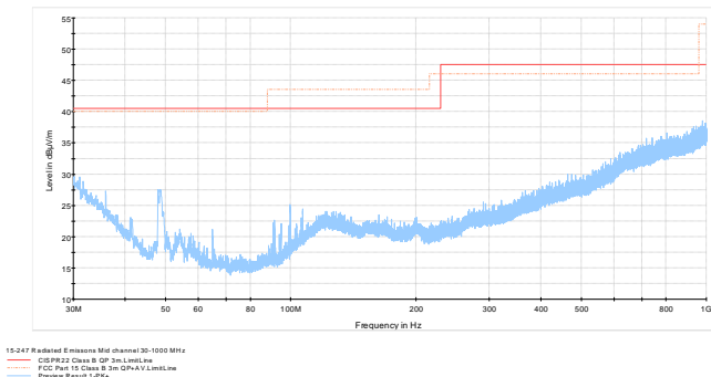
Plot 8.5-12: Radiated spurious emissions on mid channel
