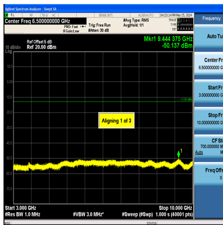
Band26_10MHz_QPSK_26915_1RB#0_3000~10000_3000~10000
