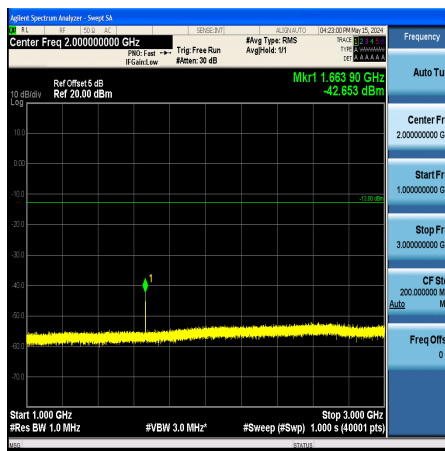
Band26_10MHz_QPSK_26915_1RB#0_1000~3000_1000~3000
