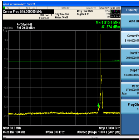
Band26_10MHz_QPSK_26915_1RB#0_30~1000_30~1000
