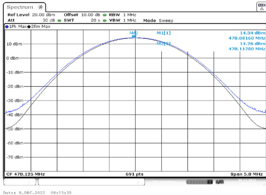
Plot 1: 470.125 MHz (modulated carrier)
