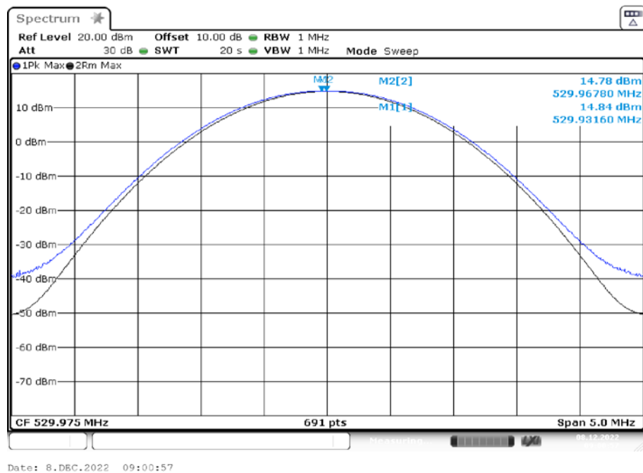
Plot 3: 529.975 MHz (modulated carrier)
