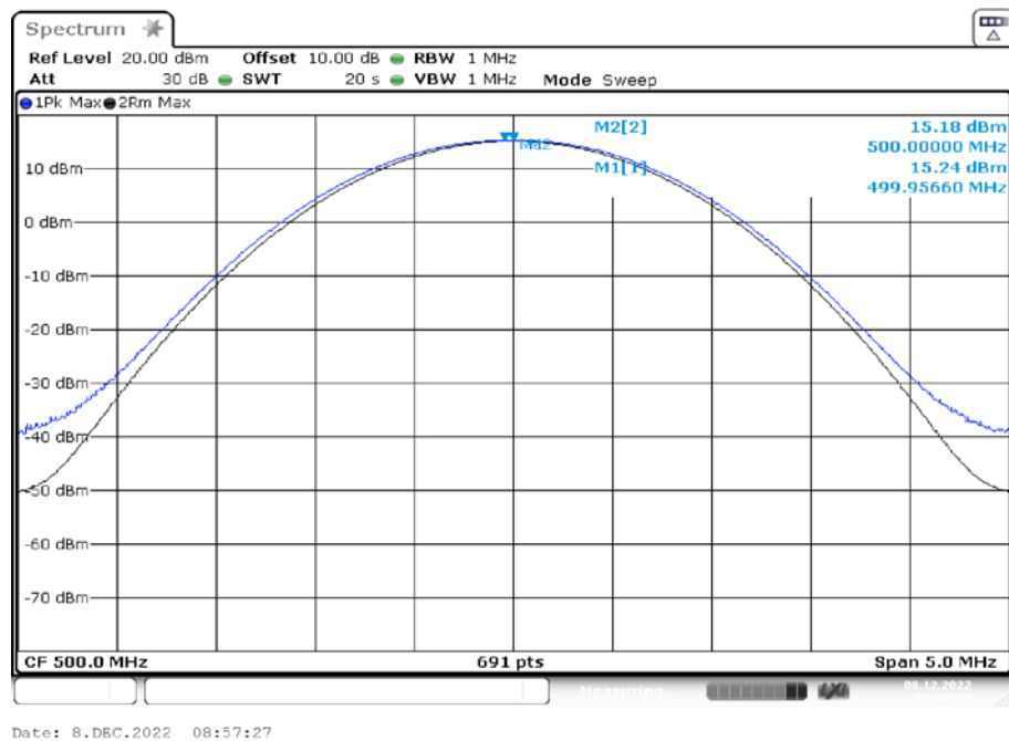
Plot 2: 500.000 MHz (modulated carrier)
