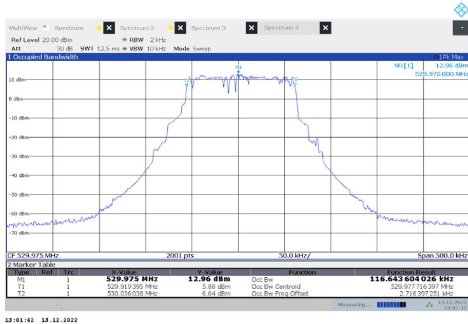
Plot 3: 529.975 MHz, max hold with frequency variation from 50 Hz to 15 kHz
