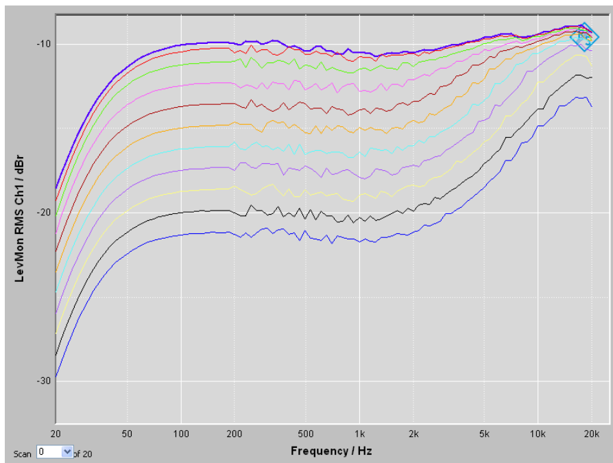
Plot 1: 11 curves with voltage and frequency variation
