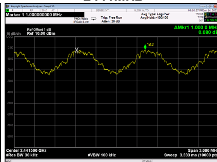
2441MHz
